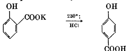
Potassium salicylate
