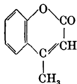
4-Methylcoumarin
