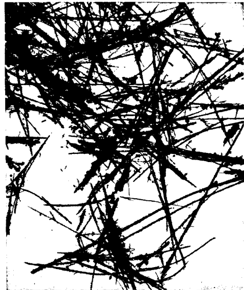
XYLOSAZONE
