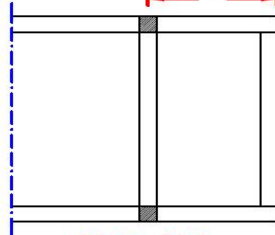
Struc. Plan
