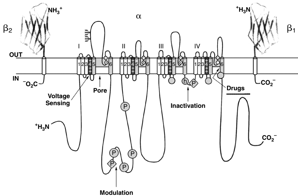
FIGURE 16-4 Functional structure of the \text{Na}^+ channel (linear representation). The four primary domains of the \alpha subunit are indicated by Roman numerals, with the six helical segments (designated S1 through S6, left to right) of each domain shown spanning the membrane. A portion of each of the S5-S6 linkages lines the outer portion of the pore and confers ion selectivity to the channel. The inner portion is lined by the S6 and (to a lesser extent) S5 helices. Outward rotation of the positively charged S4 cylinders and coupled movements of the S6 segments open the pore. Concurrently, portions of the S4-S5 linkages of domains III and IV, which help form the inner mouth of the channel, and the S6 segment of domain IV create a receptor (unlettered circles) for a hydrophobic triad of amino acid residues (isoleucine-phenylalanine-methionine; IFM motif) in the intracellular loop between domains III and IV, which constitutes the inactivation, or h , gate ( h ). Binding of the h gate to its receptor inactivates the channel within about 1 ms. Each P indicates a phosphorylation site for protein kinase A (circles) and protein kinase C (diamonds). Phosphorylation of the h gate slows inactivation; phosphorylation of other sites reduces channel activation. The \psi symbols indicate glycosylation sites. The \beta subunits ( \beta_1 and \beta_2 ) modulate \text{Na}^+ channel electrophysiology and serve as cell adhesion molecules, stabilizing the \alpha subunit in the nerve membrane by interacting with other \beta subunits and with contactin and ankyrin proteins. (Adapted from Catterall WA: From ionic currents to molecular mechanisms: the structure and function of voltage-gated sodium channels, Neuron 26:13-25, 2000.)
