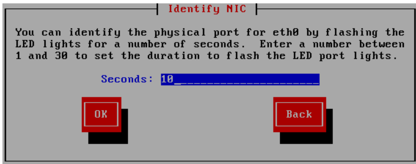
Figure 8.7. Identify NIC
