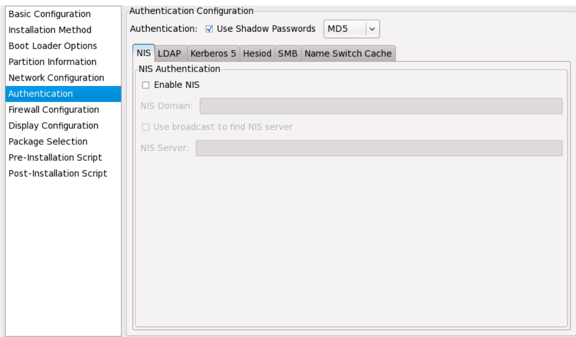
Figure 33.9. Authentication
