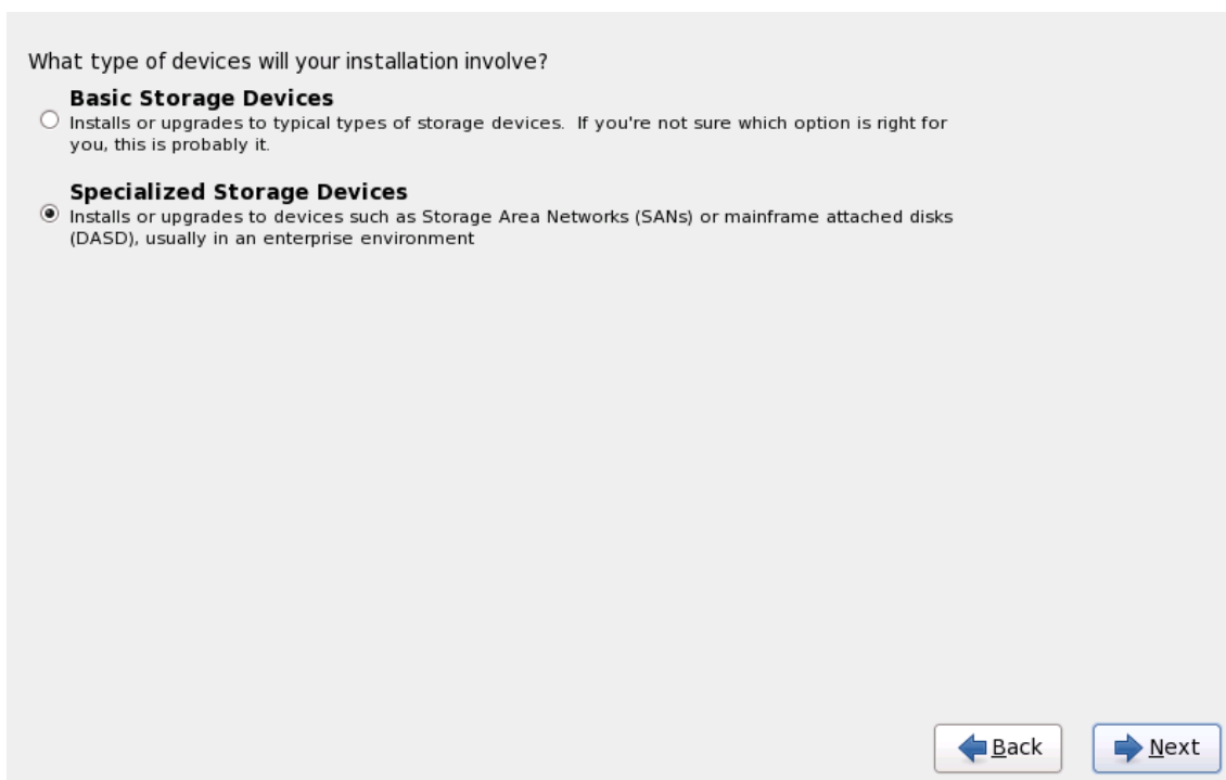
Figure 23.4. Storage devices
