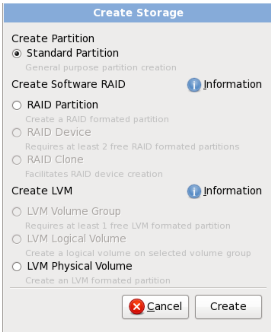
Figure 16.40. Creating Storage
