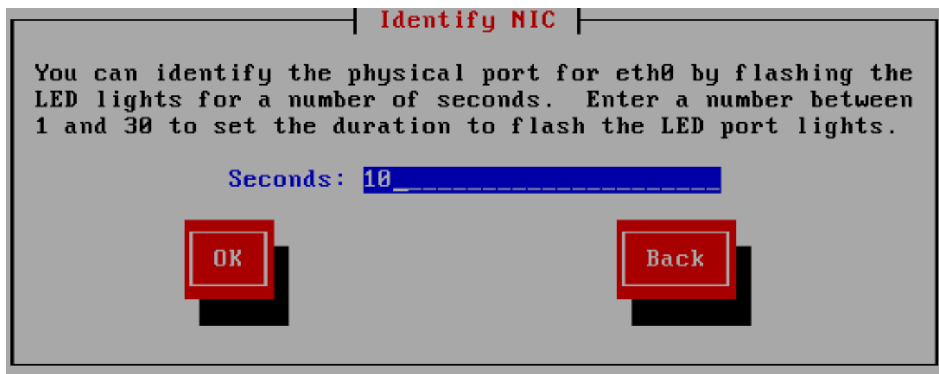
Figure 15.7. Identify NIC
