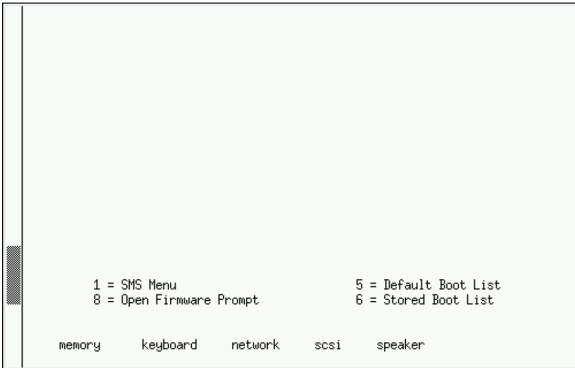
Figure 14.1. SMS console
