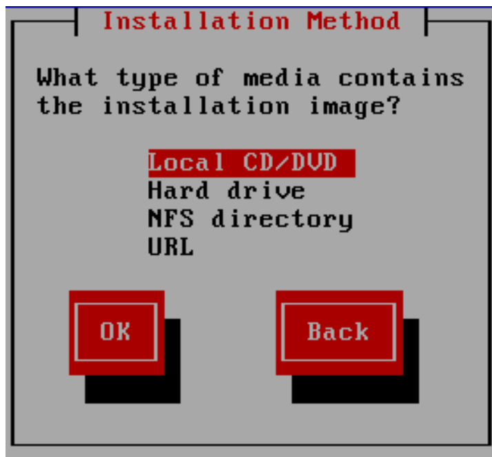
Figure 8.4. Installation Method
