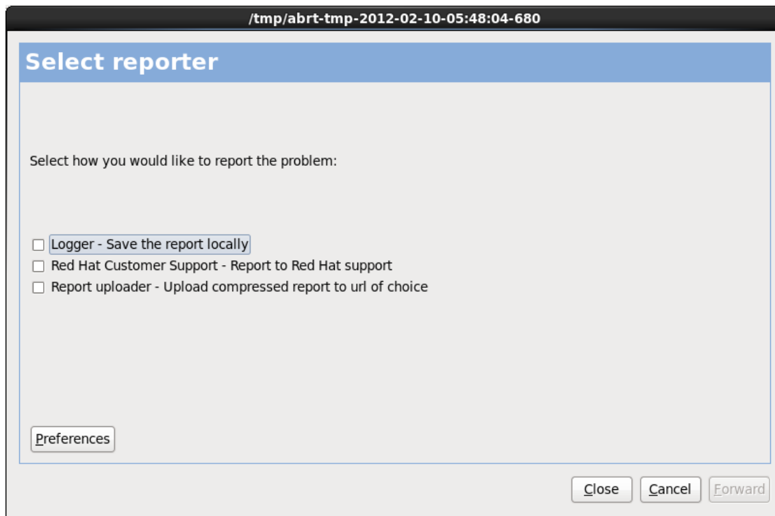
Figure 10.3. Select reporter
