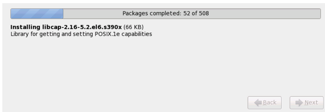
Figure 16.55. Packages completed
