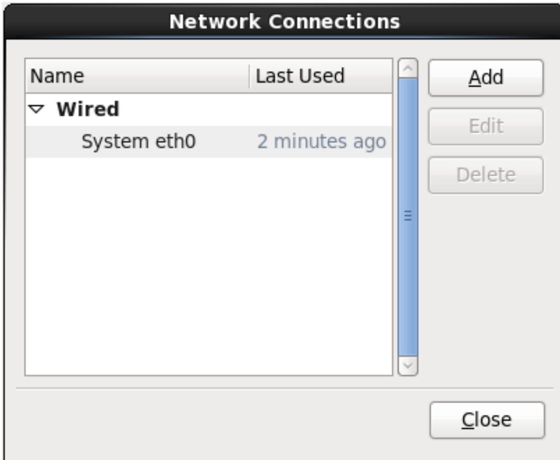
Figure 9.52. Network Connections
