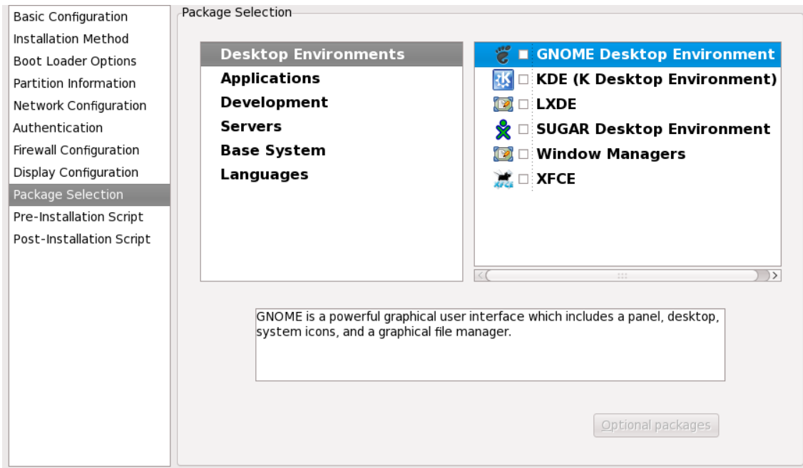
Figure 33.12. Package Selection
