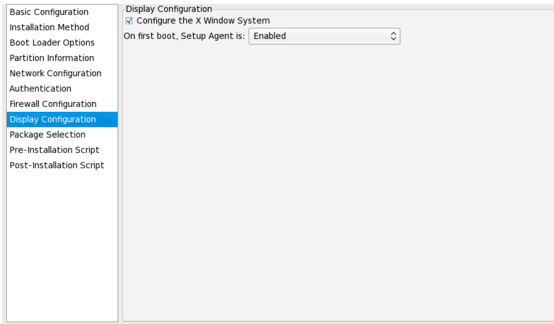
Figure 33.11. X Configuration
