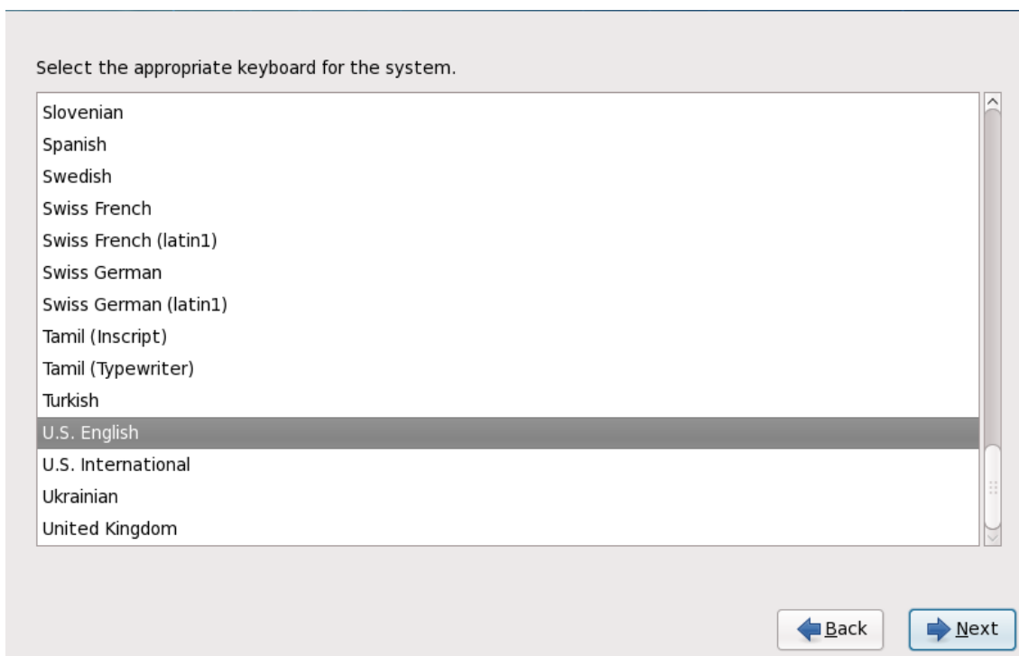
Figure 9.3. Keyboard Configuration
