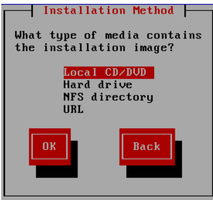
Figure 22.4. Installation Method
