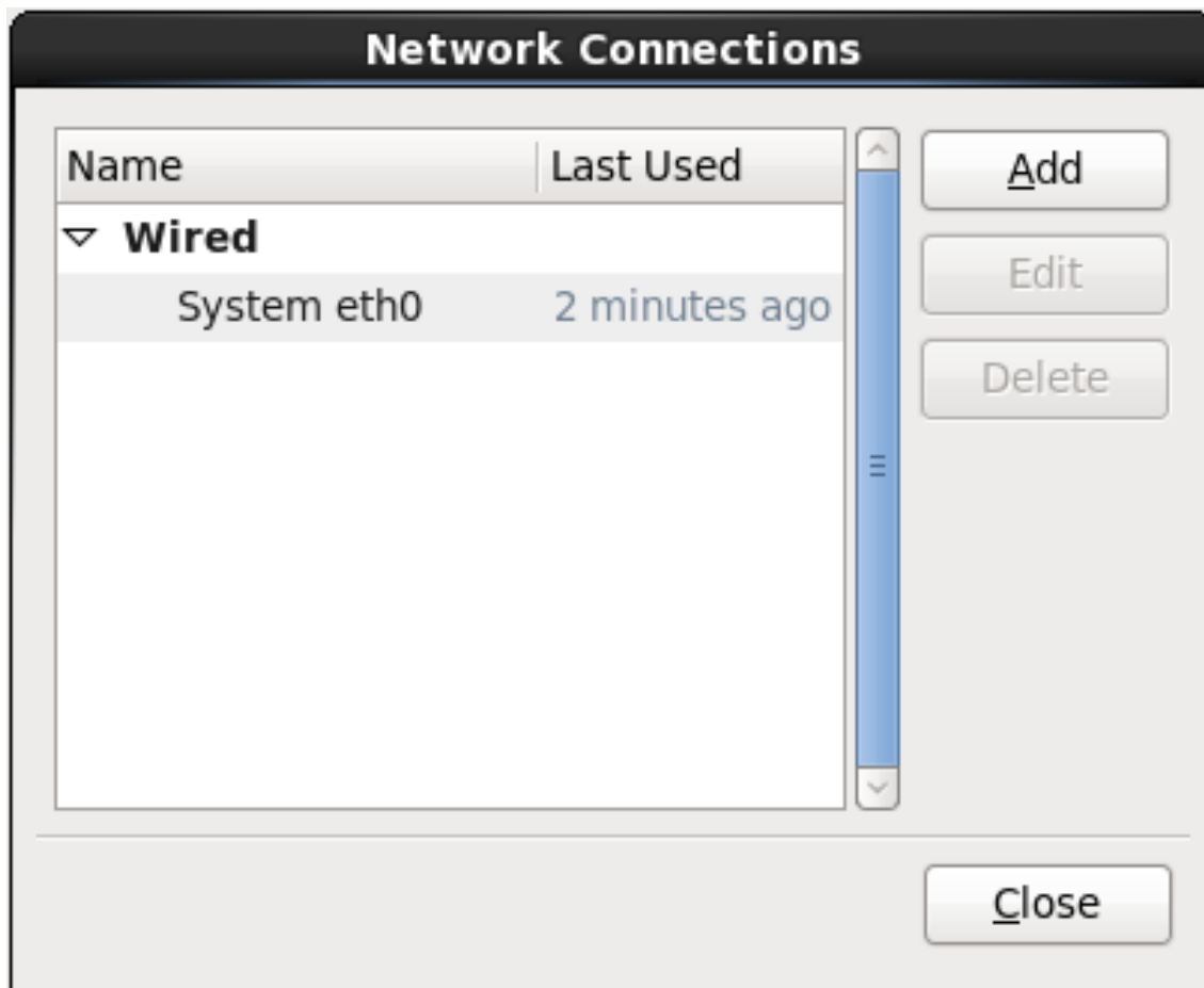
Figure 23.24. Network Connections
