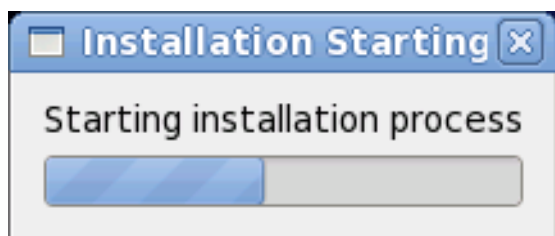
Figure 16.54. Starting installation
