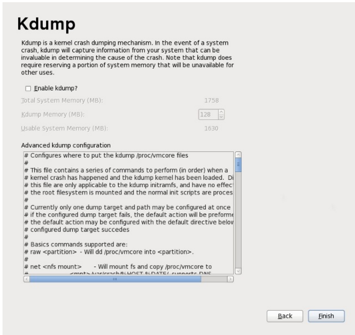
Figure 34.16. Kdump screen
