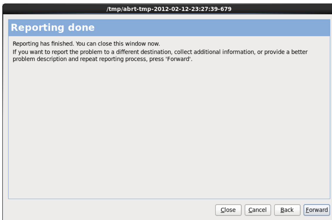
Figure 17.11. Reporting done
