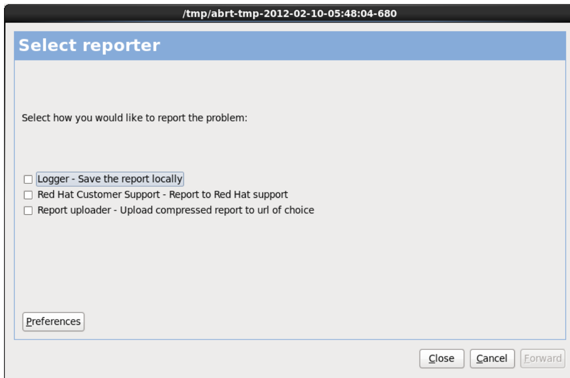
Figure 17.3. Select reporter
