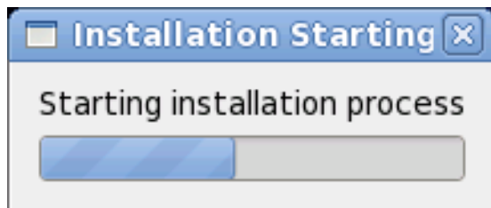
Figure 23.53. Starting installation
