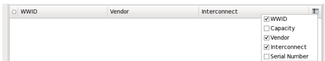
Figure 9.9. Selecting Columns
