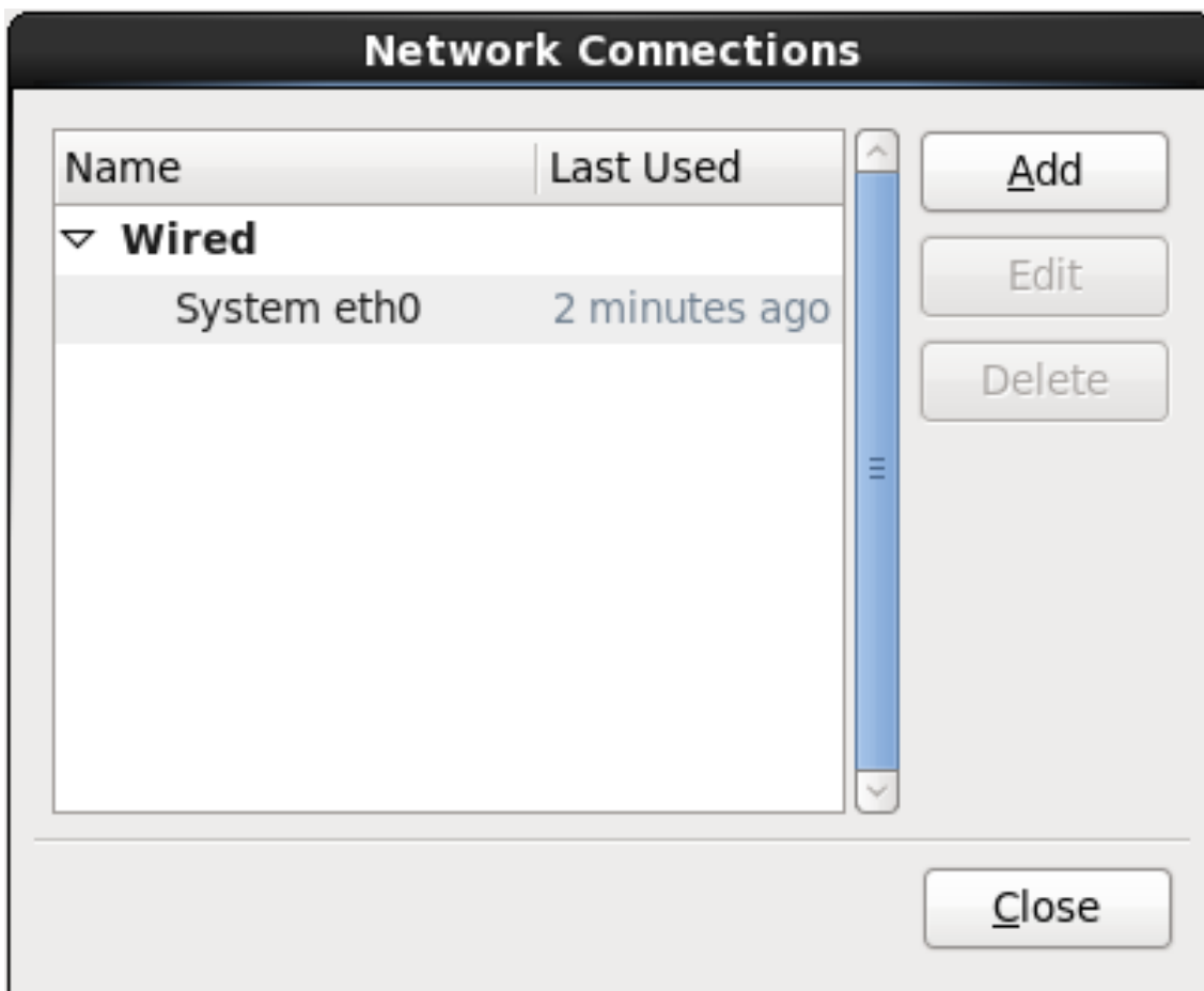
Figure 16.25. Network Connections
