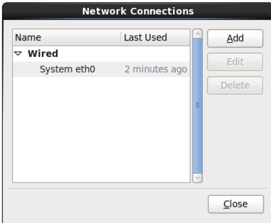
Figure 16.12. Network Connections
