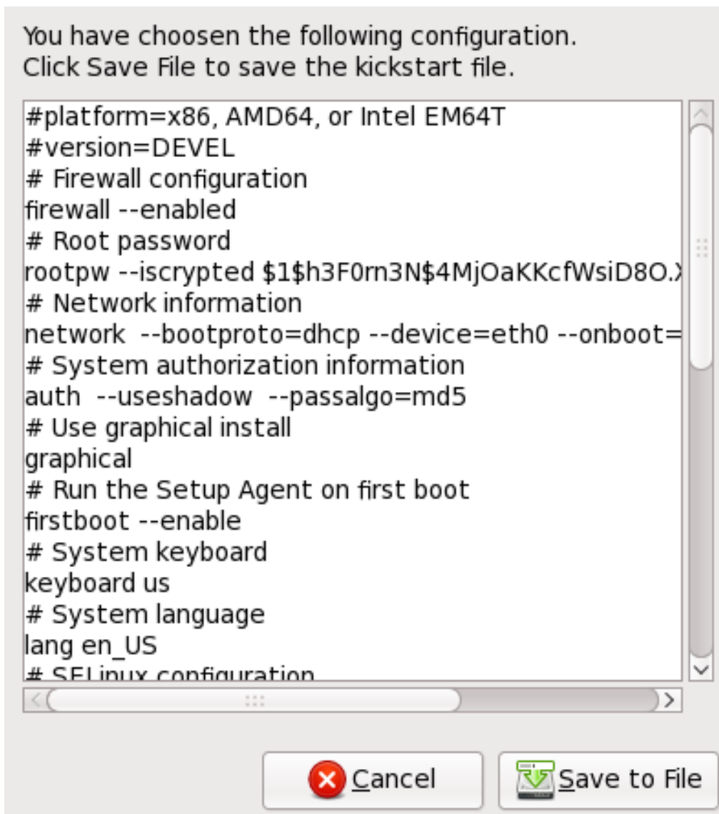
Figure 33.15. Preview
