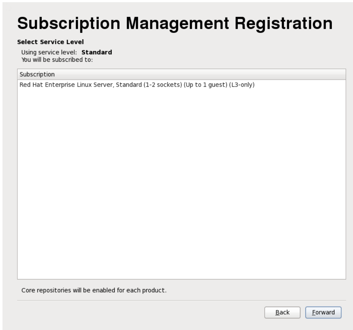
Figure 34.10. Confirm Subscription
