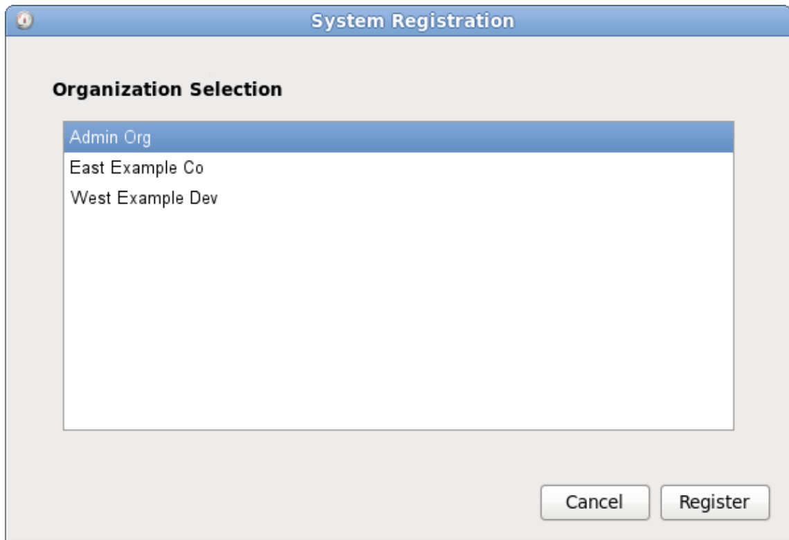
Figure 34.8. Organization Selection
