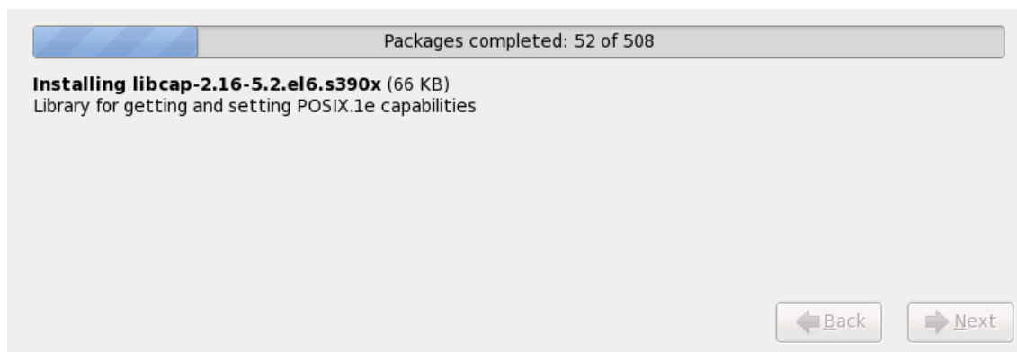
Figure 23.54. Packages completed
