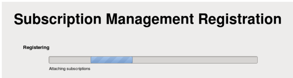
Figure 34.9. Auto-Selecting Subscriptions
