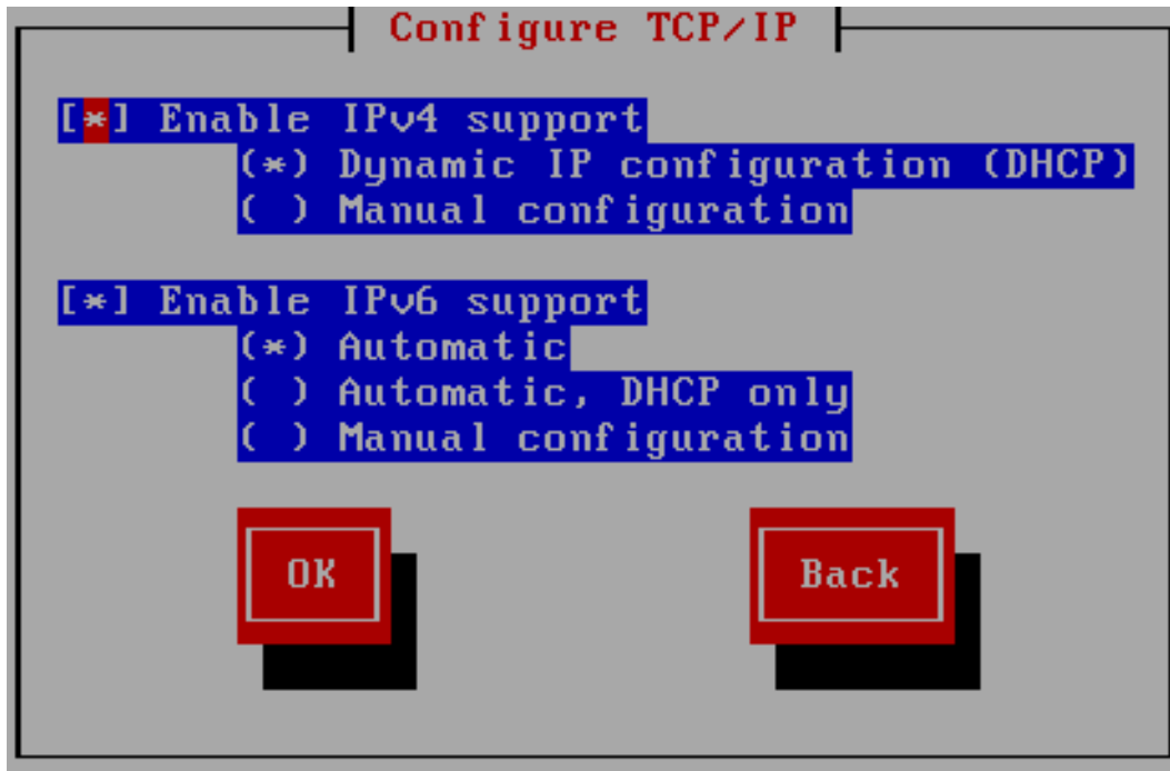
Figure 15.8. Configure TCP/IP
