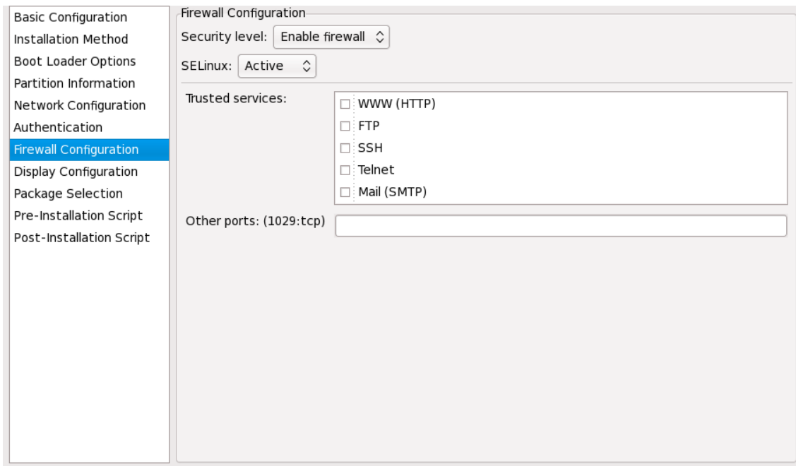
Figure 33.10. Firewall Configuration
