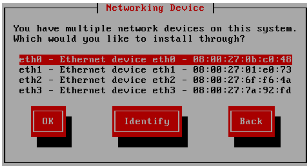
Figure 8.6. Networking Device
