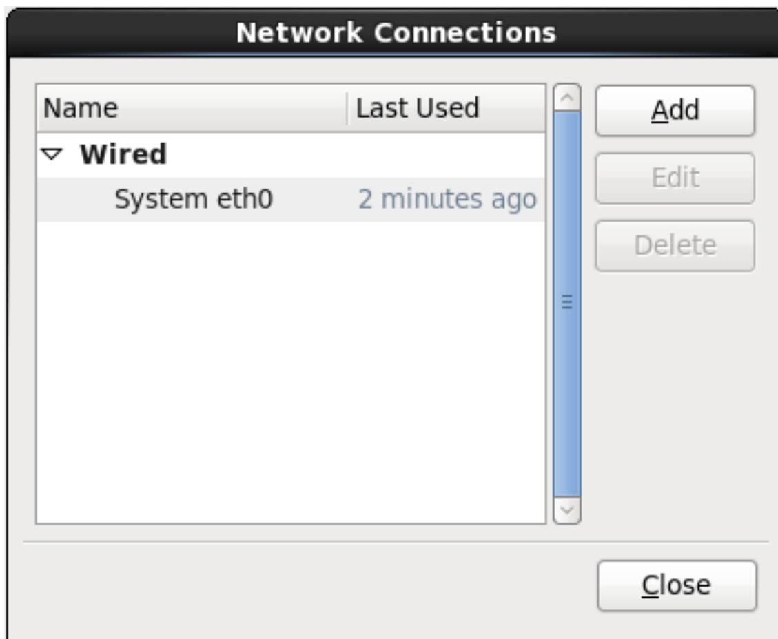
Figure 9.25. Network Connections
