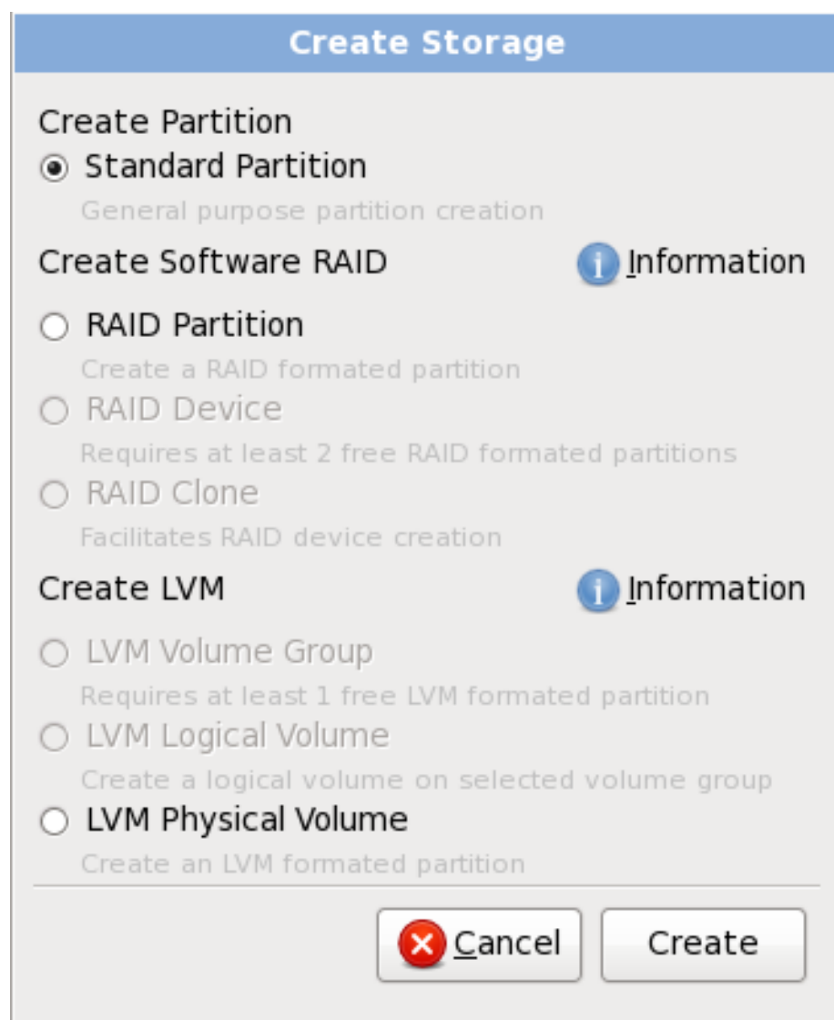
Figure 23.39. Creating Storage
