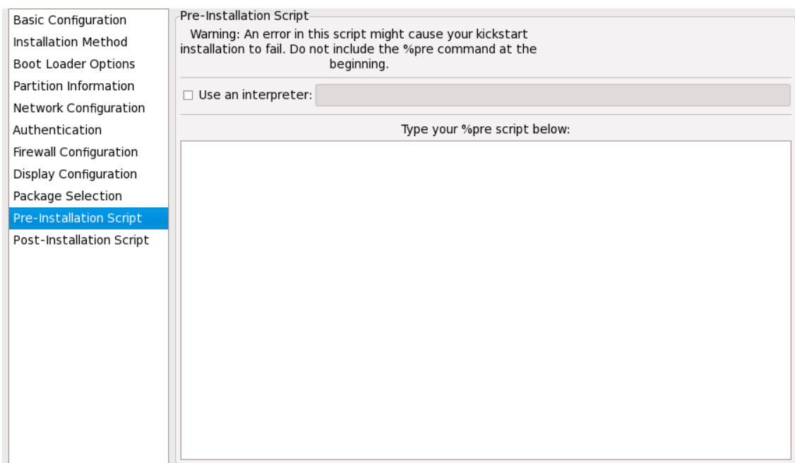
Figure 33.13. Pre-Installation Script
