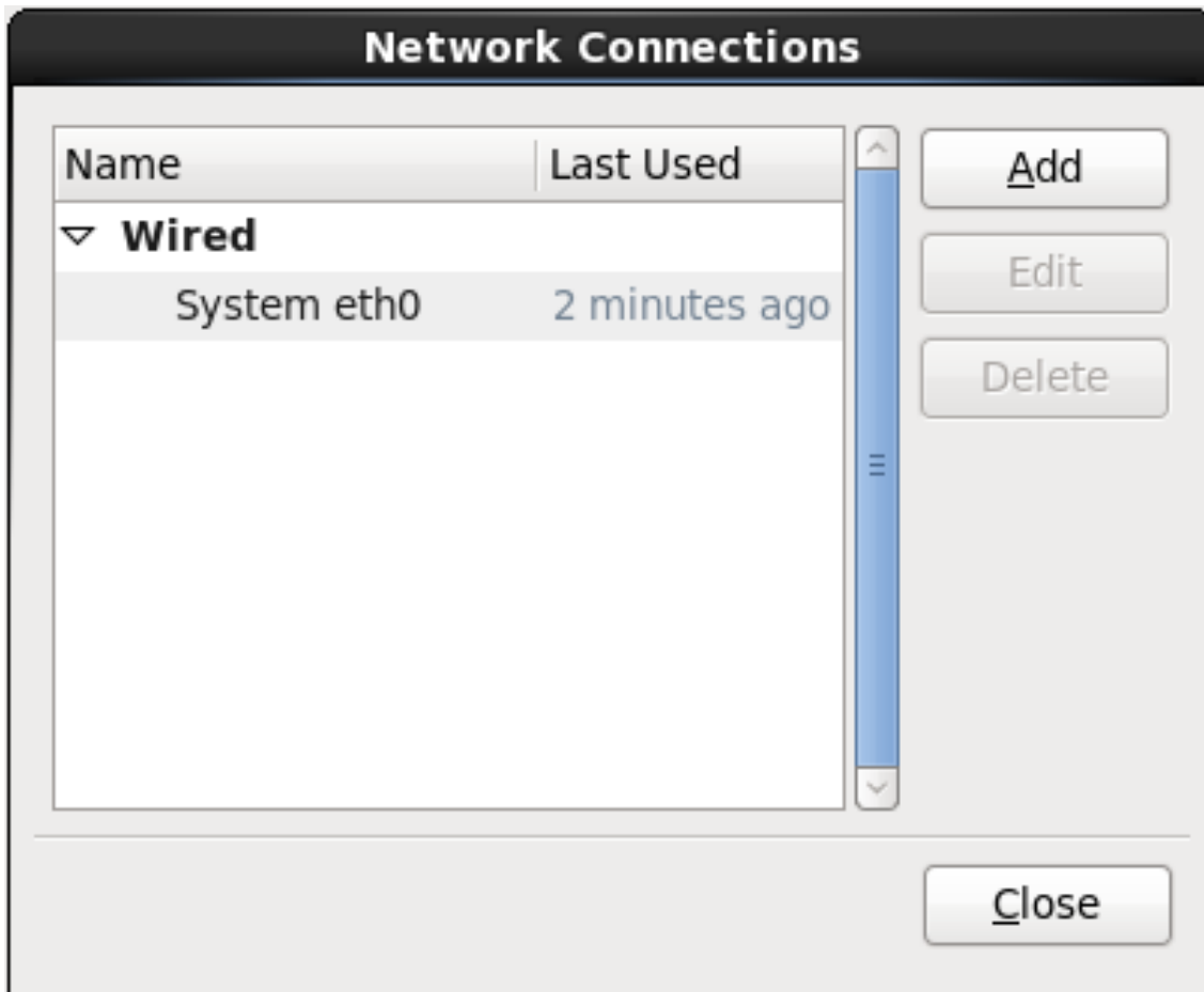
Figure 16.51. Network Connections
