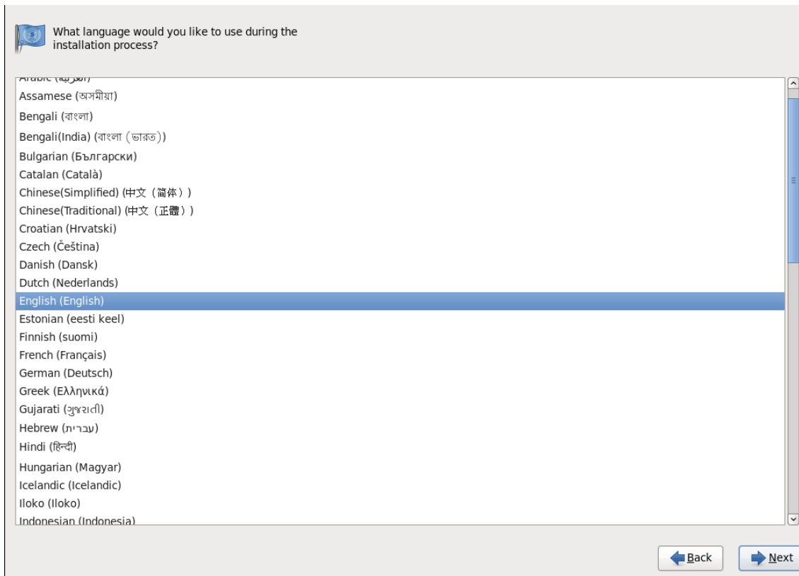
Figure 9.2. Language Configuration
