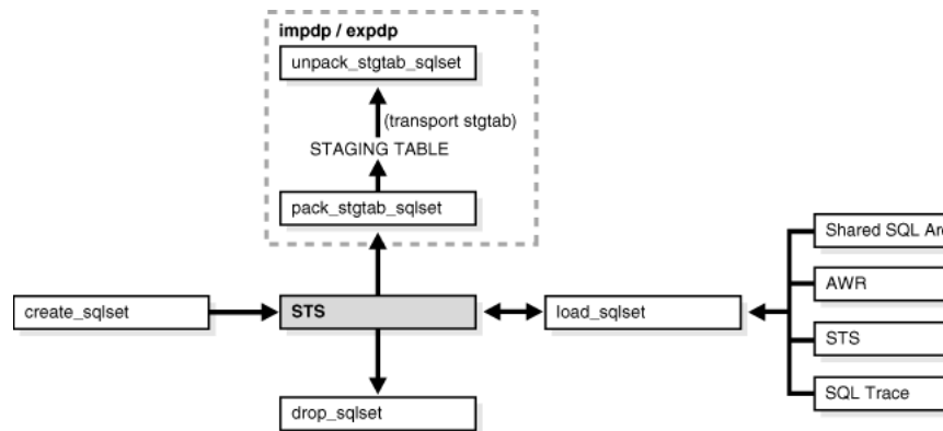
Figure 17-3 SQL Tuning Sets APIs
