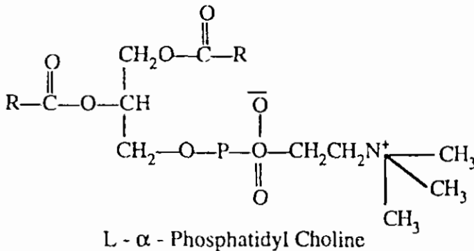
Lecithin
