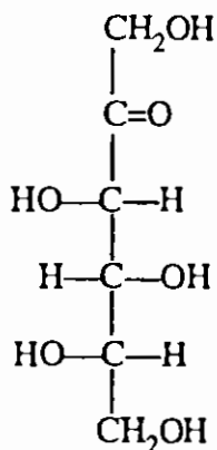
L—Sorbosc
