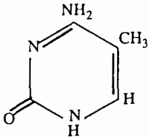
5 - Methyl cytosine
