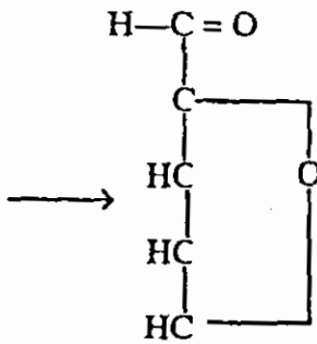
Furfural
