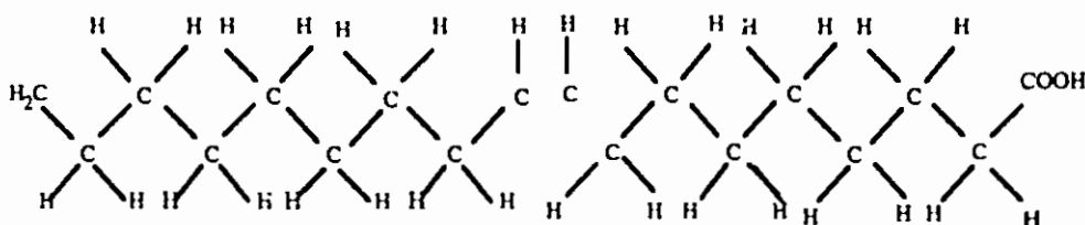
(I) Cis
