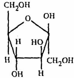
\beta -D-fructofuranose
