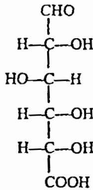
D- glucuronic
