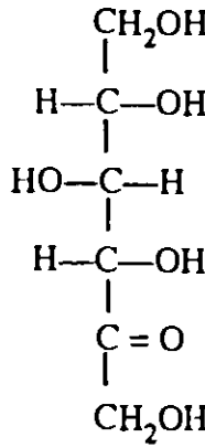
L—Sorbse
