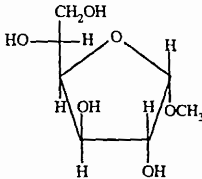
Methyl \alpha -D-glucofuranoside
