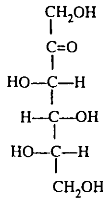
L—Sorbse
