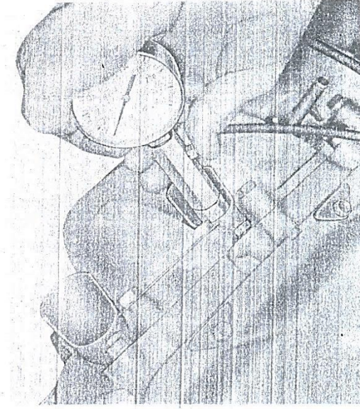
Fig. 8.5 Using cylinder-compression tester.
