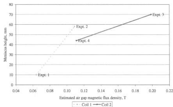
Figure 7. The obtained meniscus height (+/- 5mm) is plotted against the magnetic flux density estimated using Equation (2) for the long coil (Coil 1) and the multi-layer coil (Coil 2).
