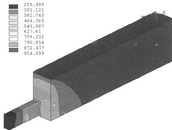
Figure 3: Temperature solution of the base case model
