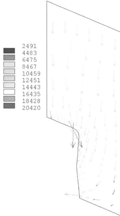
Figure 7: Current density with variable contact resistance values
