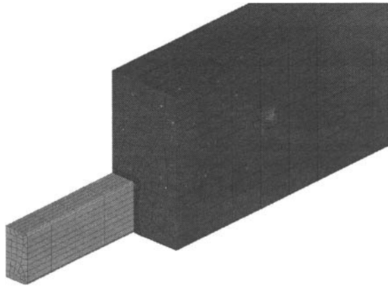
Figure 1: Mesh of the base case model
