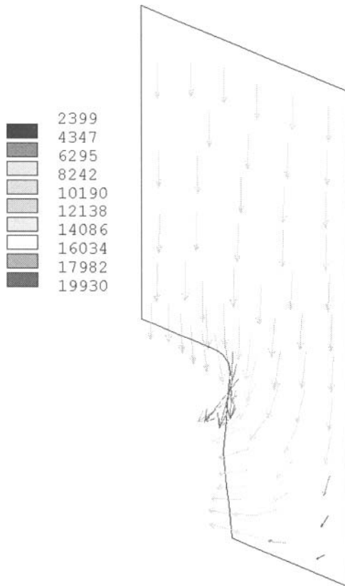
Figure 5: Current density with constant contact resistance values
