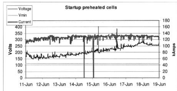
Figure 6: Start-up of preheating cells
