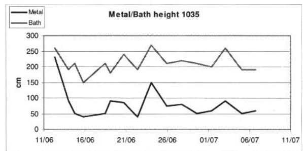
Figure 10: Metal and bath height development
