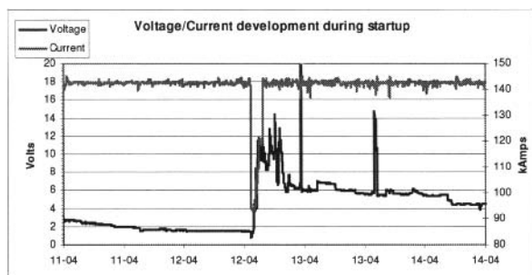
Figure 4: Voltage development during start up
