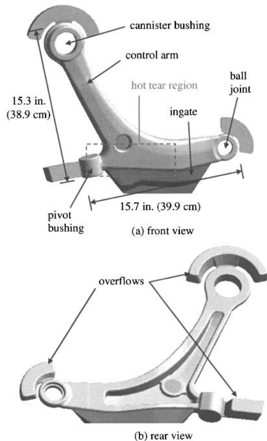
Figure 1. Original AM60B control arm geometry.
