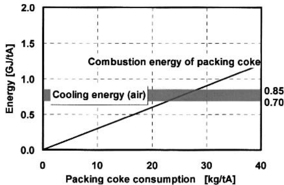
Figure 10: Influence of packing coke consumption on anode cooling
