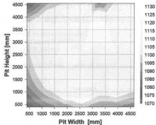
Figure 4: Real pit temperature distribution in °C
