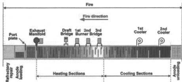
Figure 3: Arrangement of firing equipment
