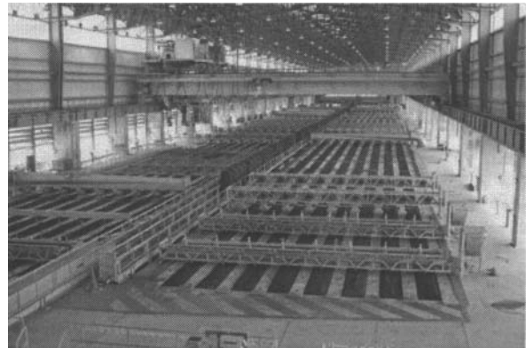
Figure 2: Overview of bake furnace ABF 1 in operation
