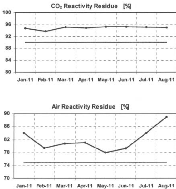
Figure 6: CO 2 and air reactivity residue
