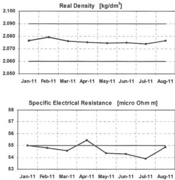
Figure 5: Real density and specific electrical resistance
