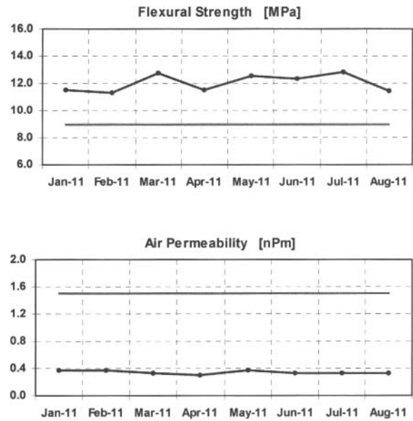
Figure 7: Flexural strength and air permeability
