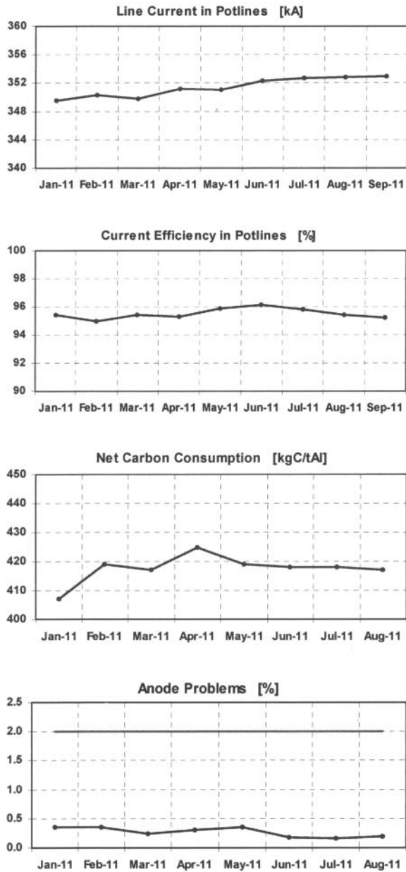
Figure 8: Evolution of key pot performance figures
