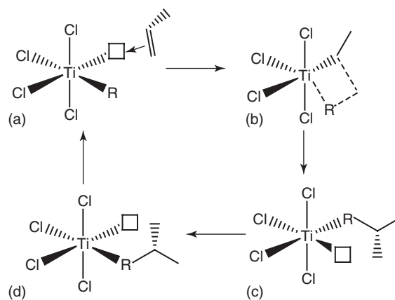
Figure 5.9 The Cossee–Arlman mechanism a) Olefin coordination, b) Olefin concerted insertion, c) Insertion step, d) Chain migration.
