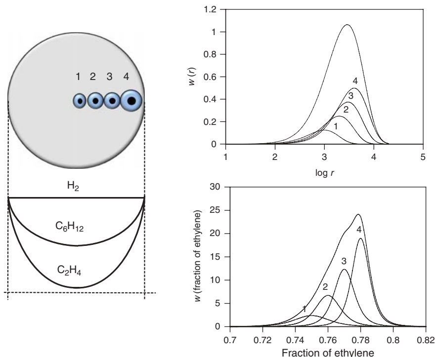
Figure 5.14 Effect of radial concentration profiles on the chain length and chemical composition distributions of an ethylene/1-hexene copolymer (four microparticle layers were used for simplicity sake: many more layers are required in an actual MGM simulation) [131].
