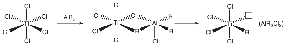
Figure 5.8 Active species formation in a classical Ziegler–Natta catalyst.
