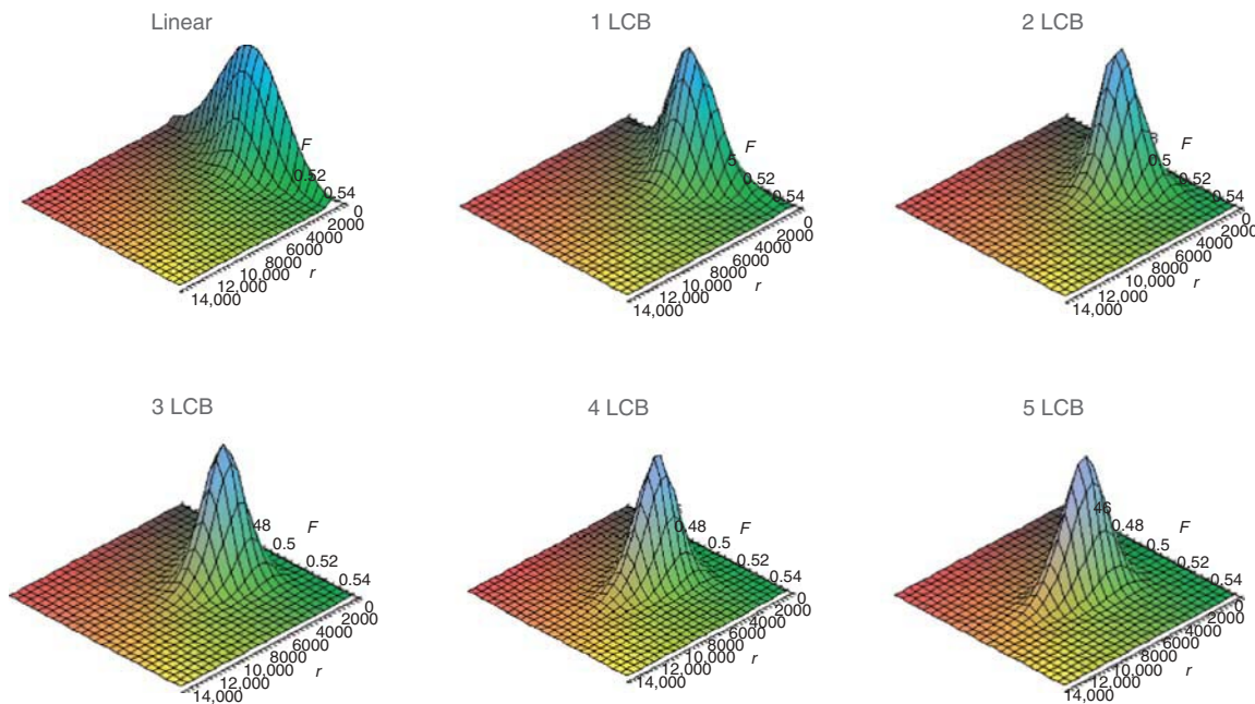
Figure 5.11 Trivariate distribution for a model polymer. (See insert for the color representation of the figure.)
