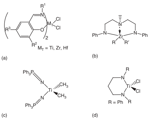
Figure 5.6 Postmetallocenes' catalytic systems: (a) phenoxyimine (FI), (b) Schrock, (c) Stephan, (d) McConville.
