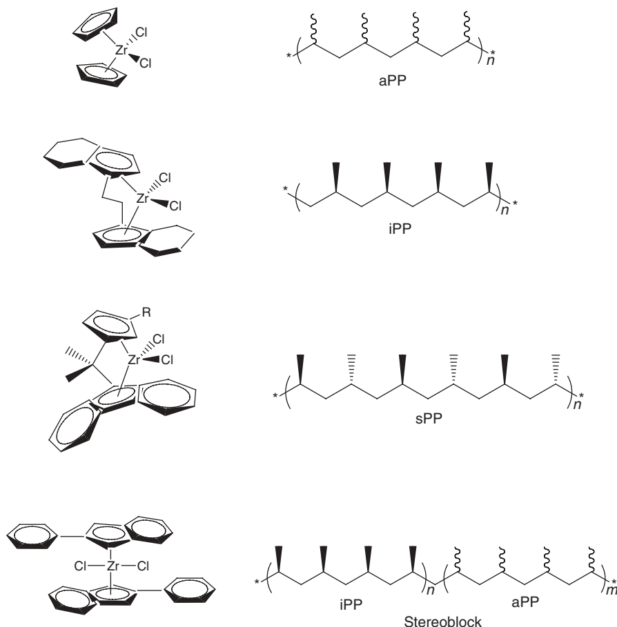
Figure 5.3 Zirconocene precursors for propylene polymerization. aPP, atactic polypropylene; sPP, syndiotactic polypropylene.
