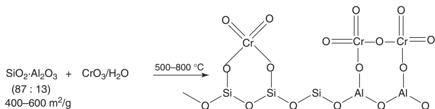
Figure 5.1 The Phillips catalyst synthesis.
