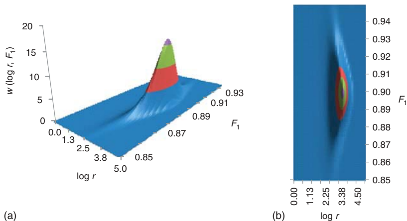
Figure 5.10 The Stockmayer distribution for a copolymer made with a single-site catalyst. a) Three-dimensional plot, b) Bird's eye view. (See insert for the color representation of the figure.)
