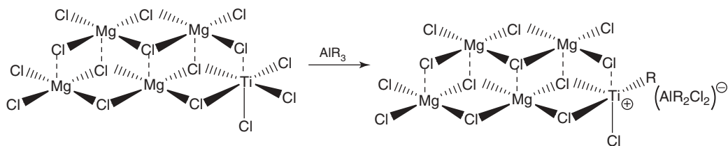
Figure 5.2 The classical Ziegler–Natta heterogenized catalyst.
