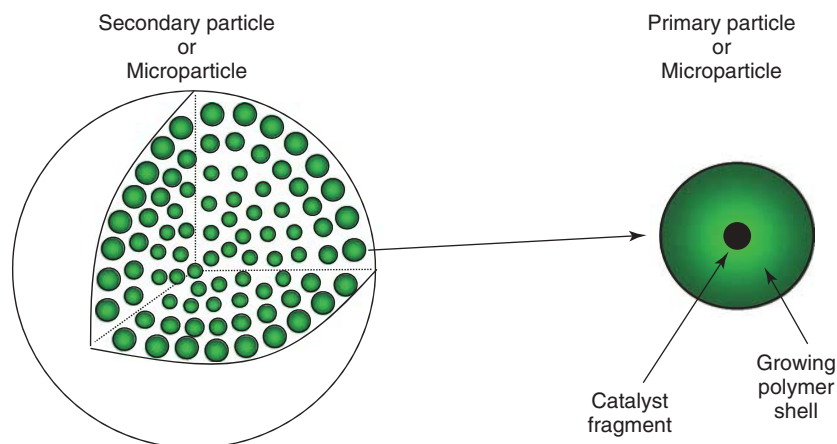
Figure 5.13 The multigrain model (MGM). (See insert for the color representation of the figure.)
