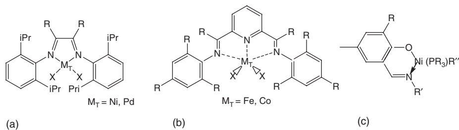
Figure 5.7 Main late transition-metal catalysts: (a) Versipol catalyst, (b) Brookhart/Gibson, (c) Grubbs/Johnson.
