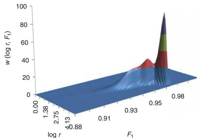
Figure 5.12 Simulated chain length and chemical composition distributions of a polymer made from a three-site catalyst. (See insert for the color representation of the figure.)
