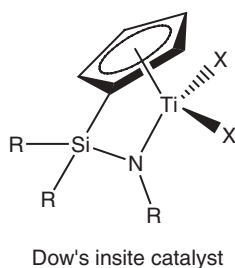
Figure 5.5 Constrained geometry catalyst (CGC).
