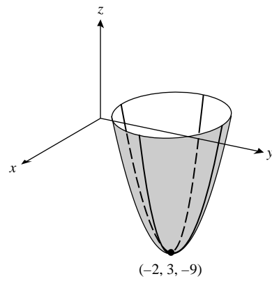
37. Circular paraboloid
