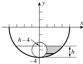
59. (a) 0 \leq h < 2
