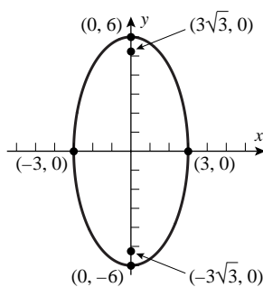
(b) \frac{x^2}{9} + \frac{y^2}{36} = 1 , c^2 = 36 - 9 = 27 , c = 3\sqrt{3} .
