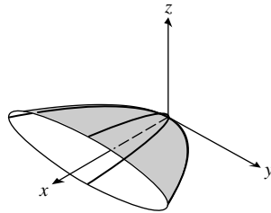
28. Elliptic paraboloid
