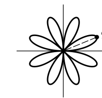
45. Eight-petal rose
