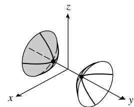
22. Hyperboloid of two sheets
