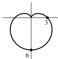
15. Cardioid
