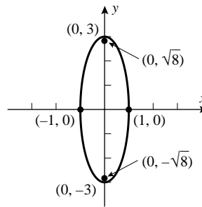
(b) \frac{x^2}{1} + \frac{y^2}{9} = 1 , c^2 = 9 - 1 = 8 , c = 2\sqrt{2} .
