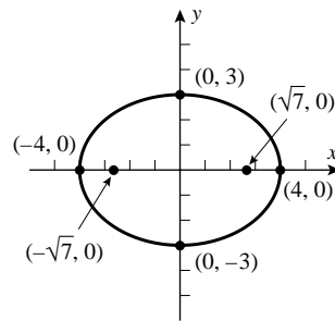
7. (a) c^2 = 16 - 9 = 7 , c = \sqrt{7} .
