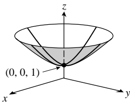
37. Circular paraboloid
