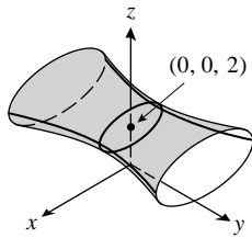
38. Hyperboloid of one sheet
