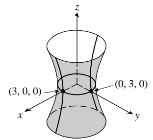
18. Hyperboloid of one sheet
