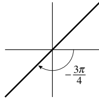
22. Line
