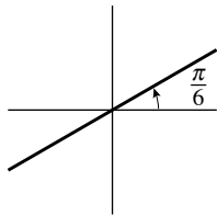
13. Line
