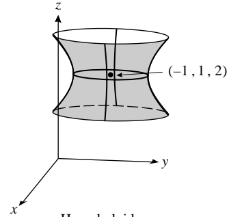
40. Hyperboloid of one sheet
