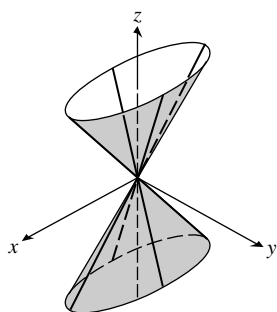
19. Elliptic cone
