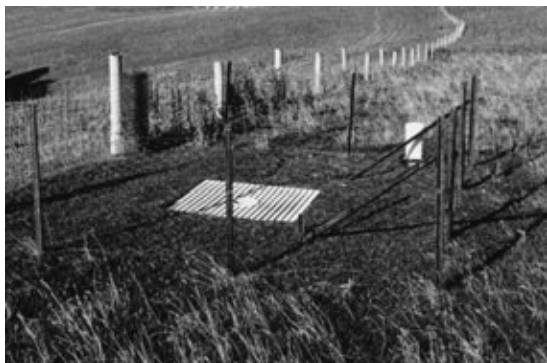
Figure 2.6 Surface rain gauge with non-splash surround.
