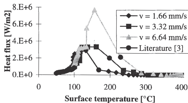
Figure 7. Influence of speed on q(T_{surf}) .
