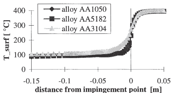
Figure 9. Influence of alloy on T_{surf}(y) .
