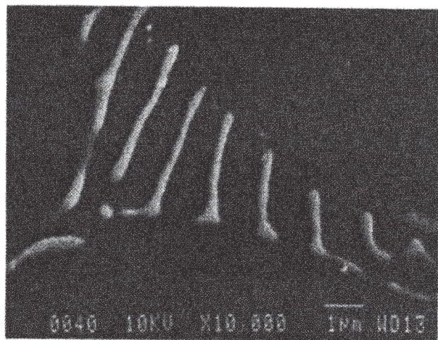
(c) grain-refined Al-0.5wt.%Fe-0.1wt.%Si
