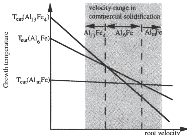
(b) for ternary Al-Fe-Si alloy with grain refiner
