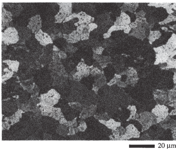
Figure 5: Grain structure obtained when 20 ppt Al-Ti-C grain-refiner is used. The sample was grown at 60 mm min -1 .
