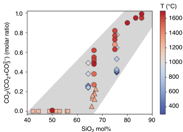
Figure 16.1 Molar ratio, \text{CO}_2/(\text{CO}_2+\text{CO}_3^{2-}) as a function of silica content at 300 °C–1700 °C for melts and glasses along the \text{NaAlO}_2\text{-SiO}_2 join from Brooker et al. (1999) (circles), andesite melts from King and Holloway (2002) (triangles), phonolite and dacite melts from Korschak and Keppler (2014) (diamonds), and mafic melts from Shishkina et al. (2014) (squares). The data from Brooker et al. (1999) and King and Holloway (2002) were obtained at 1–2 GPa and 1 GPa, respectively. Shishkina et al. (2014) did not observe any molecular \text{CO}_2 species for the range of mafic melts investigated at 1200 °C–1250 °C up to 0.5 GPa. Korschak and Keppler (2014) reported that the carbon speciation is independent of pressure in the pressure range of 3–20 GPa at temperatures of up to 1000 °C; however, Brooker et al. (1999) observed a negative correlation of \text{CO}_2/(\text{CO}_2+\text{CO}_3^{2-}) and pressure. In either case, the effect of pressure and temperature is secondary to the effect of silica content on carbon's speciation. See electronic version for color representation of the figures in this book.
