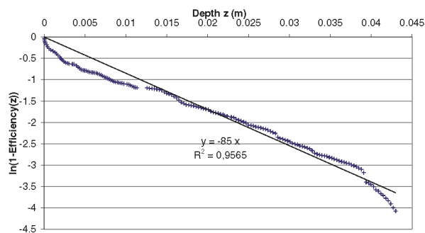
Figure 13. Filtration law linking filtration efficiency and filter depth
