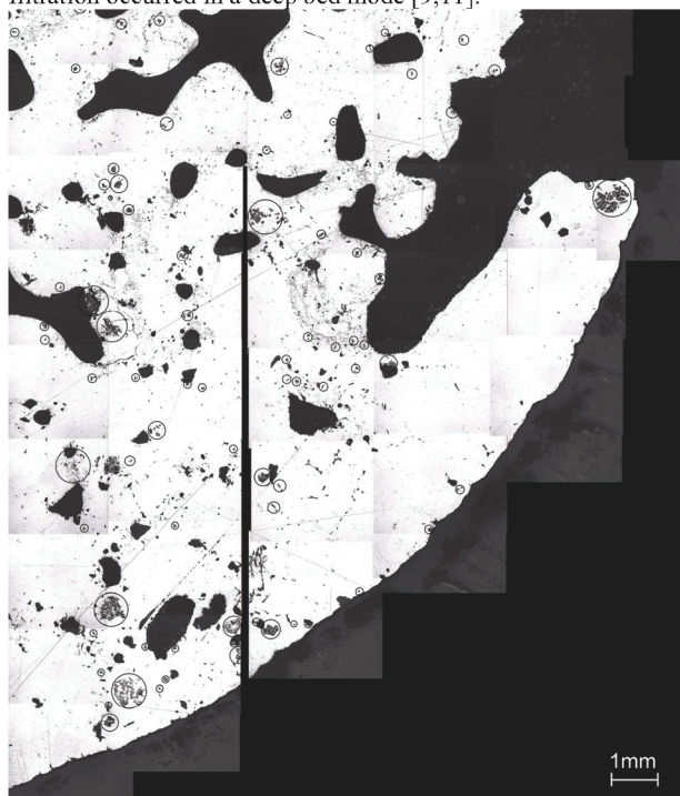
Figure 11. Transversal metallographic cut of a quarter of the filter (100µm from the filter inlet)
