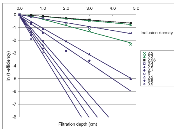
Figure 5. Representation of ln(1-Efficiency) in function of the filter depth for a range of inclusion densities
