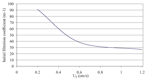
Figure 9. Computed influence of filtration speed on initial filtration coefficient (60ppi filter, 50µm-3200 kg/m3 inclusions)
