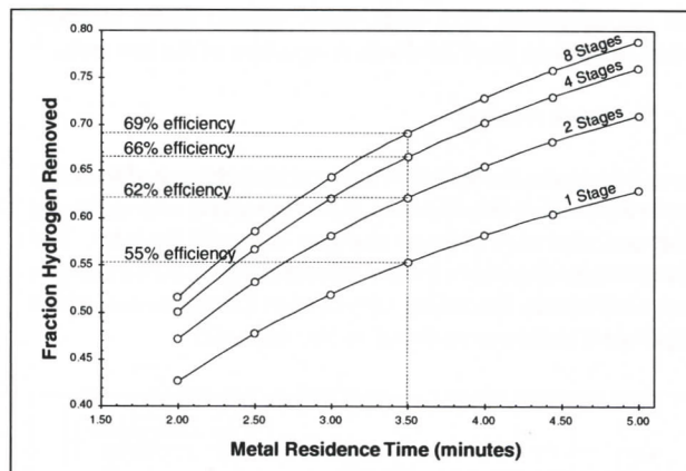
Figure 2 : Effect of increased treatment stages on in-line hydrogen removal.
