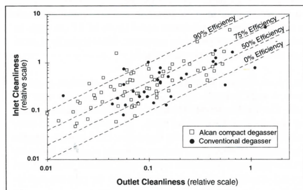
Figure 4 : Global metal cleanliness results for in-line degassing processes compared to the Alcan compact degasser.
