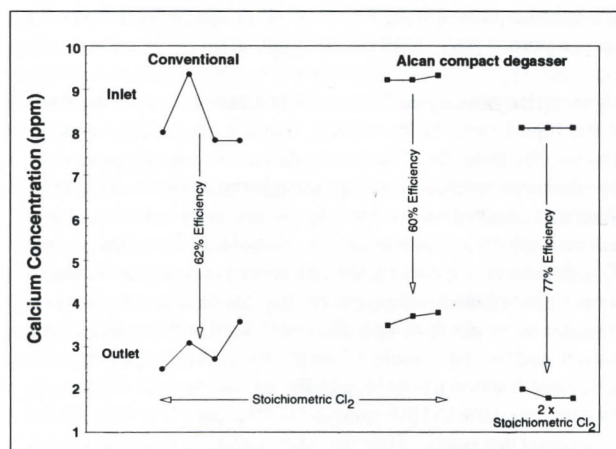
Figure 5 : Comparison of the calcium removal performance of the Alcan compact degasser vs conventional degassing technology.
