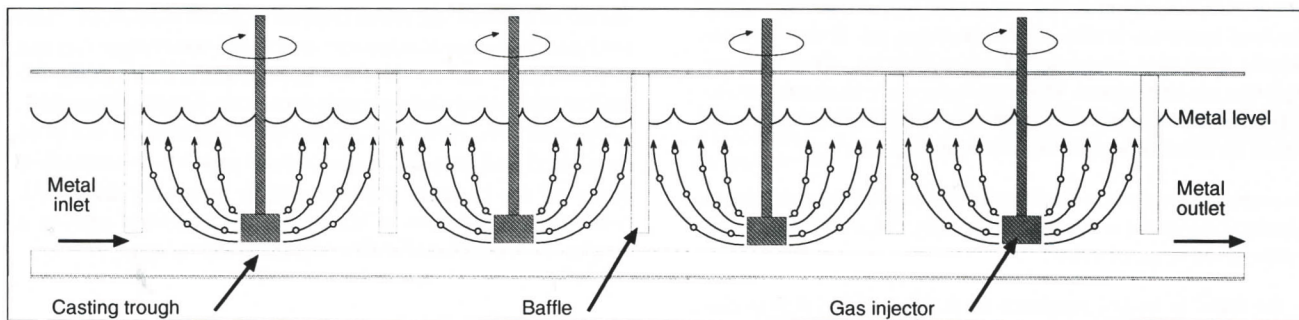
Figure 1 : Schematic representation of a multi-rotor compact degassing unit.
