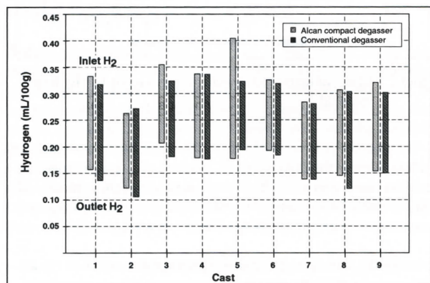
Figure 3 : Hydrogen removal performance of the Alcan compact degasser compared to conventional degassing technology.
