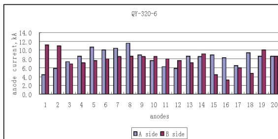
Figure 3a Anode current distribution of QY-320-6
