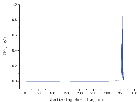
Figure 2a Original CF 4 Emission Trace of QY-320-7
