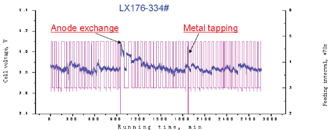
Figure 5 Trends of cell voltage and feeding interval during measurement
