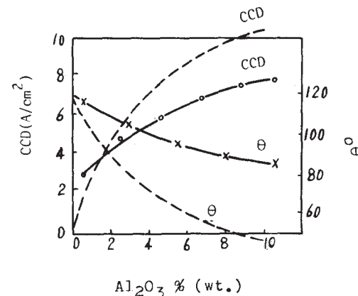
Fig. 3 ccd = f(Al_2O_3\%) , \theta = f(Al_2O_3\%) . curves ----- obtained by Belyaev, curves ——— this paper
