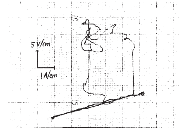
Fig. 1 I-V curve in aluminium electrolysis. ( C.R. = 2.98, Al_2O_3 8.5%, 1050°C)
