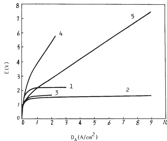
Fig. 5 Relationships between anodic current density and back EMF of aluminium electrolysis cell. 1--- back EMF of platinum anode, 2--- back EMF of carbon anode, 3--- back EMF obtained by Abramov, 4--- cell voltage of platinum anode, 5--- cell voltage of carbon anode.
