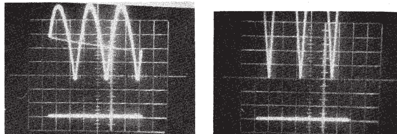
Photo B. Oscillograms in aluminium electrolysis with carbon anode.
