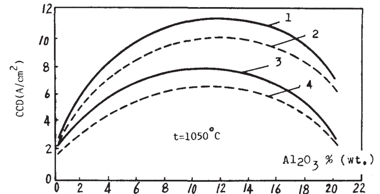
Fig. 2 Critical current densities on carbon anodes in aluminium electrolysis. Na_3AlF_6 ( NaF/ AlF_3 mole ratio = 3.0) + Al_2O_3 (saturated), 1-new anode, 2-anode after AE, 3-new anode, with the addition of Al, 4-anode after AE, with the addition of Al.
