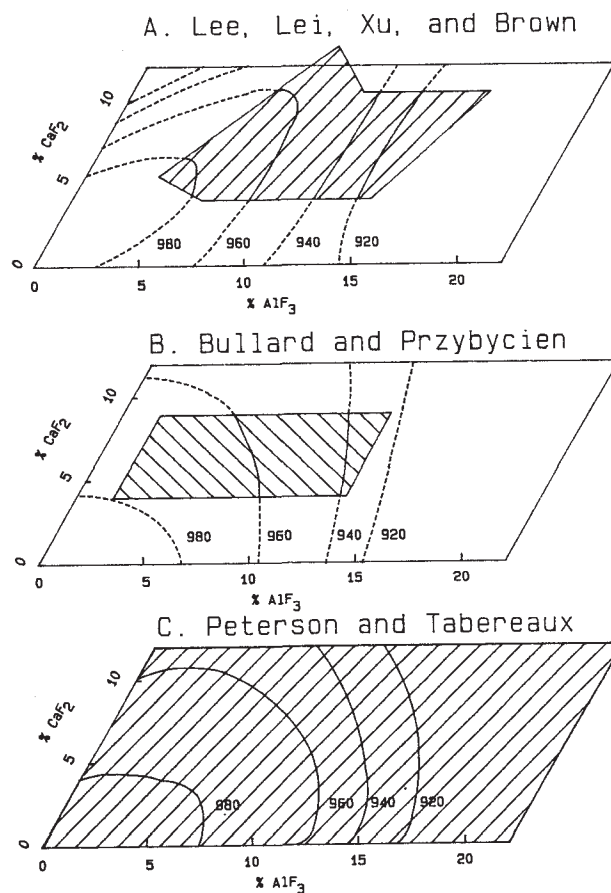
Figure 6 • Comparison of liquidus isopleths based on three different models in the 97% \text{Na}_3\text{AlF}_6 - 3 \text{Al}_2\text{O}_3 plane. The experimental range from which each model was derived is shown in cross hatching.
