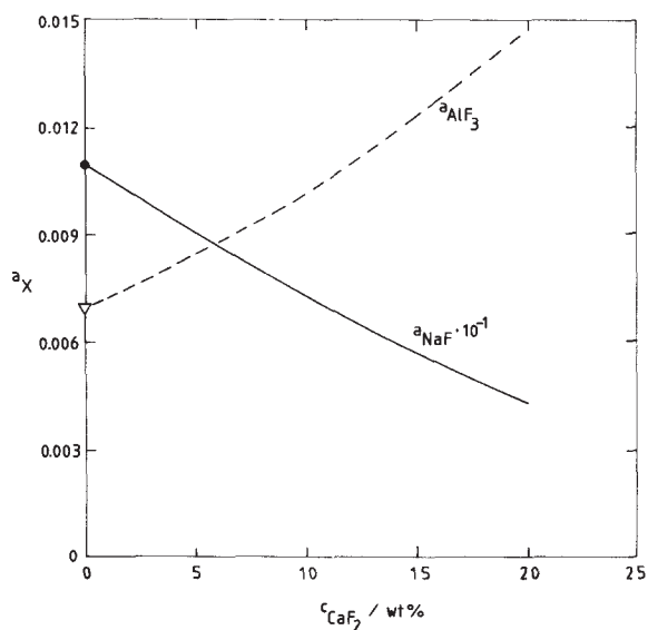
Fig. 5. Estimated activities of NaF and AlF 3 as a function of CaF 2 addition at CR = 1.80 and 1020°C.
