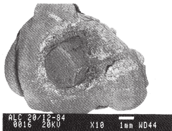
Fig. 10. SEM micrograph of electrodeposited carbon. Deposition conditions: I=1.0 A, t=1020^{\circ}\text{C} , \text{CR}=1.50 . The smooth area in the center of the sample is the contact area to the end of the vitreous carbon electrode (3 mm diam.).
