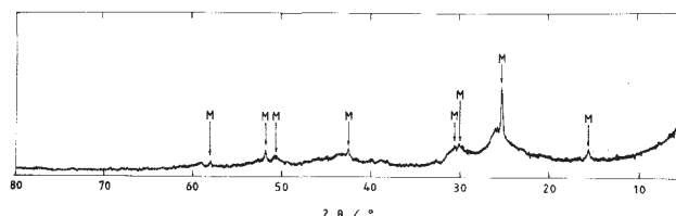
Fig. 7. X-ray diffractogram of electrodeposited carbon. Peaks marked "M" were identified as being due to salt compound (NaAlF 4 , Na 5 Al 3 F 14 ). Deposition conditions: CR=1.50, t=1000°C, I=2A. Diffraction angle scan 5-80°.
