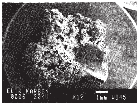
Fig. 9. SEM micrograph of electrodeposited carbon. Deposition conditions: I=10.0 A, t=1020°C, CR=1.50. The smooth area visible on the picture is the contact area to the vitreous carbon electrode (3 mm diam.).
