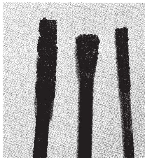
Fig. 6. Carbon deposits on rods made of; 1: iron (3 mm), 2: vitreous carbon (3 mm) 3: tungsten (2 mm). CR=1.50, t=1000°C, total current 1-5 A.
