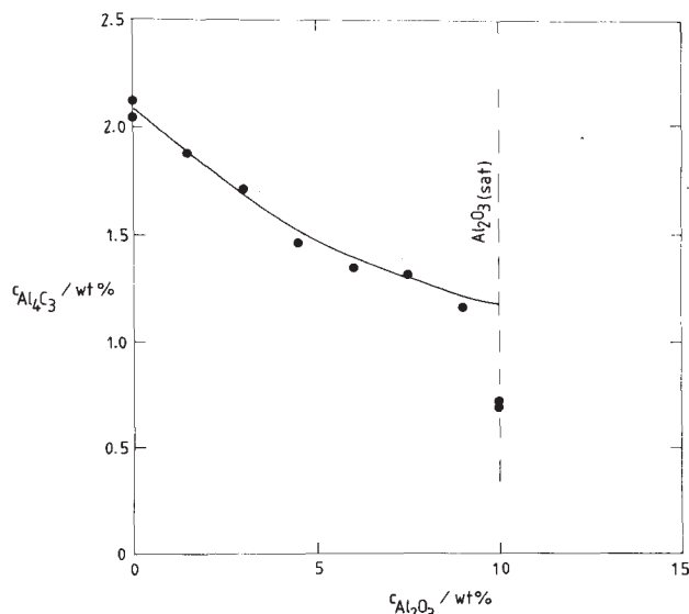
Fig. 3. Concentration of dissolved aluminium carbide as a function of the concentration of alumina in NaF-AlF 3 -Al 2 O 3 melts at CR=1.80 and 1020 ± 2°C. (●): experimental data. The full line is based on calculated solubilities according to eq. (8).
