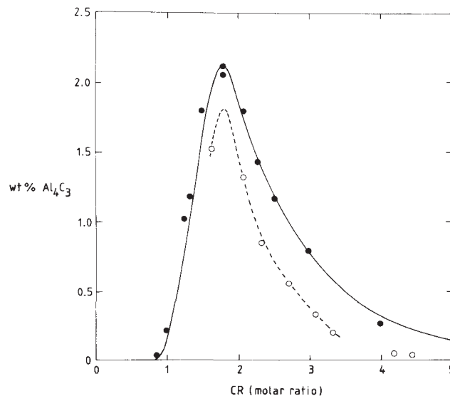
Fig. 1. Concentration of dissolved aluminium carbide in \text{NaF}-\text{AlF}_3 melts as a function of the \text{NaF}/\text{AlF}_3 molar ratio (CR) 1020 \pm 2^\circ\text{C} . ●: present work, ○: Dewing [1]. The full line is based on a dissolution reaction according to eq. (8) (see text).
