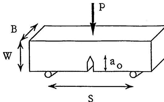
Figure 3 Three-point bending test on single. Edge notched beam.
