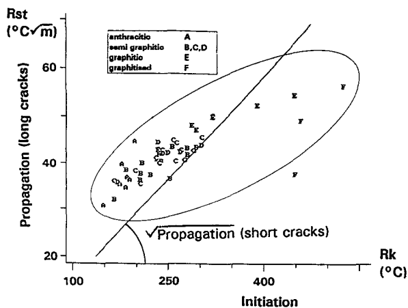
Figure 8 Thermal shock resistance diagram. Application to industrial cathodic material.
