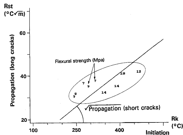
Figure 7 Thermal shock resistance diagram: application on industrial anodes. Weight of the flexural strength.
