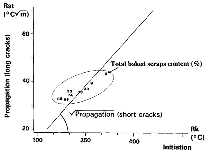
Figure 5 Influence of the baked scraps content on the resistance to thermal shock [benchscale anodes].
