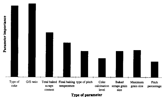
Figure 6 Influence of the different parameters tested on the resistance to thermal shock (benchscale anodes).
