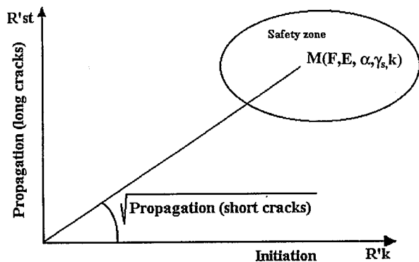
Figure 2 Diagram for SOFT thermal shock.
