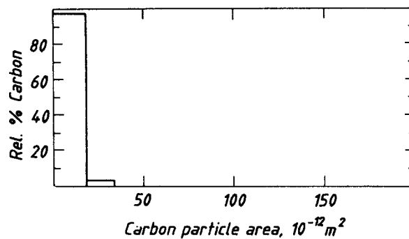
Fig. 9. Dust particle size distribution in pot E14, sample 7 (prebaked).
