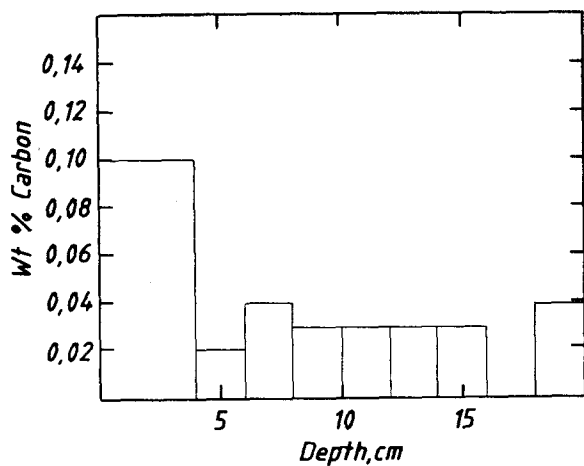
Fig. 14. Dust content vs. bath depth, pot B31H (prebaked.)
