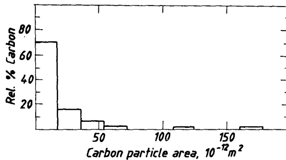
Fig. 3 Dust particle size distribution in pot E14, sample 1 (prebaked).
