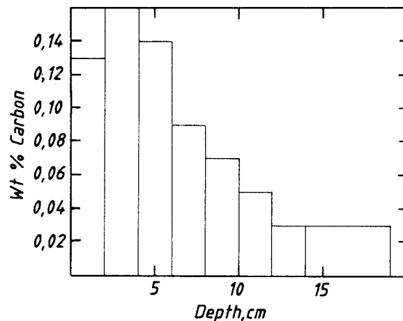
Fig. 10. Dust content vs. bath depth, pot R27A (Soderberg).
