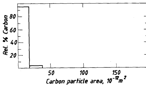
Fig. 4 Dust particle size distribution in pot E14, sample 2 (prebaked).
