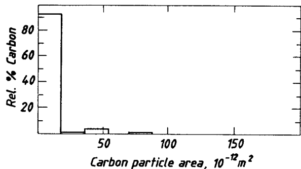
Fig. 7. Dust particle size distribution in pot E14, sample 5 (prebaked).
