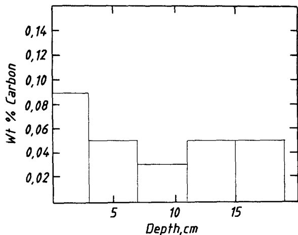
Fig. 12. Dust content vs. bath depth, pot K40A (prebaked.)
