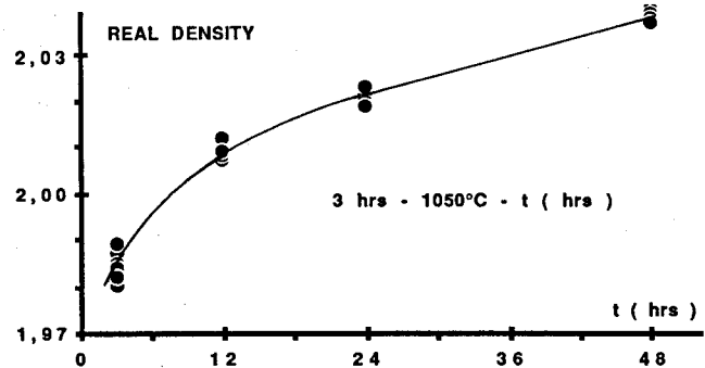
Figure 2 - Time at temperature versus real density.
