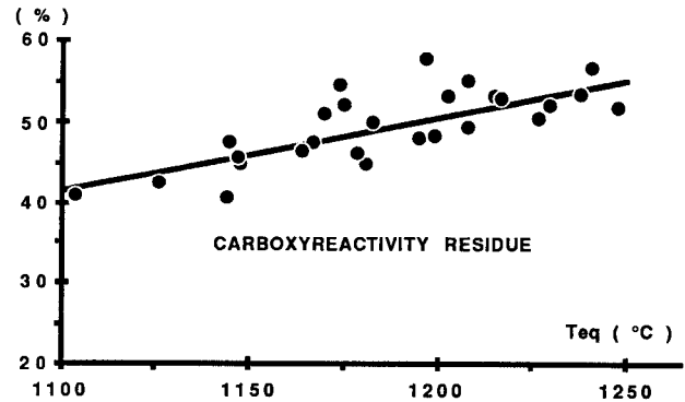
Figure 4 - Carboxyreactivity residue versus equivalent temperature.
