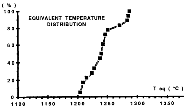
Figure 10 - Equivalent temperature distribution (New furnace).
