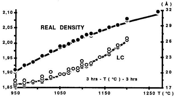
Figure 3 - Calibration curve : Real density/Lc versus equivalent temperature.
