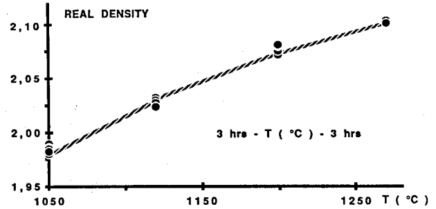
Figure 1 - Treatment temperature versus real density.
