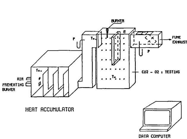
Figure 7 - Burner testing unit.
