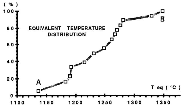
Figure 5 - Equivalent temperature distribution (Old furnace).
