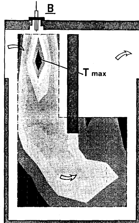
Figure 8 - Comparison of two different types of burners. Isotherms recorded after 300 seconds' operation.
