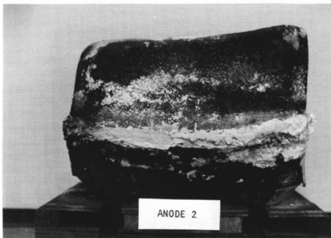
FIGURE 21. HIGH TEMPERATURE ANODES
