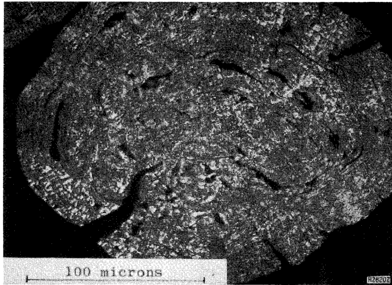
Figure 11 Onion-Like Microstructure of a Fluid Coke Particle
