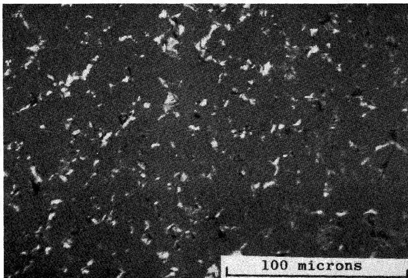
Figure 21 Structure of Baked Mesophase Coke Containing 20% Lampblack
