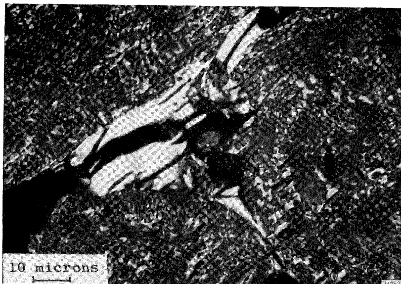
Figure 23 Microstructure of Pitch-Coke Bond from Petroleum Pitch Containing No Primary QI
