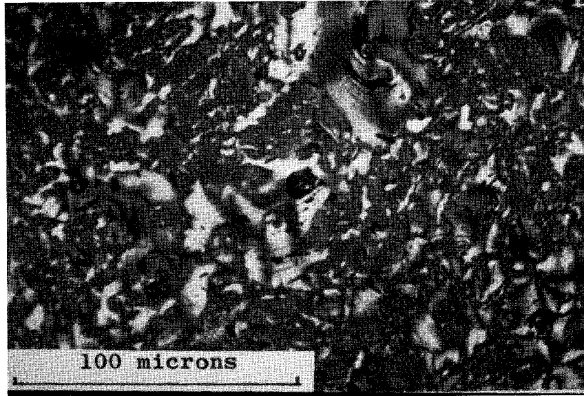
Figure 18 Structure of Baked Coke for Coal-Tar Pitch Containing 10% QI
