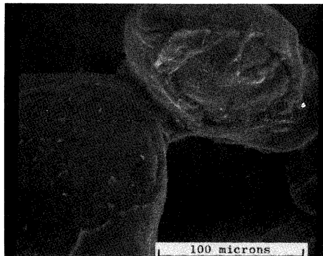
Figure 12 Fracture Surface in a Baked Fluid Coke Composite with Coal-Tar Pitch Binder
