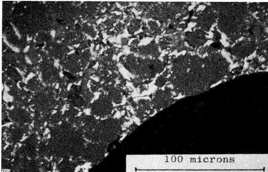
Figure 20 Structure of Baked Coke for Coal-Tar Pitch Containing 20% QI
