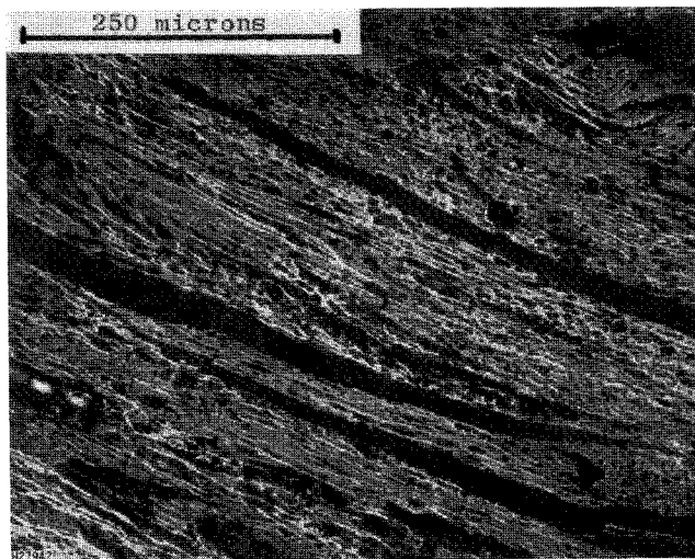
Figure 3 Ordered Filler Coke Structure
