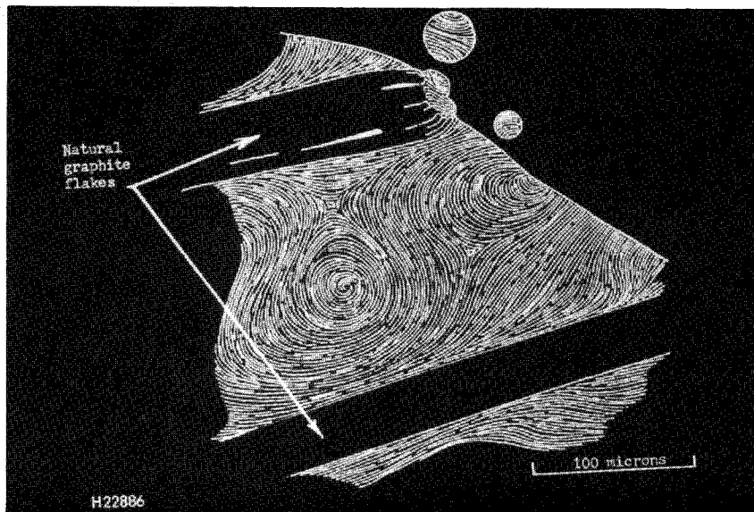
Figure 7 Alignment of Mesophase Layers With Graphite Surfaces
