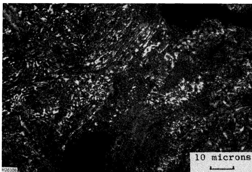
Figure 24 Microstructure of Pitch-Coke Bond from Coal-Tar Pitch Containing 27% Primary QI
