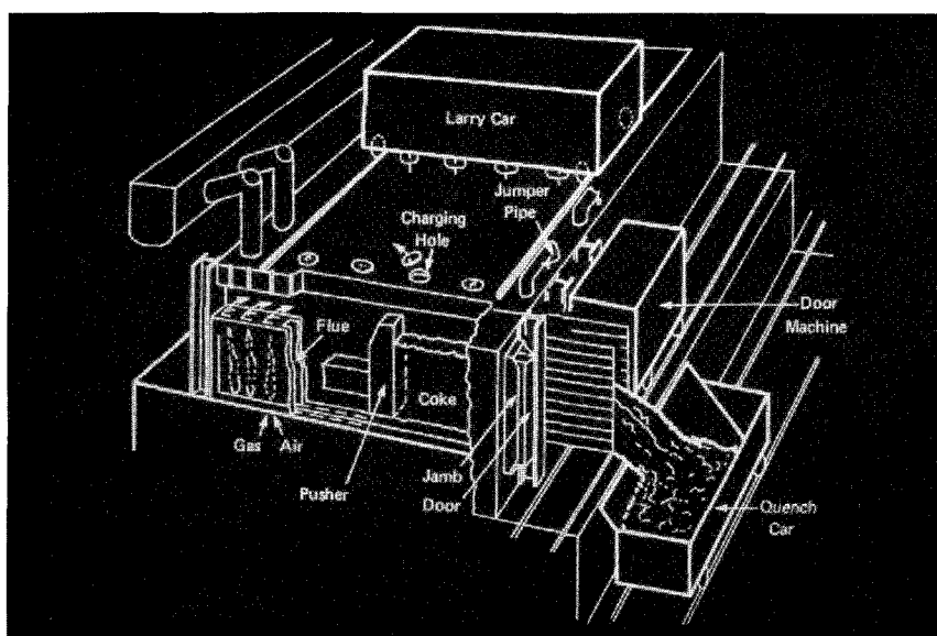
Figure 27 Diagram of Coal Coke Oven Structure
