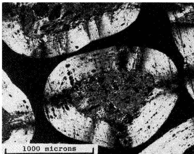
Figure 13 Microstructure of Pyrocarbon-Coated Fluid Coke
