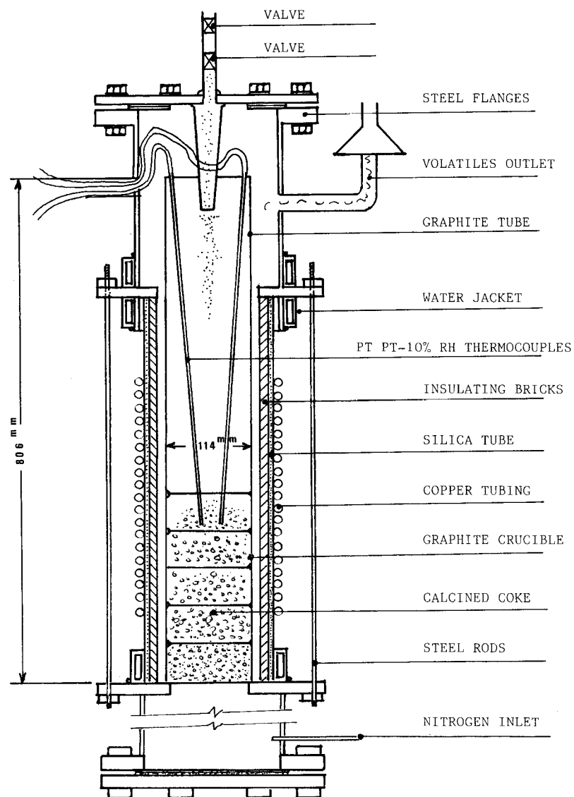
Fig. 1 - Laboratory Induction Furnace Used for Calcination.
