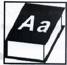
dictionary
