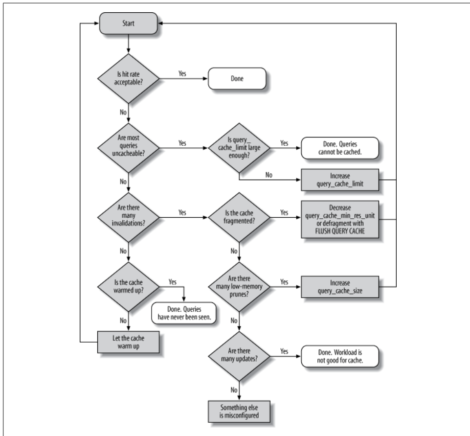
Figure 7-5. How to analyze and configure the query cache
