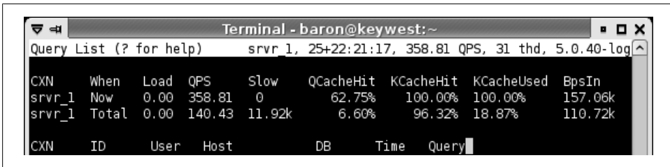
Figure 16-9. Adding a header (result)
