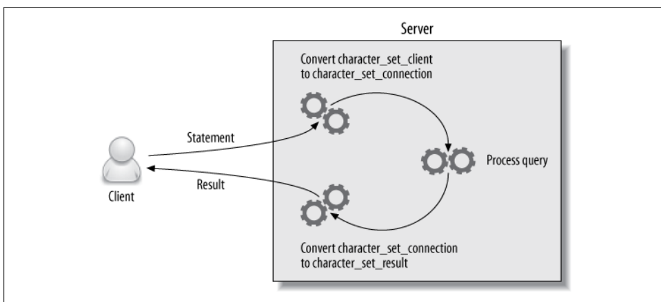
Figure 7-2. Client and server character sets
