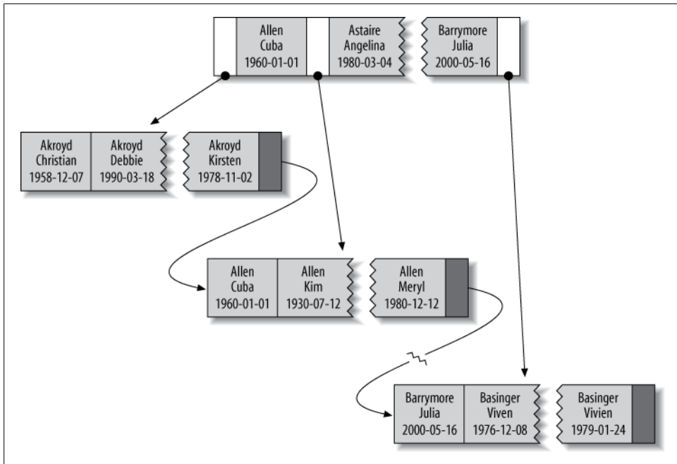
Figure 5-2. Sample entries from a B-Tree (technically, a B+Tree) index
