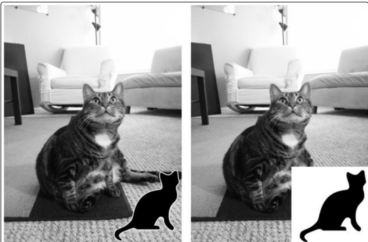
Figure 17-13. The image zophie.png resized and the logo added (left). If you forget the third argument, the transparent pixels in the logo will be copied as solid white pixels (right).
