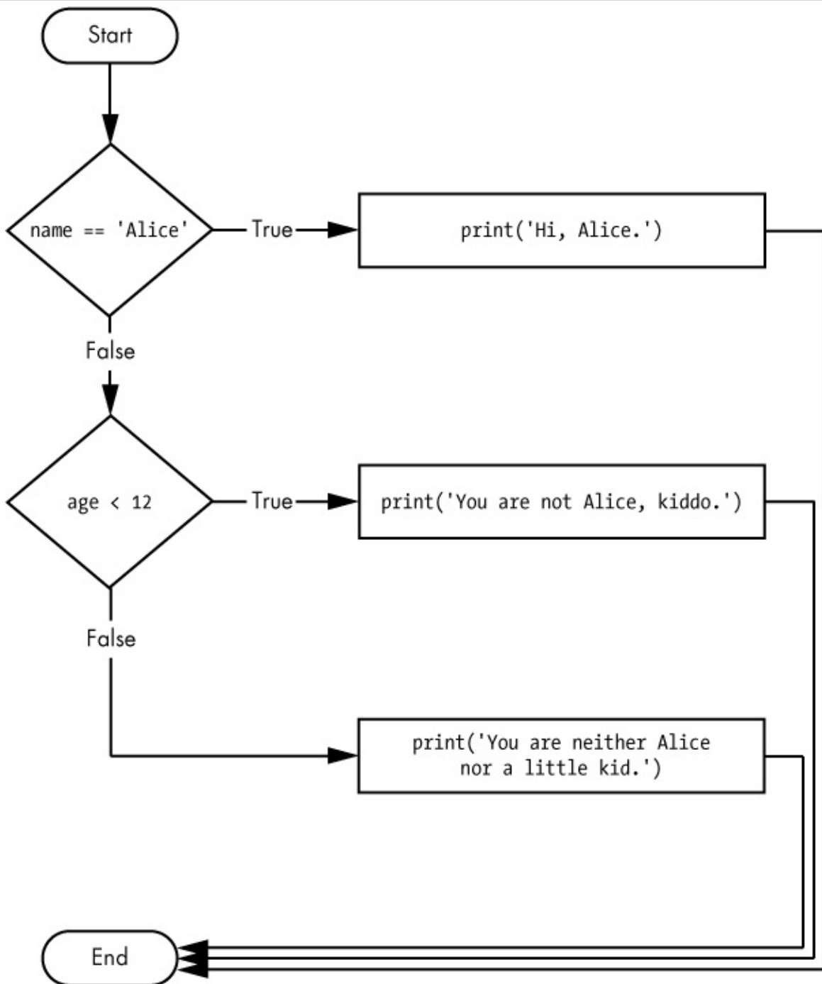
Figure 2-8. Flowchart for the previous littleKid.py program
