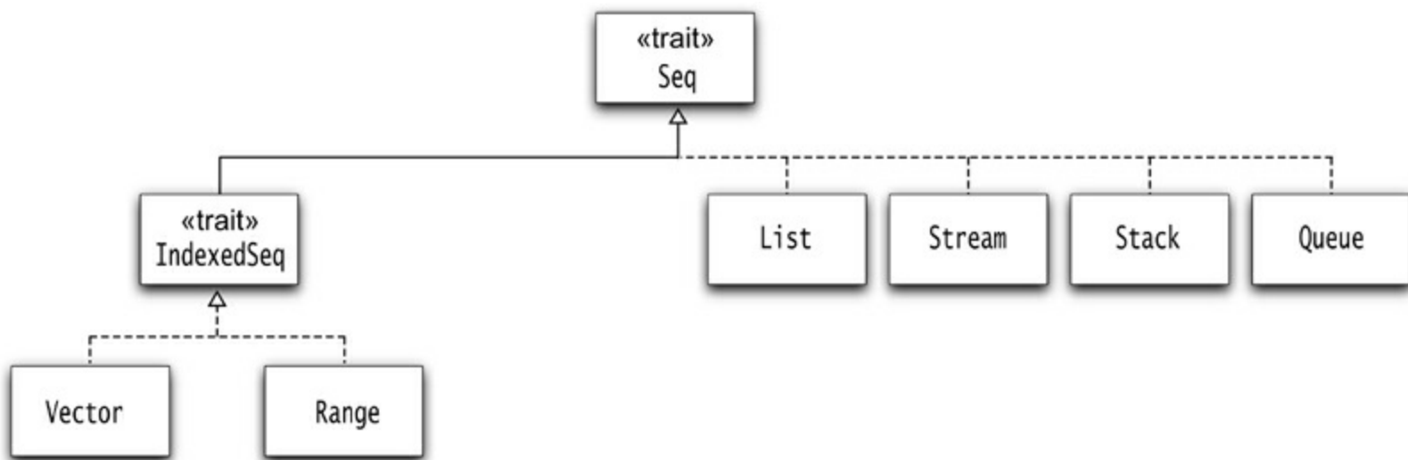
Figure 13–2 Immutable sequences
