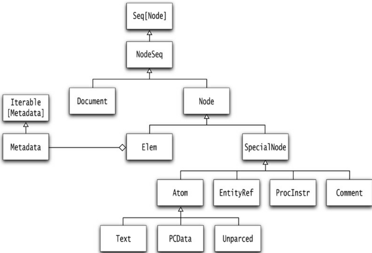
Figure 16–1 XML node types
