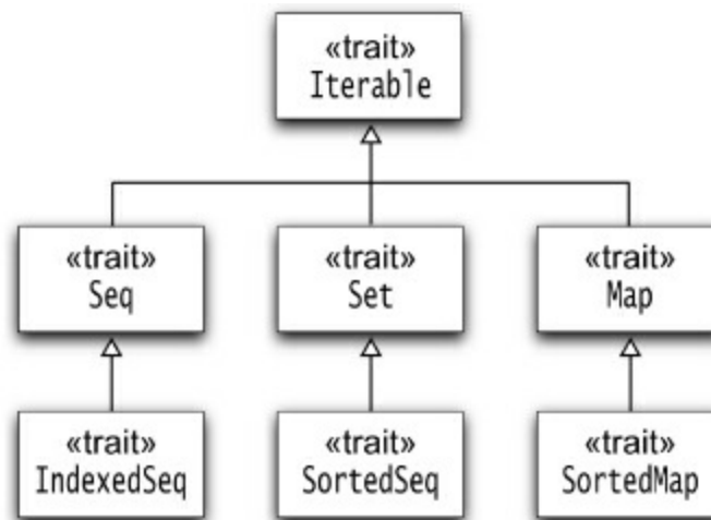
Figure 13–1 Key traits in the Scala collections hierarchy
