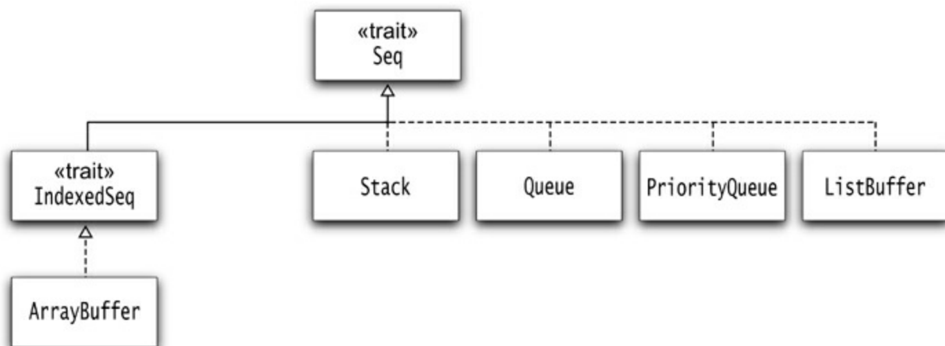
Figure 13–3 Mutable sequences
