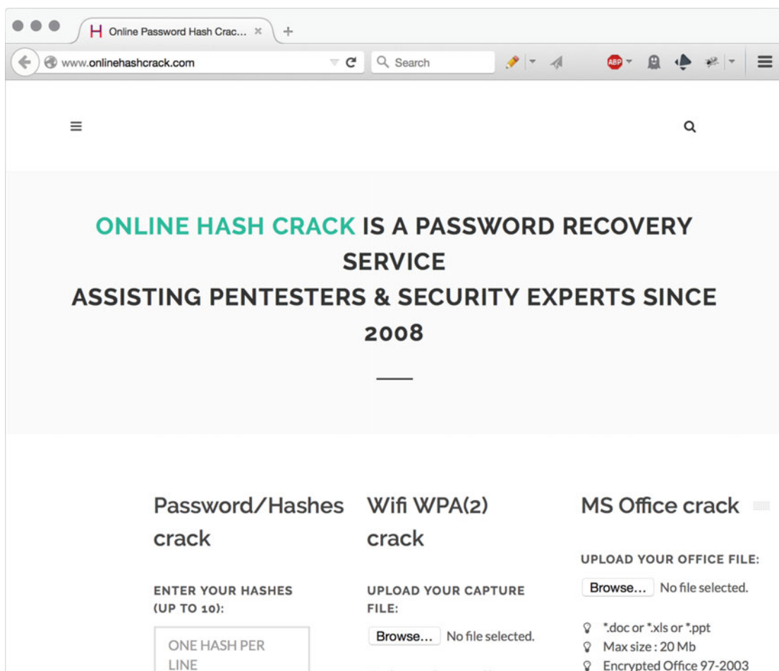
Figure 7-7. Onlinehashcrack.com
