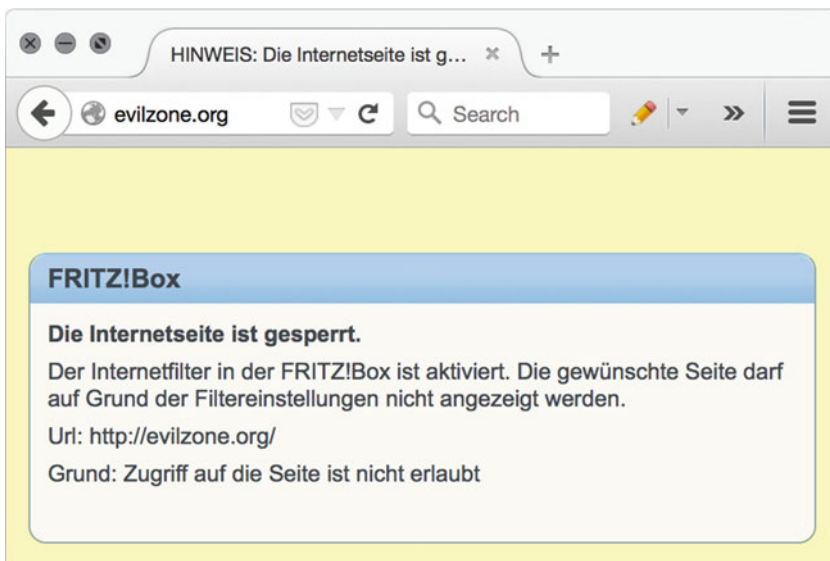
Figure 4-6. Blocked site
