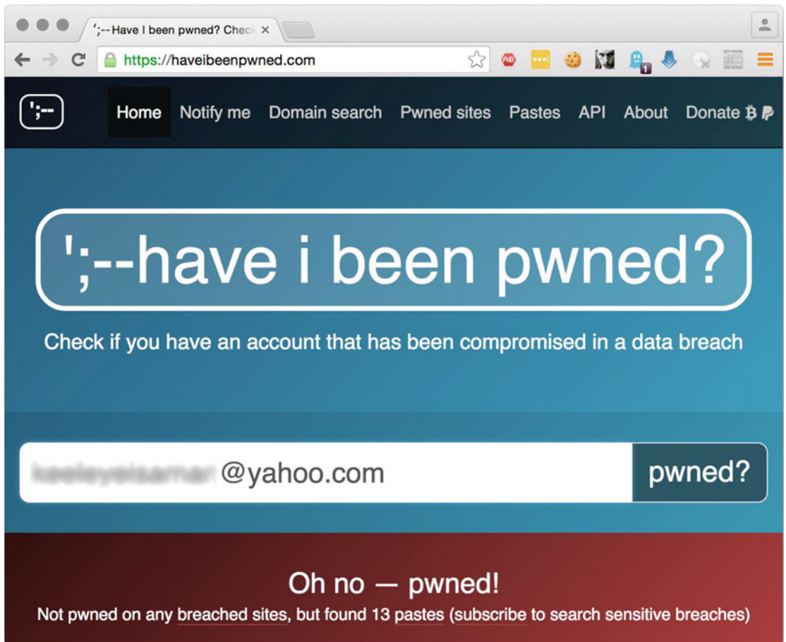
Figure 6-7. Haveibeenpwned.com
