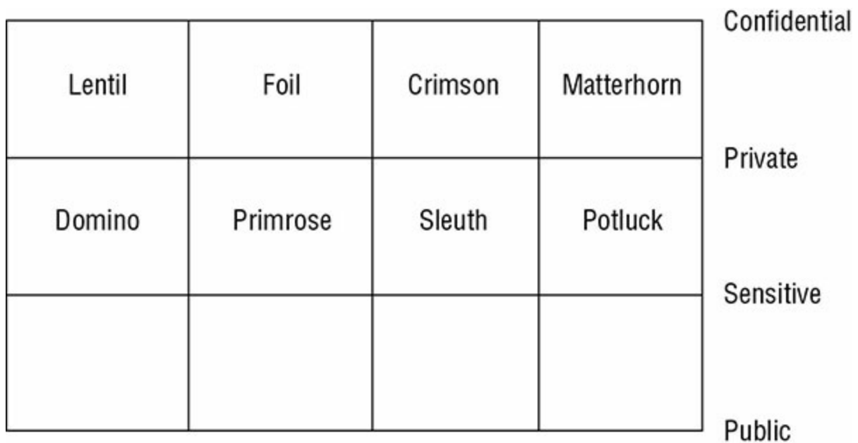
FIGURE 14.3 A representation of the boundaries provided by lattice-
