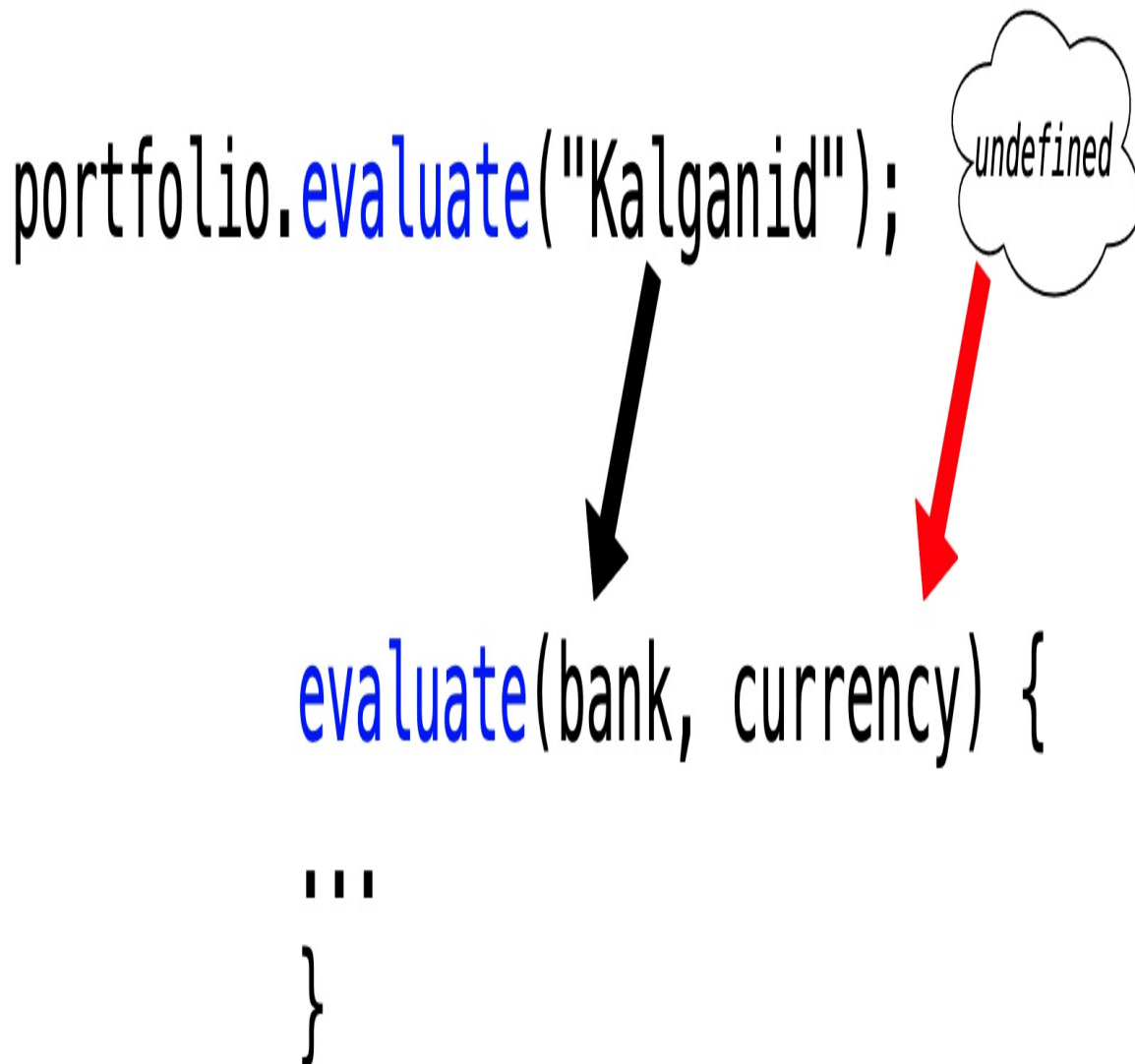
Figure 11-2. In JavaScript, any missing parameters in a method call are left as undefined
