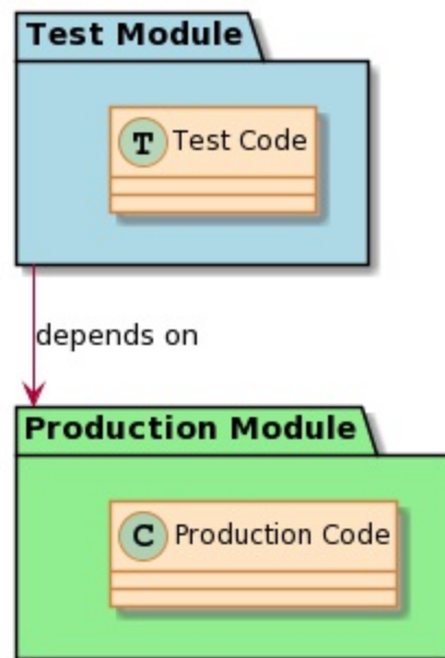
Figure 4-4. Only Test Code should depend on Production Code, not the other way around
