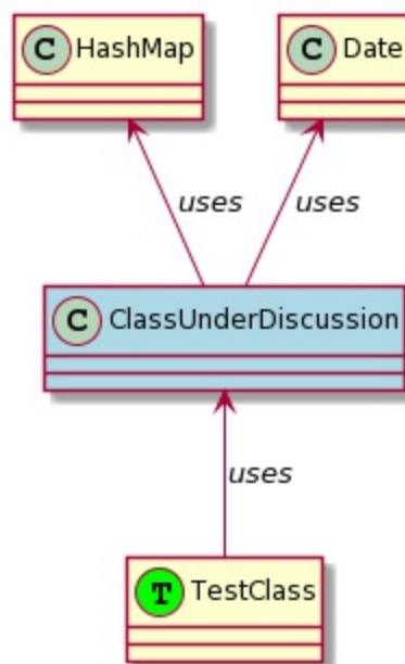
Figure 14-1. Afferent and efferent coupling
