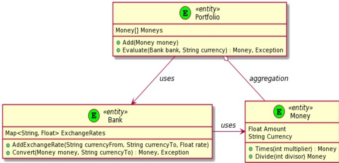
Figure 11-1. The three main entities in our program
