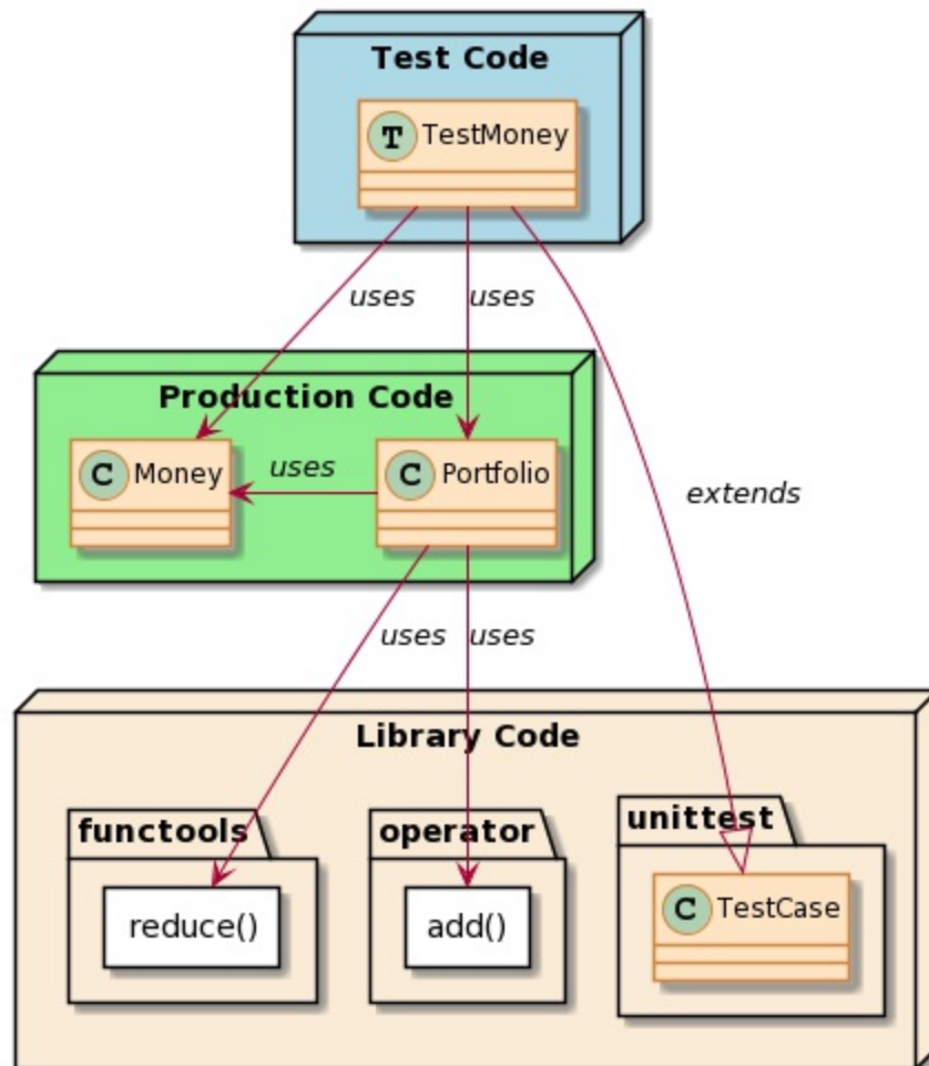
Figure 7-1. The dependency diagram of our Python code after separating it into three source files
