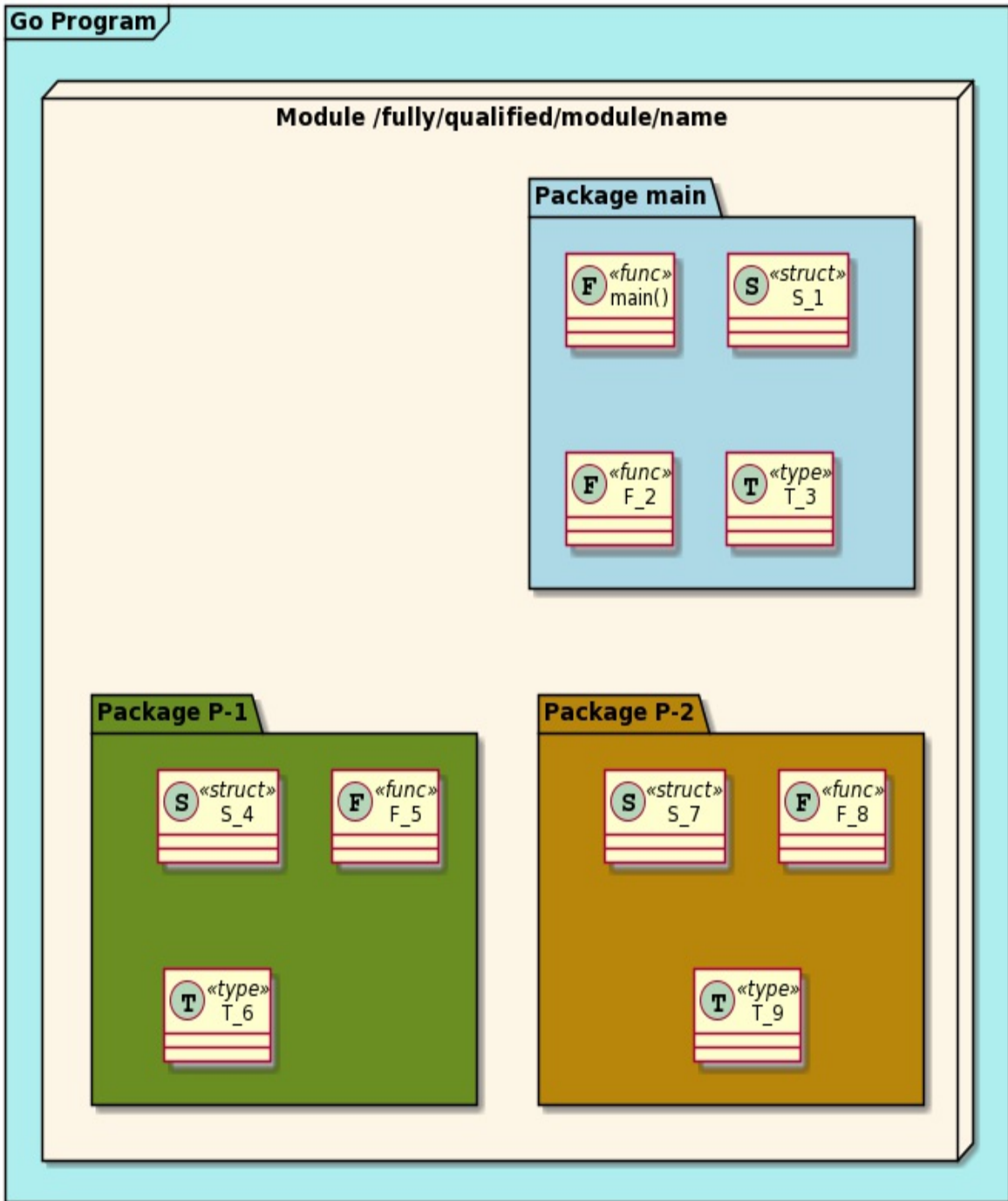
Figure 5-1. Structure of a typical Go program, showing the hierarchy of program module, packages, and files
