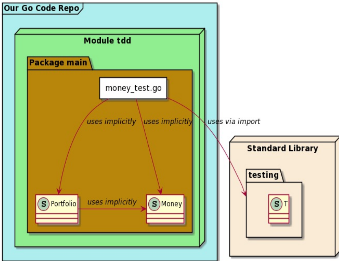
Figure 5-2. The test and production code are in the main package, therefore, the dependencies among them are implicit and do not require import statements
