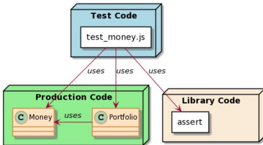
Figure 6-1. The dependency diagram of our JavaScript code after separating it into three source files
