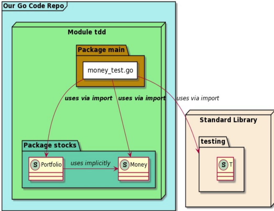
Figure 5-3. The production code is now in its own package, therefore, the dependency from test code to it is explicitly declared
