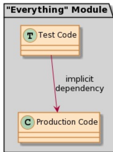
Figure 4-1. When test code and production code are in the same module, the dependency from the former to the latter is implicit
