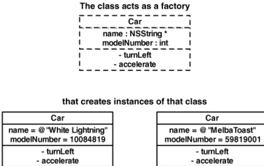
Figure 2.1. A class and its instances
