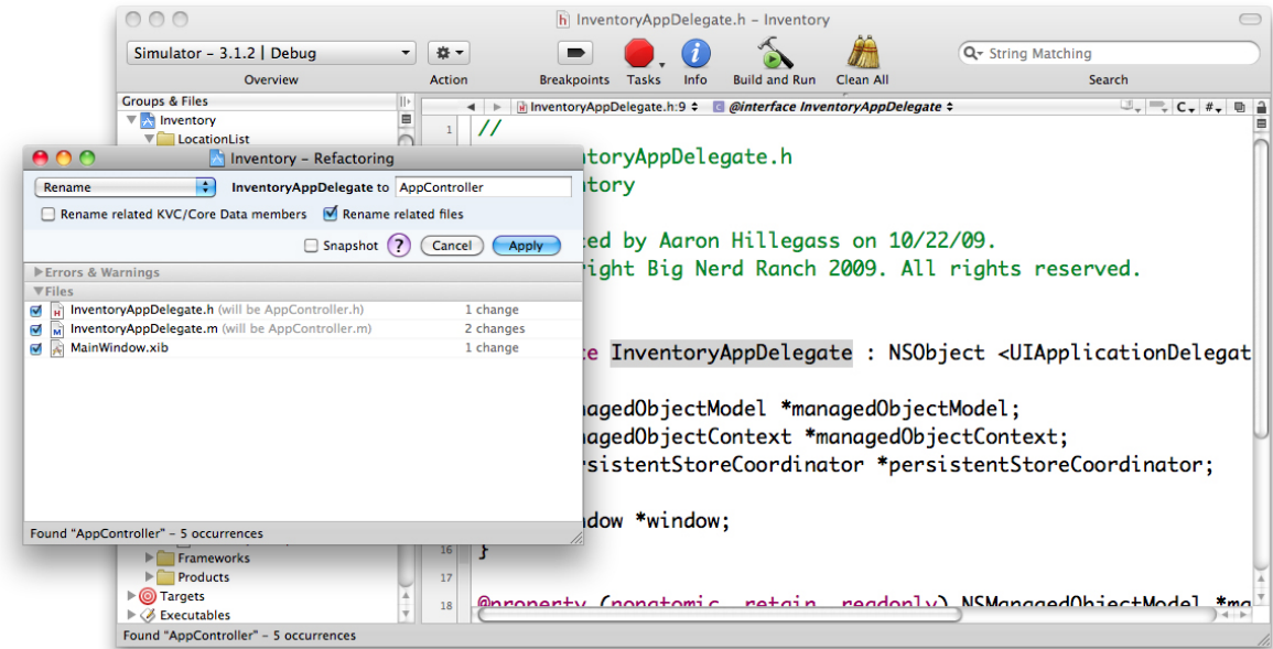
Figure 27.11. Renaming InventoryAppDelegate
