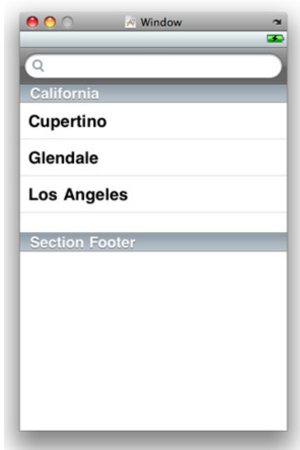
Figure 26.3. Layout
