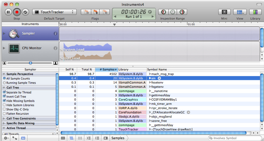
Figure 17.9. Sampler
