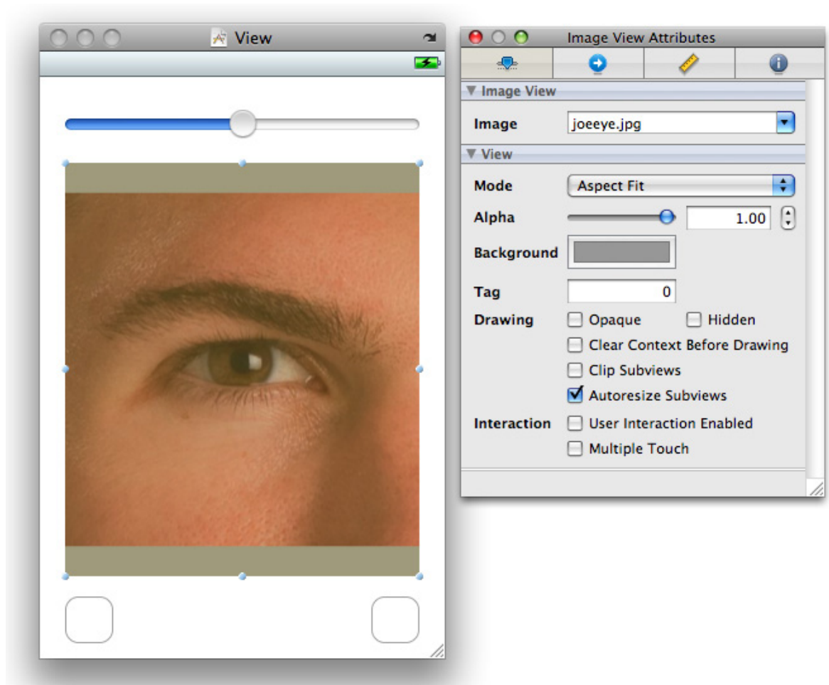
Figure 9.1. UIImageView
