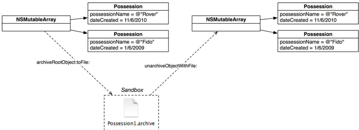
Figure 14.4. Archived object
