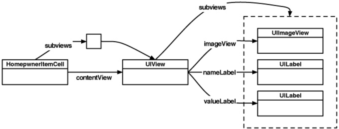
Figure 16.3. HomepwnerItemCell hierarchy
