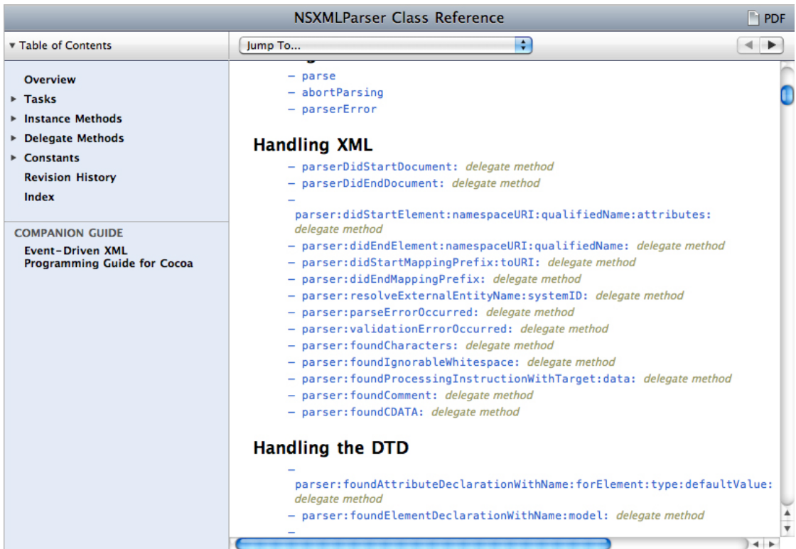
Figure 4.7. NSXMLParser Documentation
