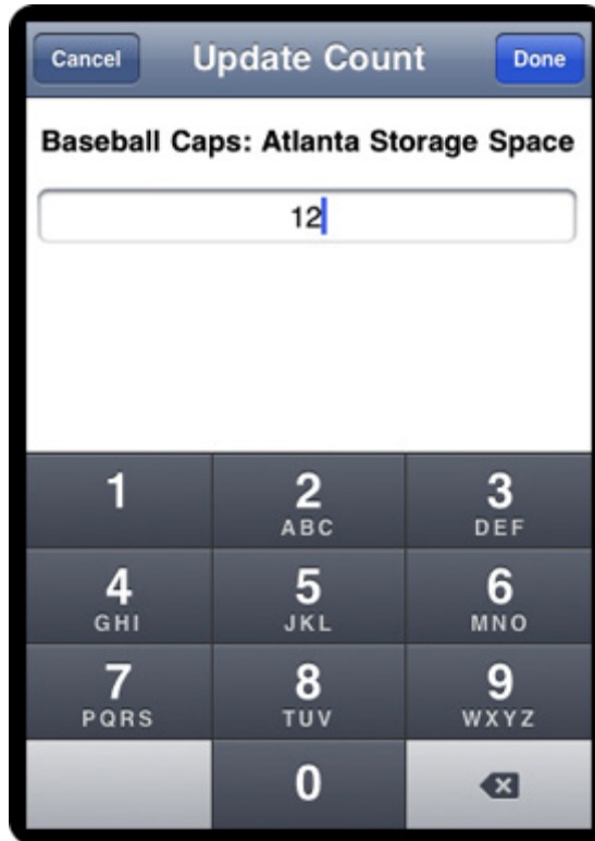
Figure 27.17. CountViewController
