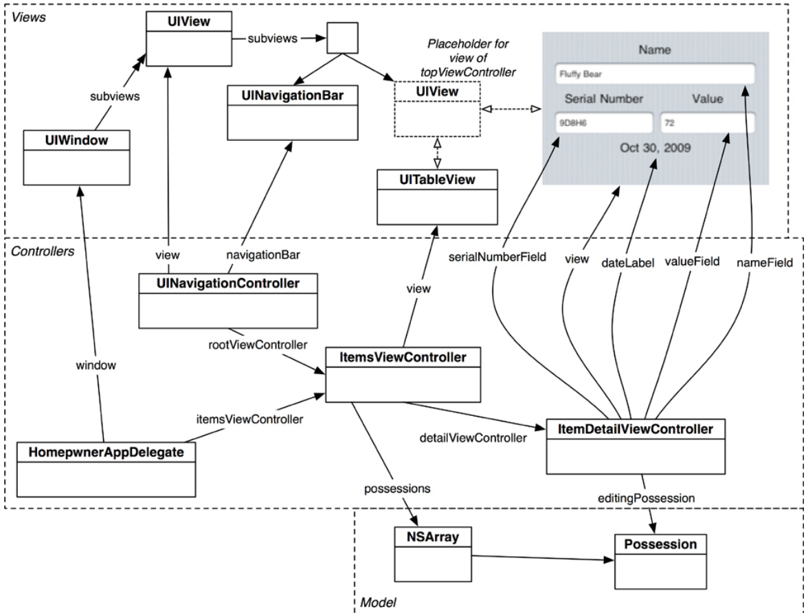
Figure 12.4. Homepwner object diagram
