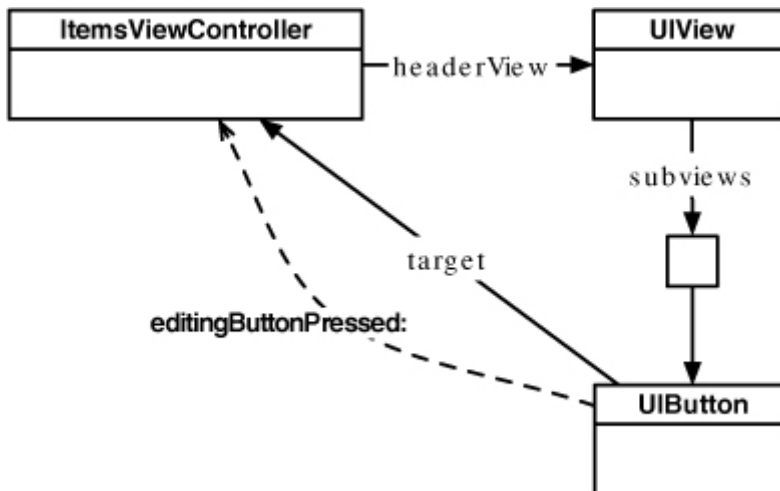
Figure 11.3. Target-Action pair
