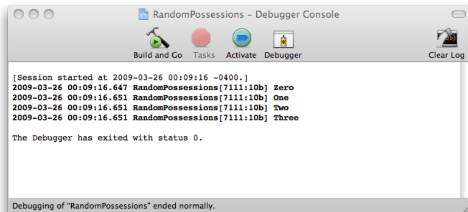
Figure 2.5. Console output
