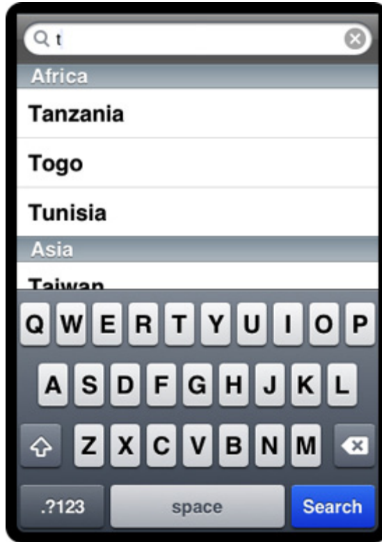
Figure 26.1. Nayshunz
