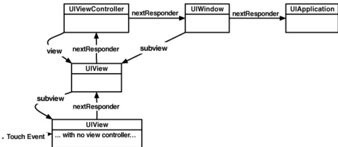
Figure 17.4. Responder chain
