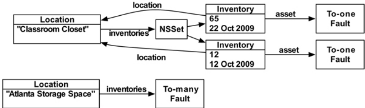
Figure 27.20. Faults, part 2
