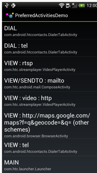
Figure 400: Preferred Activities on a Stock HTC One S
