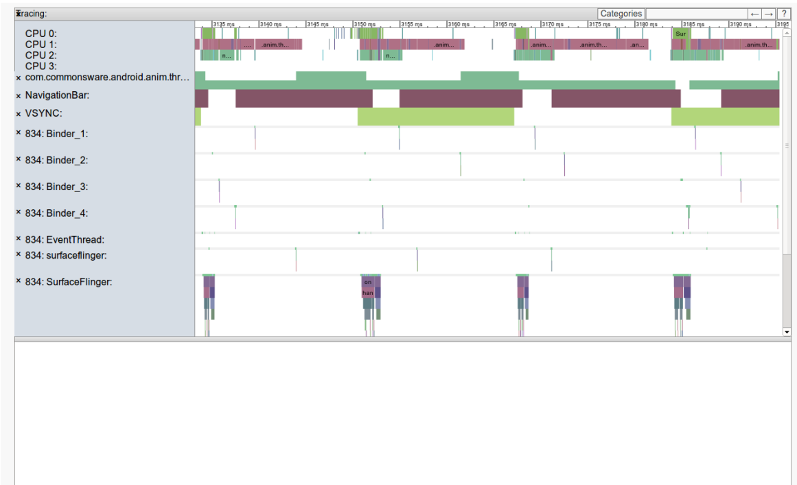
Figure 475: Systrace Output, Zoomed In, Showing 3135ms to 3190ms
