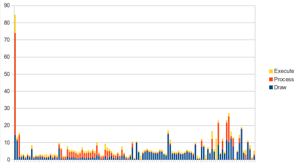
Figure 470: gfxinfo Output, In Stacked Column Chart
