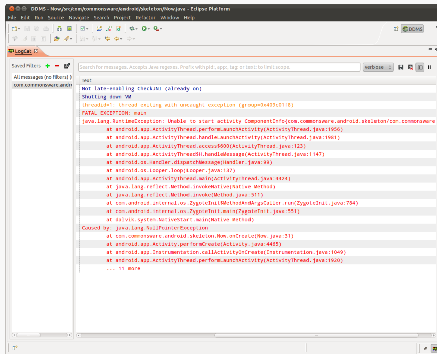
Figure 72: Eclipse Window with LogCat View Scrolled Right
