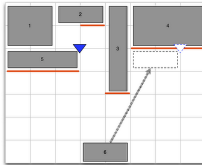
Figure 224: Span Sample (image courtesy of Android Open Source Project)
