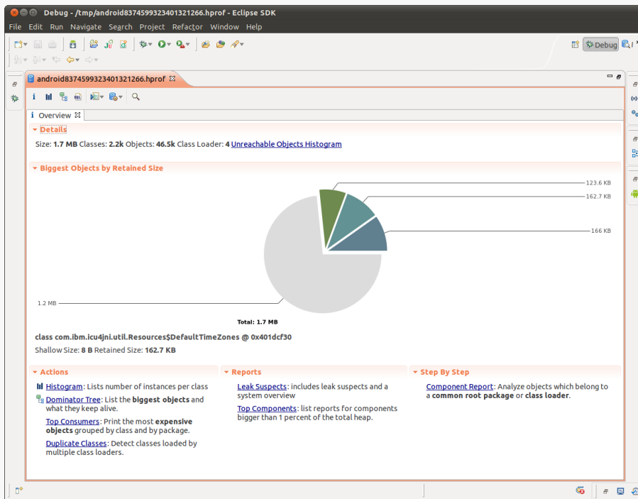
Figure 493: The Overview tool inside the MAT Eclipse perspective
