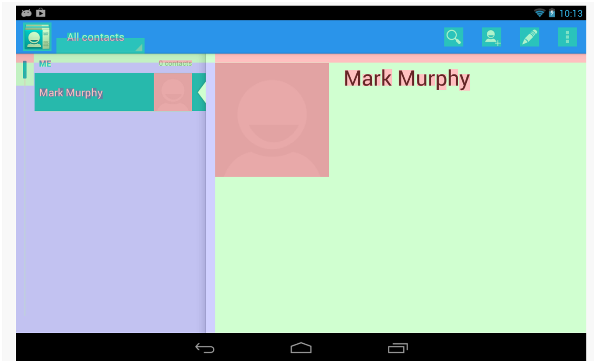
Figure 483: Contacts App, Showing Overdraw
