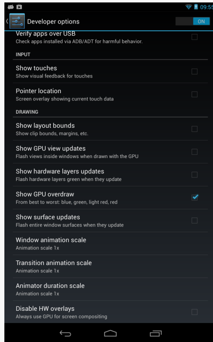
Figure 478: Nexus 7 Developer Options, with “Show GPU overdraw”
