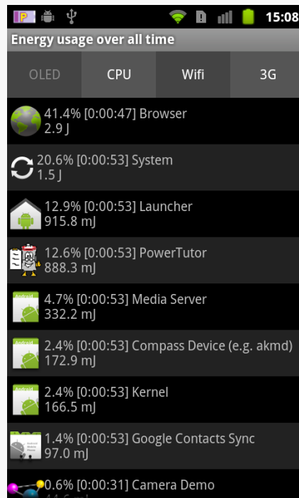
Figure 510: The PowerTutor application roster
