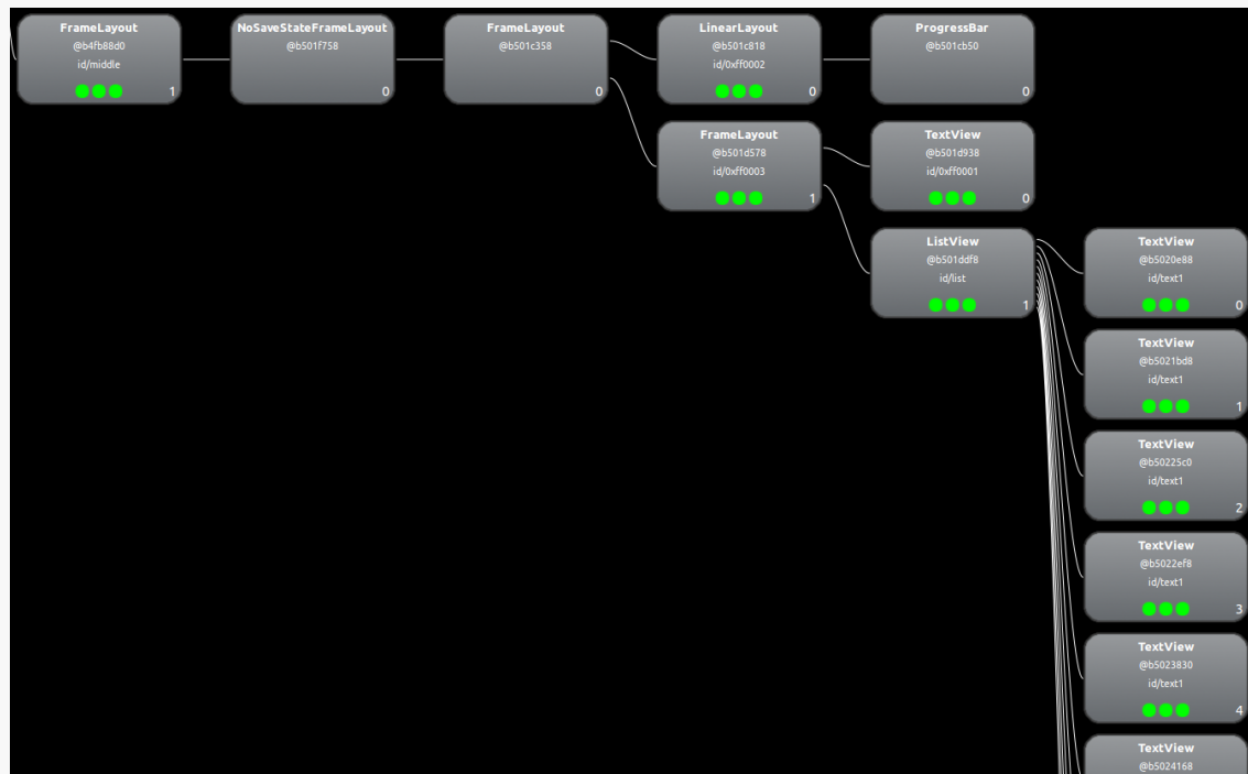
Figure 486: Contents of a ListFragment, from Hierarchy View
