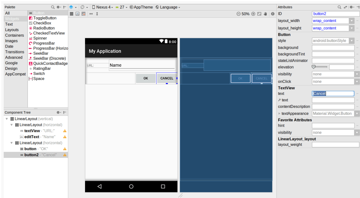
Figure 125: Buttons with Desired Captions
