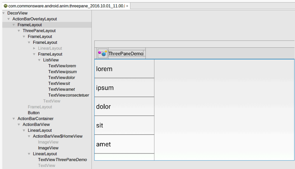
Figure 973: Three-Pane Demo in Layout Inspector, Showing More Hierarchy
