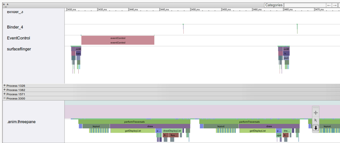
Figure 962: Systrace Output, Zoomed In on 40 Milliseconds of Profiling
