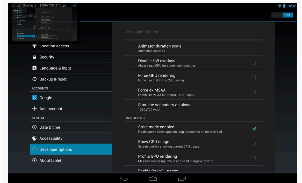
Figure 804: Nexus 10, Simulating a 720p external display
