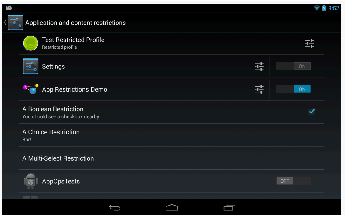
Figure 735: Restricted Profile, Showing App Restrictions
