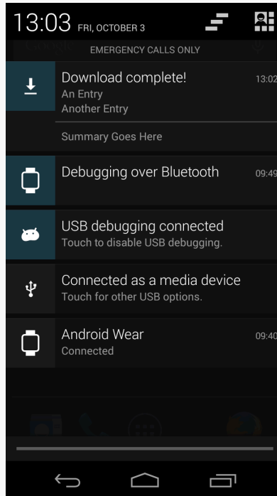
Figure 384: Stacked Notifications, Summary on Primary Device
