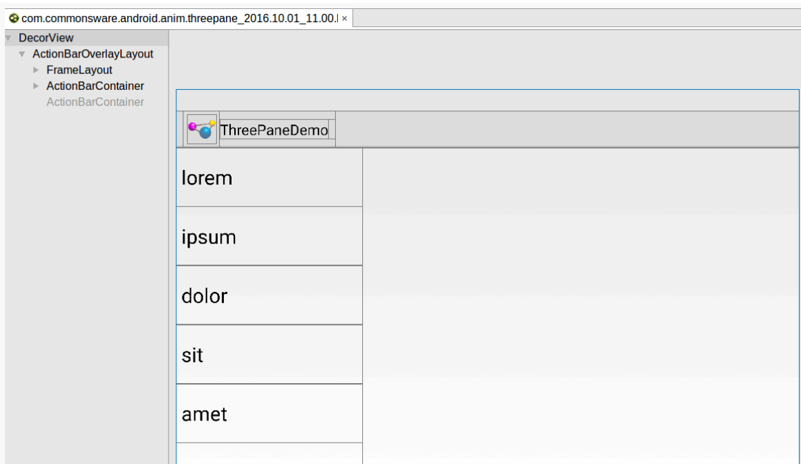
Figure 972: Three-Pane Demo, As Initially Launched, in Layout Inspector
