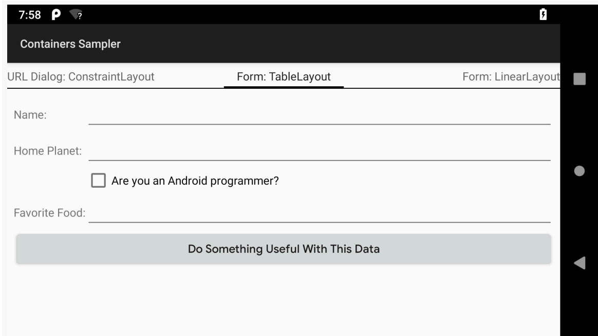
Figure 137: Form Layout, Using TableLayout
