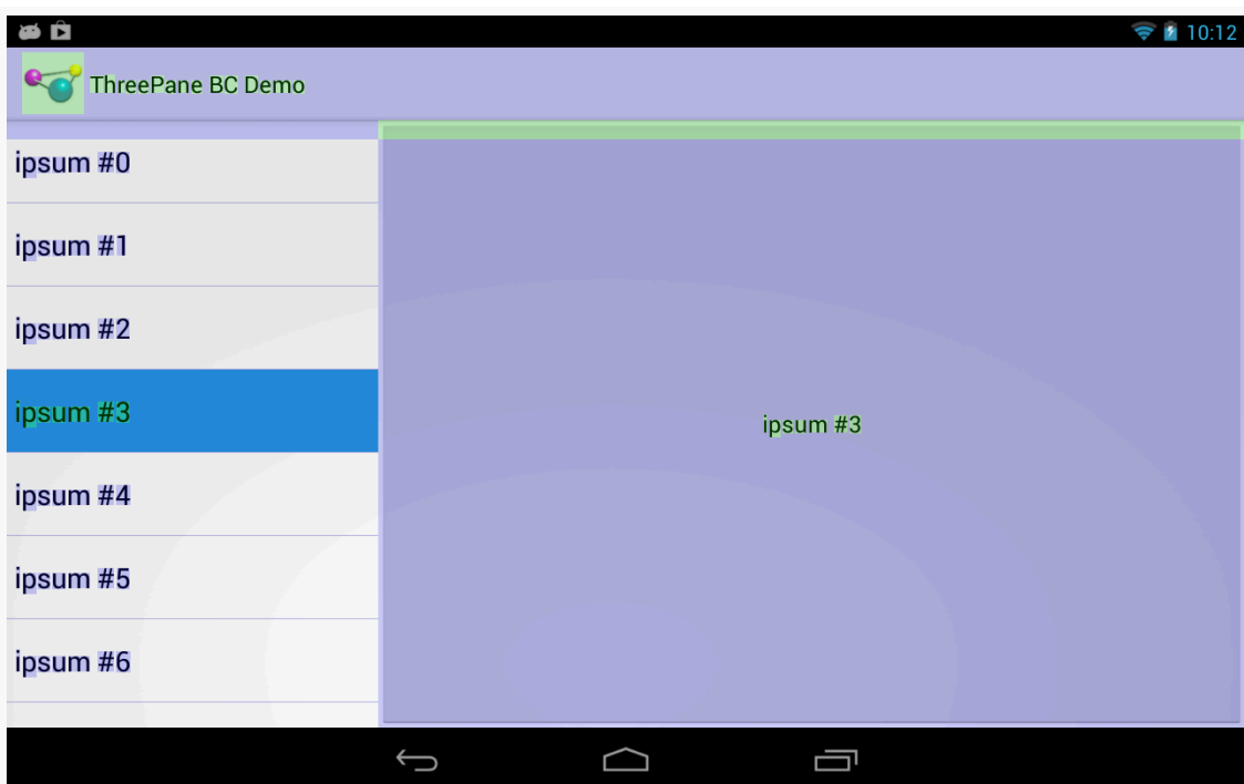
Figure 969: Three-Pane Demo, Middle and Right Panes, Showing Overdraw
