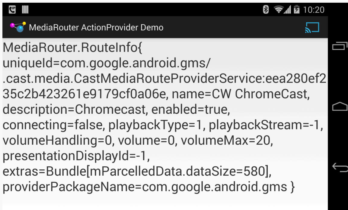
Figure 795: MediaRouter ActionProvider Demo, on a Nexus 4, Showing Selected Chromecast Route
