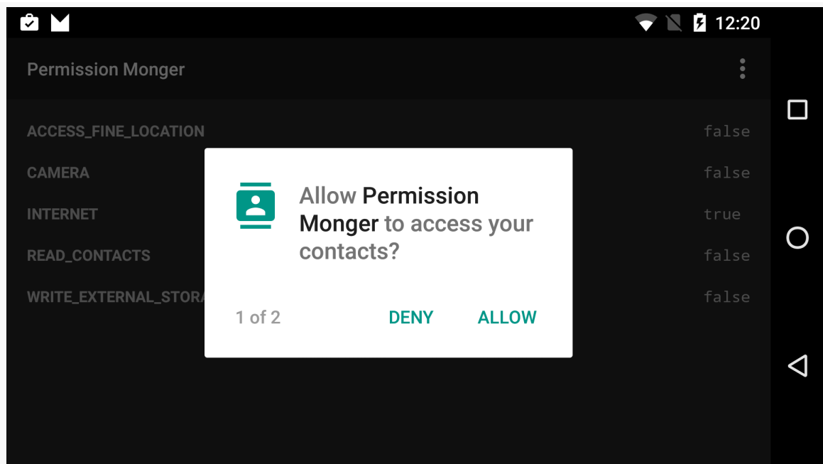
Figure 747: Runtime Permission System Dialog
