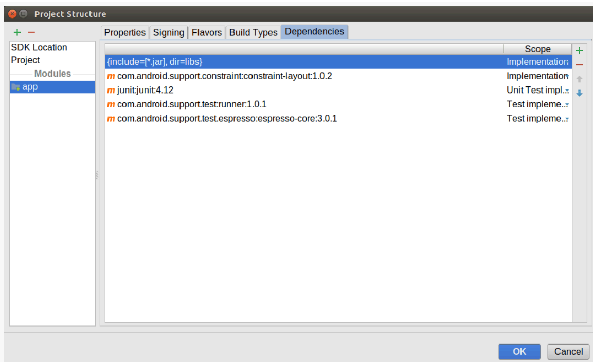
Figure 890: Project Structure Dialog, Module Category, Dependencies Tab
