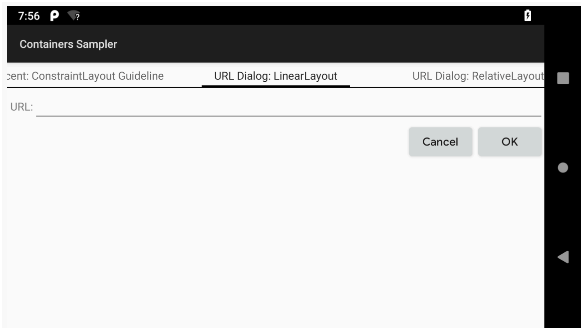
Figure 116: URL-Dialog Layout, Using LinearLayout
