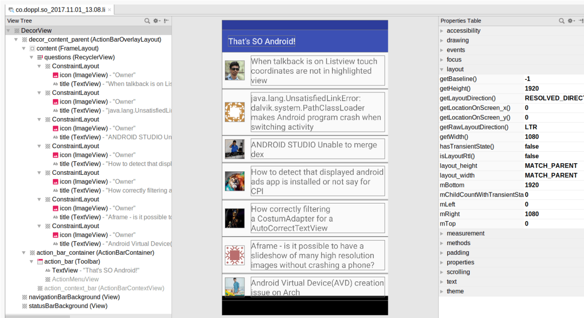
Figure 924: Layout Inspector, As Initially Launched
