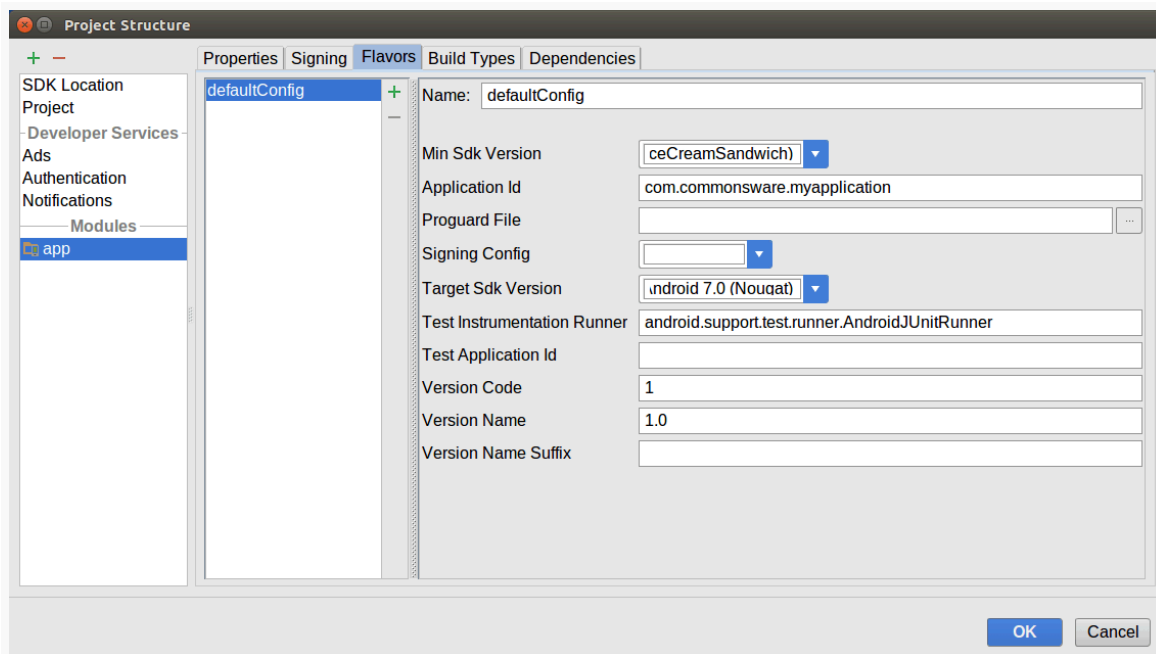
Figure 888: Project Structure Dialog, Module Category, Flavors Tab
