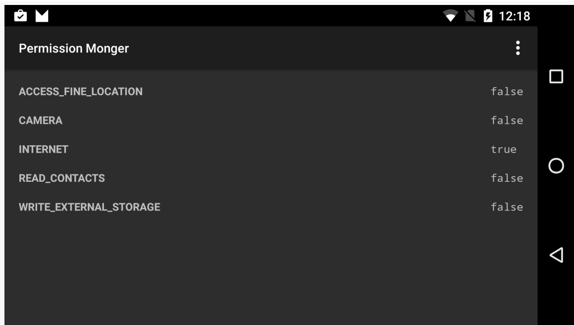
Figure 259: Permission Monger, Showing Initial Permissions
