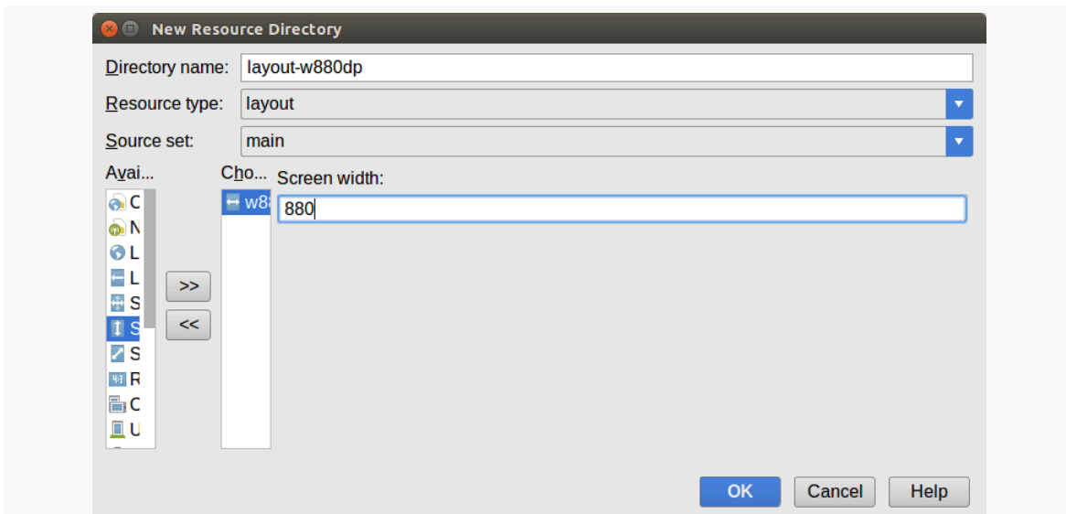
Figure 309: Android Studio New Resource Dialog, After Setting Screen Width
