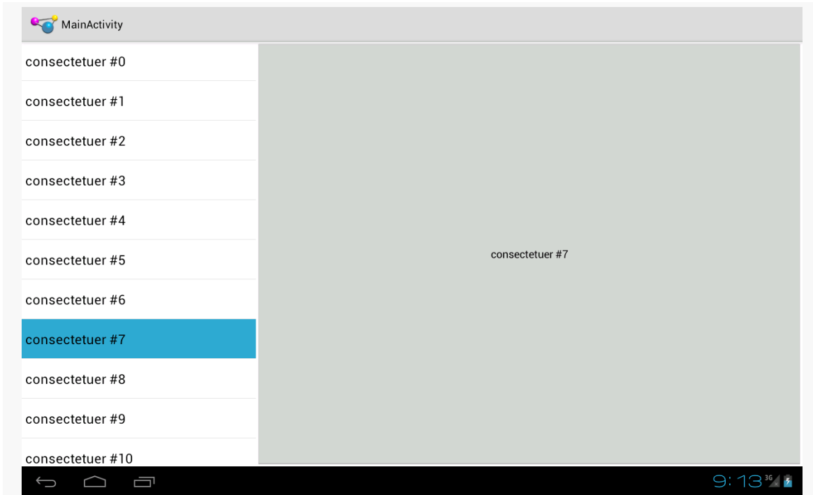
Figure 533: ThreePane, After Clicking a Numbered Word
