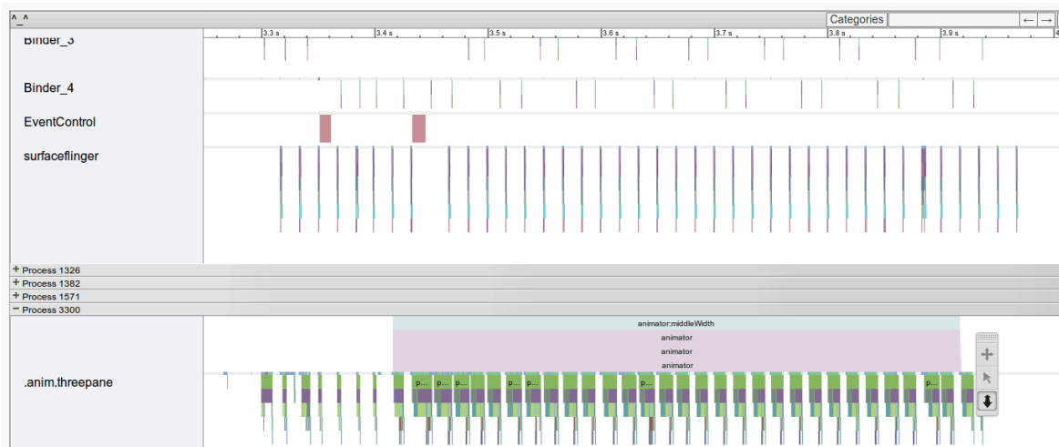
Figure 961: Systrace Output, Zoomed In on 0.7 Seconds of Profiling
