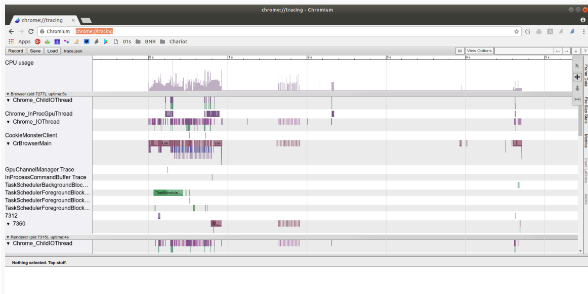
Figure 1095: Chrome Dev Tools, Showing Tracing Results
