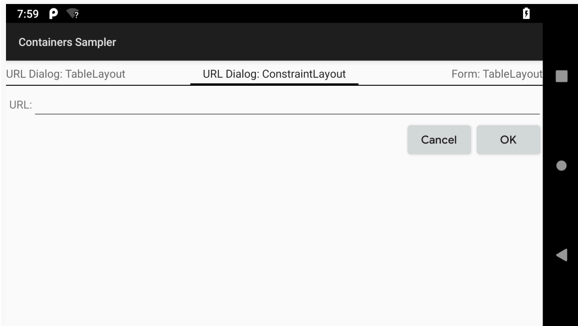
Figure 185: URL Dialog Layout, Using ConstraintLayout
