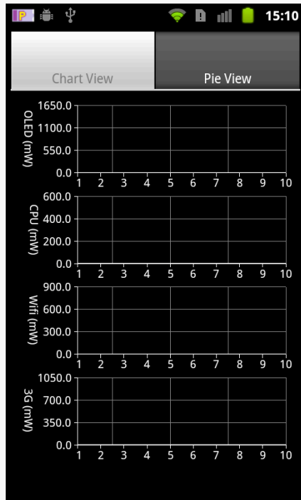
Figure 1018: The PowerTutor live charts for a single process current power consumption
