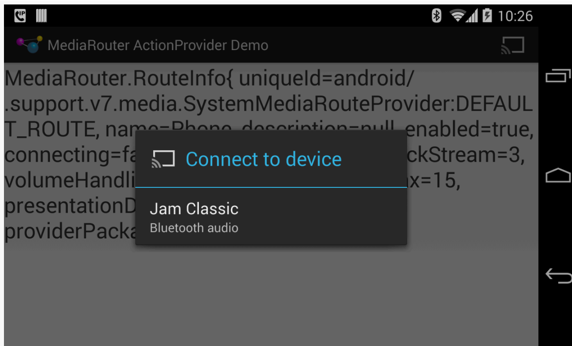
Figure 790: MediaRouter ActionProvider Demo, on a Nexus 4, Showing Available Routes
