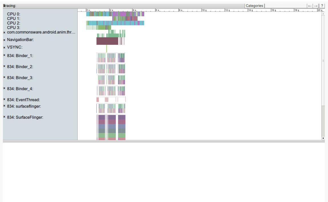
Figure 960: Systrace Output, As Initially Viewed
