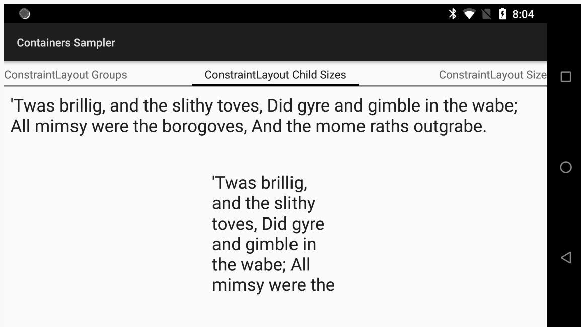
Figure 443: ConstraintLayout, with Constrained Size of Second Child
