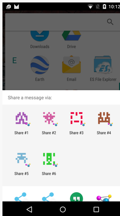
Figure 867: Chooser, Showing Direct-Share Targets
