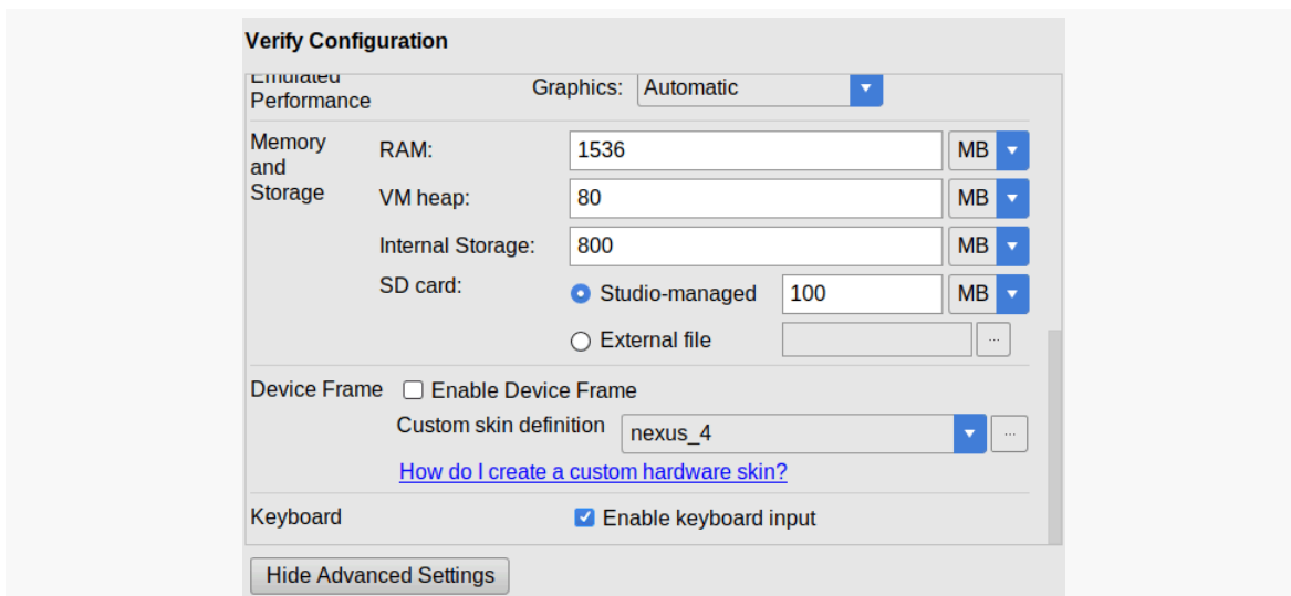
Figure 902: Virtual Device Configuration, Showing “Enable keyboard input” Checkbox
