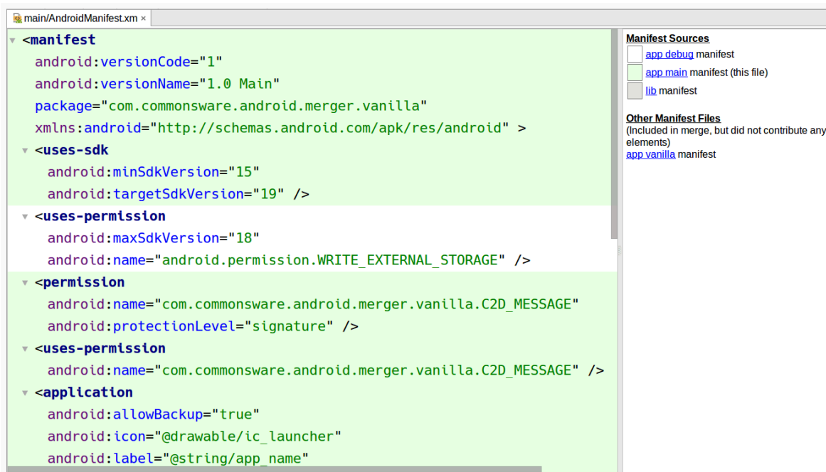
Figure 318: Merged Manifest Tab
