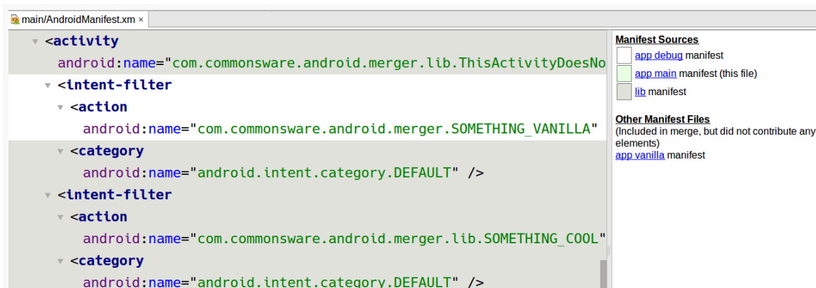
Figure 322: Merged Manifest View, Showing Merged Element
