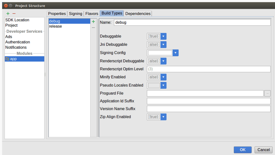
Figure 889: Project Structure Dialog, Module Category, Build Types Tab
