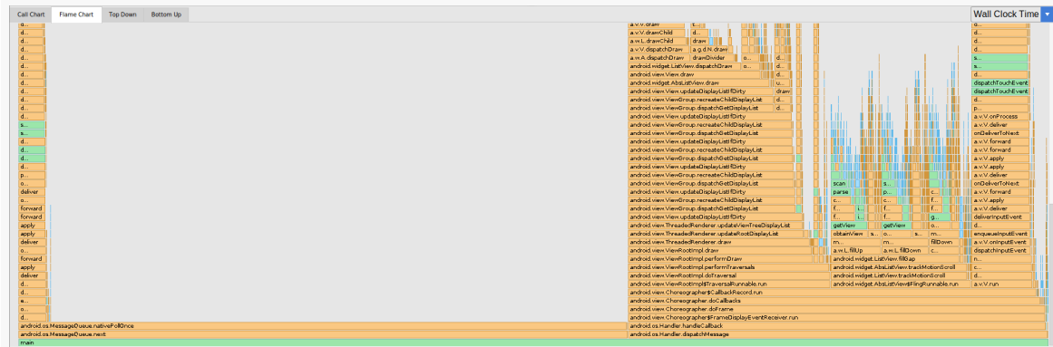
Figure 950: Method Tracing, Flame Chart, As Initially Launched
