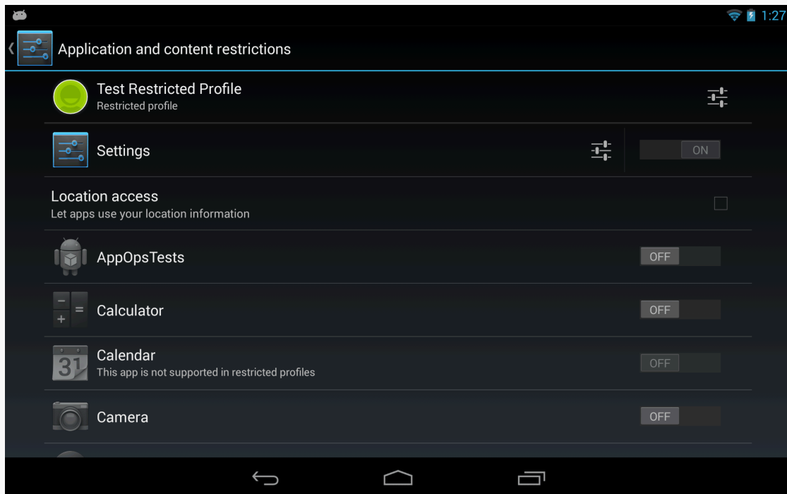
Figure 731: Location Sharing Restrictions
