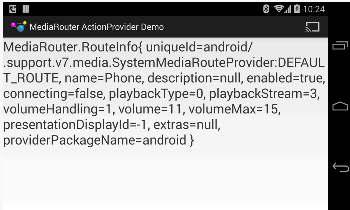
Figure 789: MediaRouter ActionProvider Demo, on a Nexus 4, Showing Default Route and Provider
