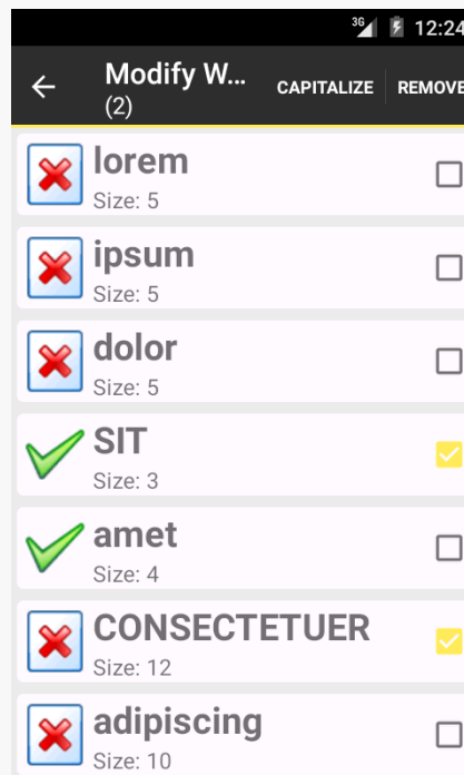
Figure 513: ActionModeList2 RecyclerView Demo, with Capitalized Words
