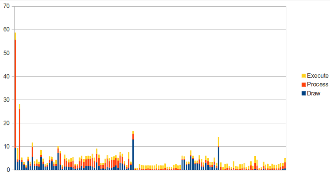
Figure 975: gfxinfo Output of Revised ThreePaneDemoBC
