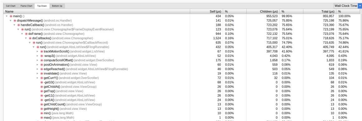
Figure 951: Method Tracing, “Top Down” Table, As Initially Launched
