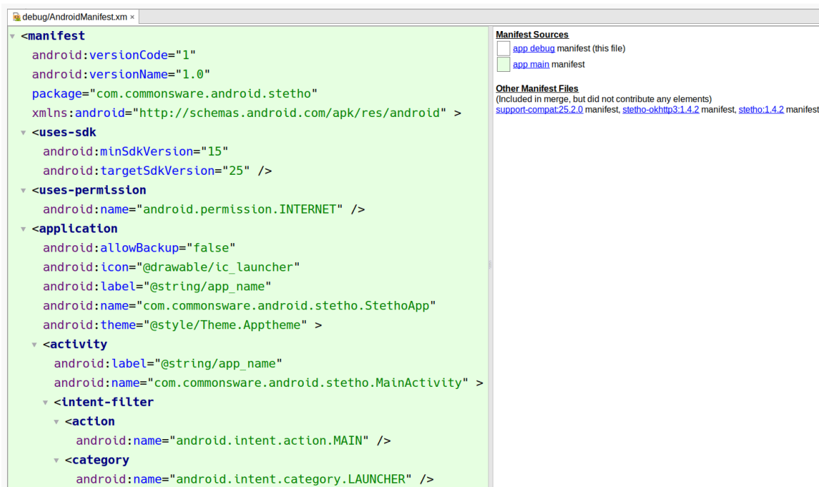
Figure 931: Merged Manifest for Debug Build, Showing StethoApp
