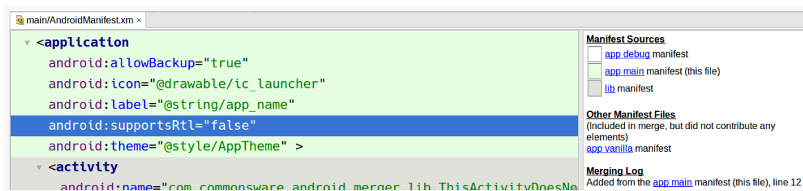
Figure 323: Merged Manifest View, Showing Merged Attribute
