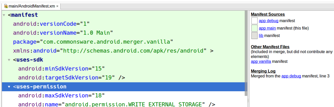
Figure 320: Merged Manifest View, Showing Merged Element
