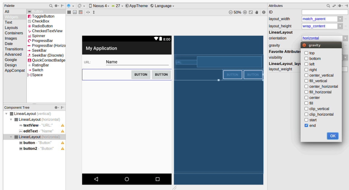
Figure 124: Two Smaller Right-Flush Buttons in Lower Horizontal LinearLayout
