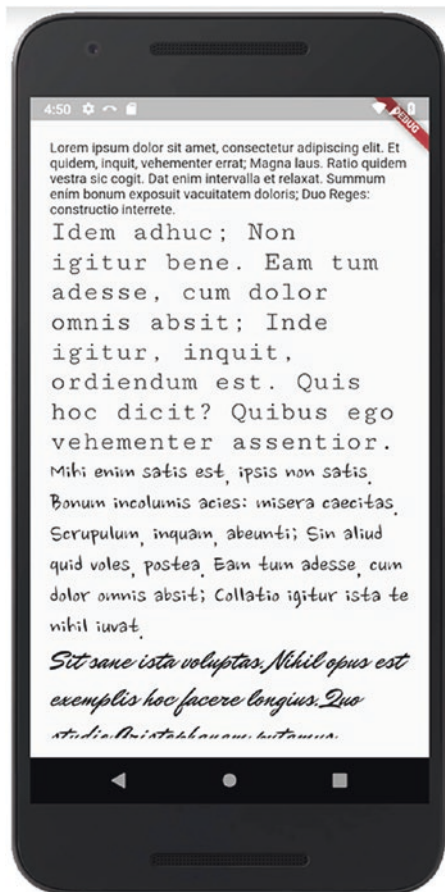
Figure 8-4. Available fonts
