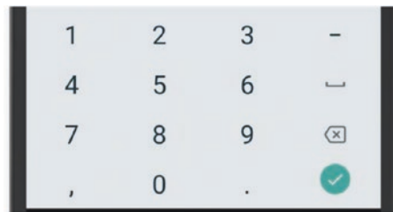
Figure 4-8. TextInputType.number
