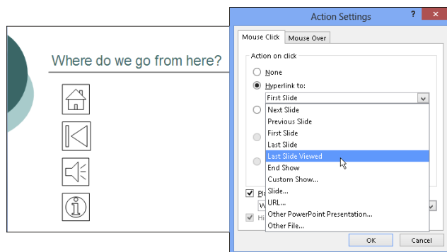
Figure 5-6: Action buttons.
