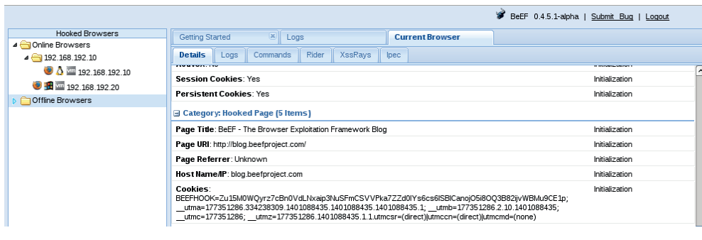
Figure 18-6 The BeEF console showing the hooked target on the blog.beefproject.com page
