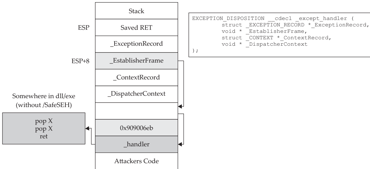
Figure 13-1 The stack when handling an exception
