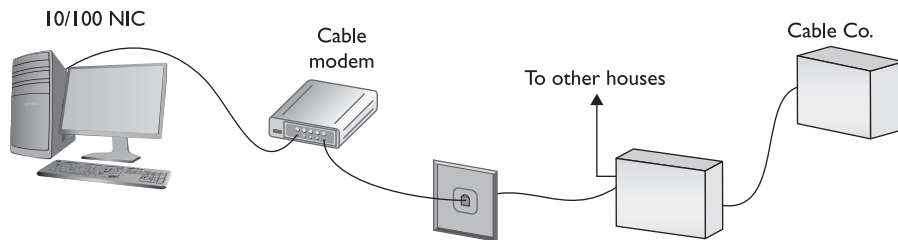
Figure 14-30 Cable modem
