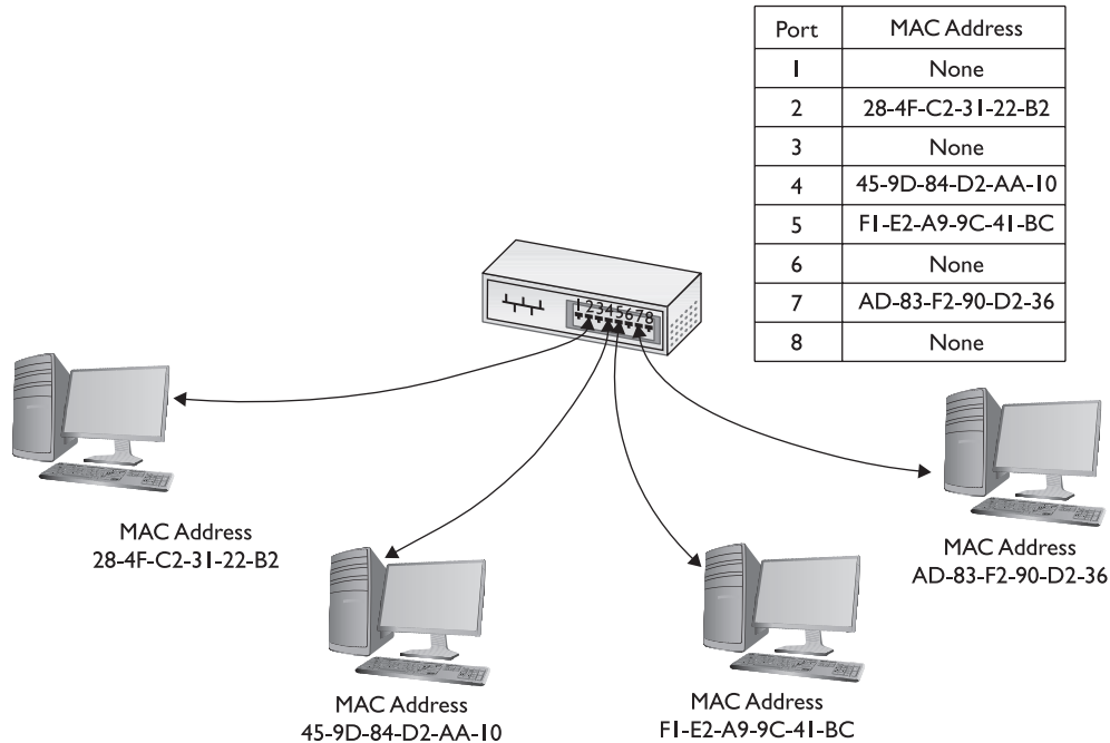
Figure 4-25 A switch tracking MAC addresses
