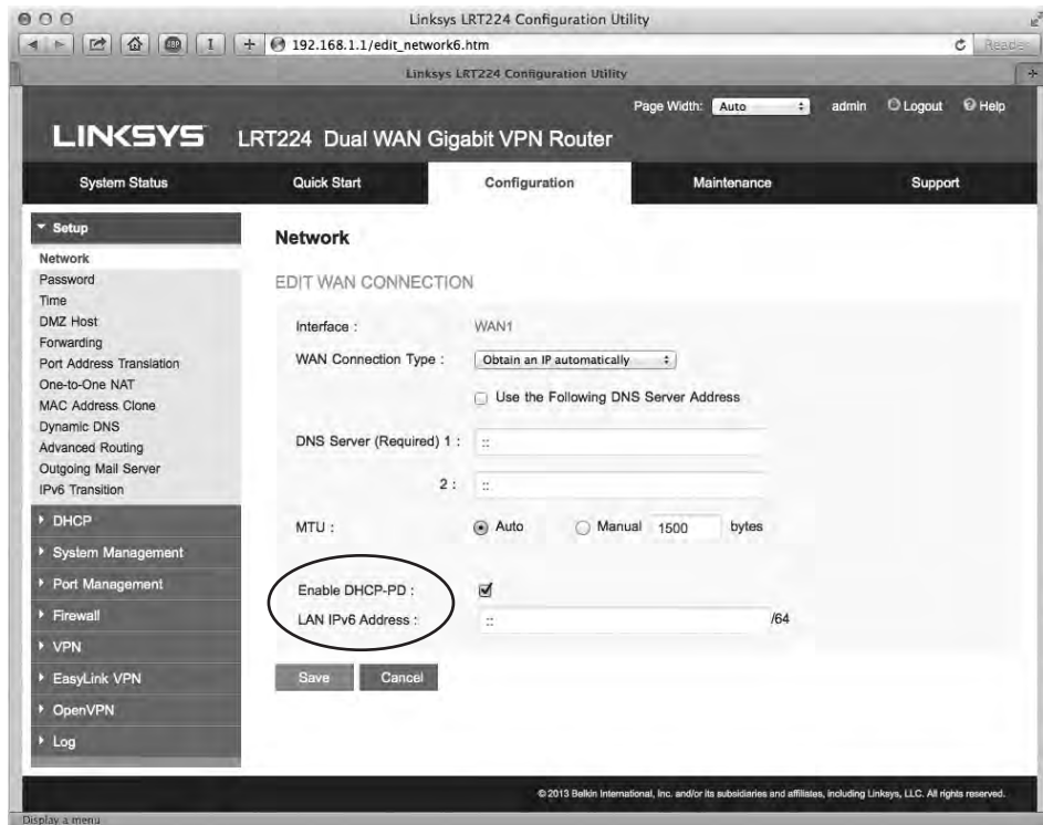
Figure 13-5 Enabling prefix delegation on a SOHO router (called DHCP-PD on this router)
