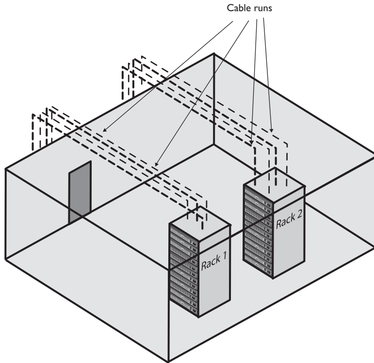
Figure 6-18 Network taking shape, with racks installed and horizontal cabling runs
