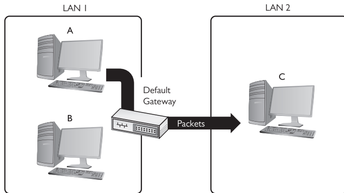
Figure 7-22 Sending a packet remotely
