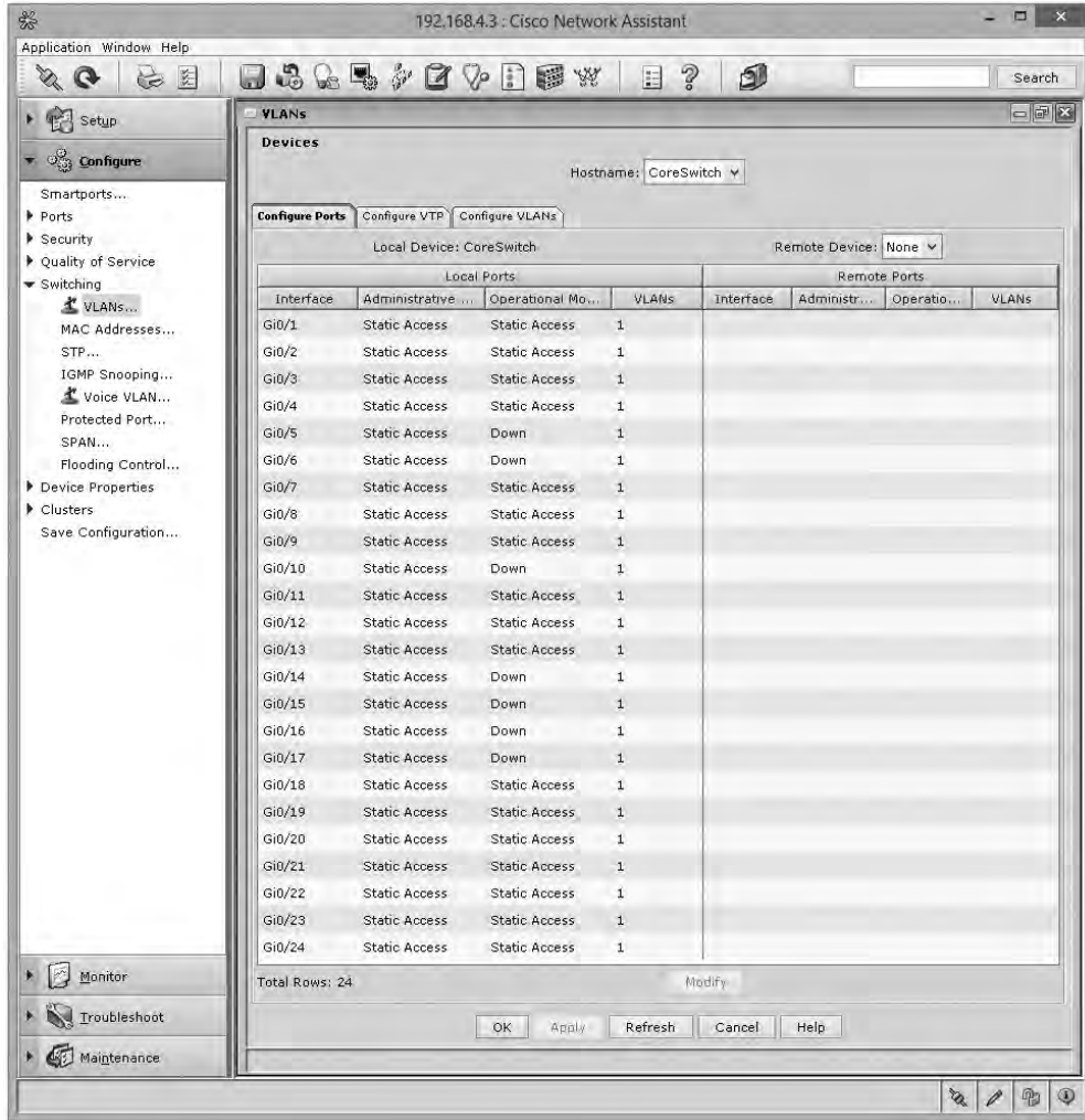
Figure 12-18 Defining VLANs in Cisco Network Assistant
