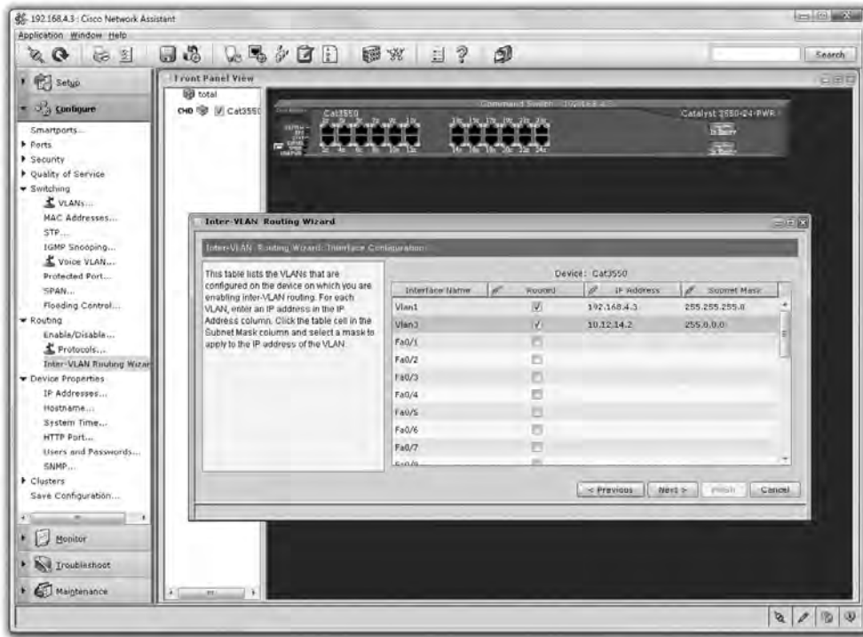
Figure 12-22 Setting up interVLAN routing
