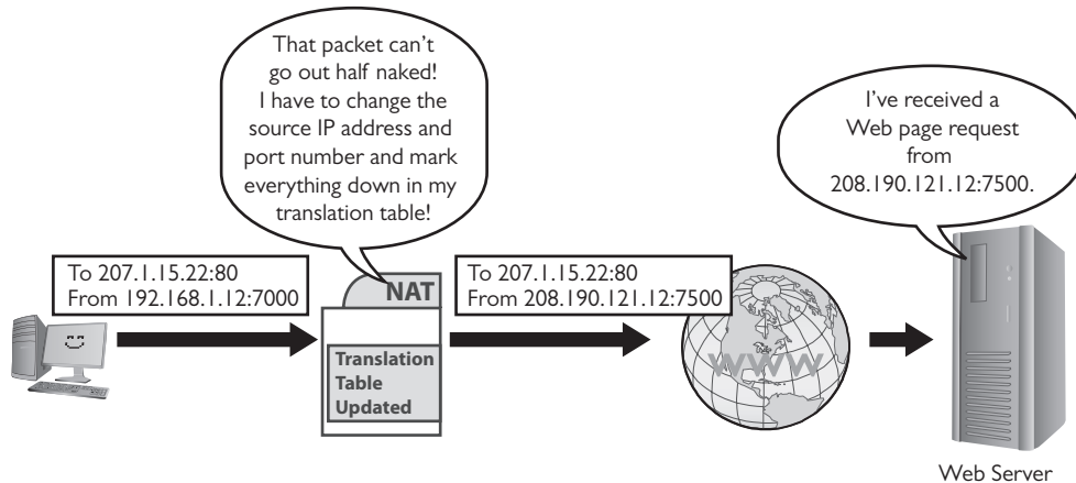
Figure 8-15 PAT in action—changing the source IP address and port number to something usable on the Internet
