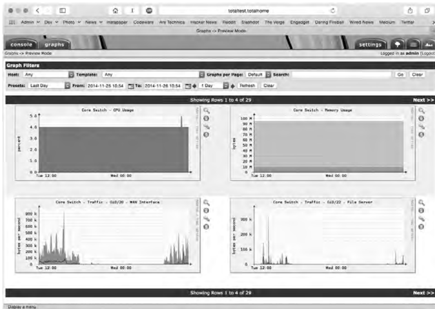
Figure 20-14 Cacti showing switch utilization graphs
