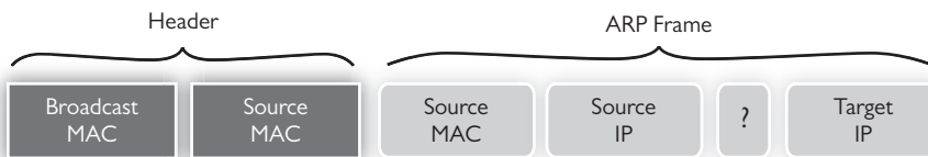
Figure 7-25 Simplified ARP frame
