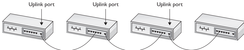
Figure 4-20 Daisy-chained hubs
