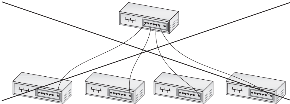
Figure 4-21 A hierarchical hub configuration will not work!
