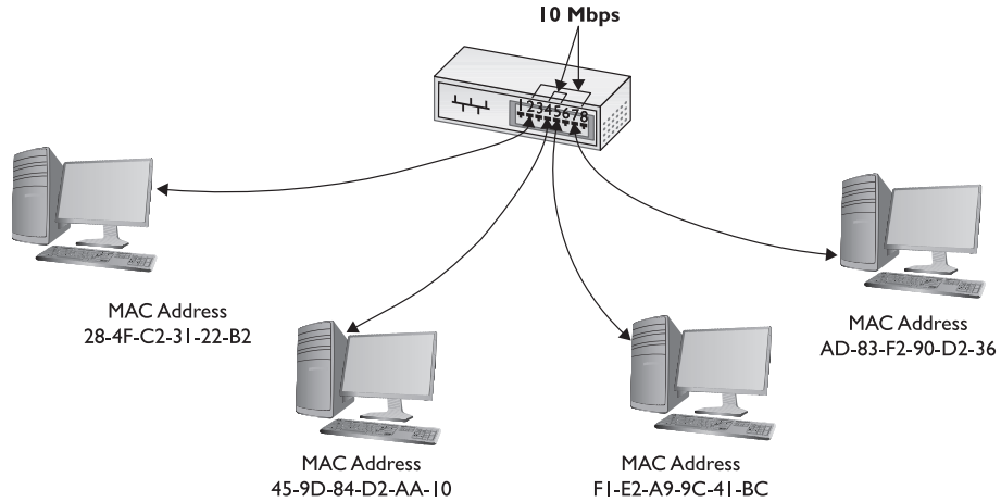
Figure 4-26 A switch making two separate connections
