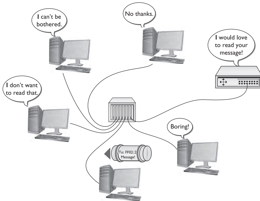
Figure 13-2 Multicast to routers
