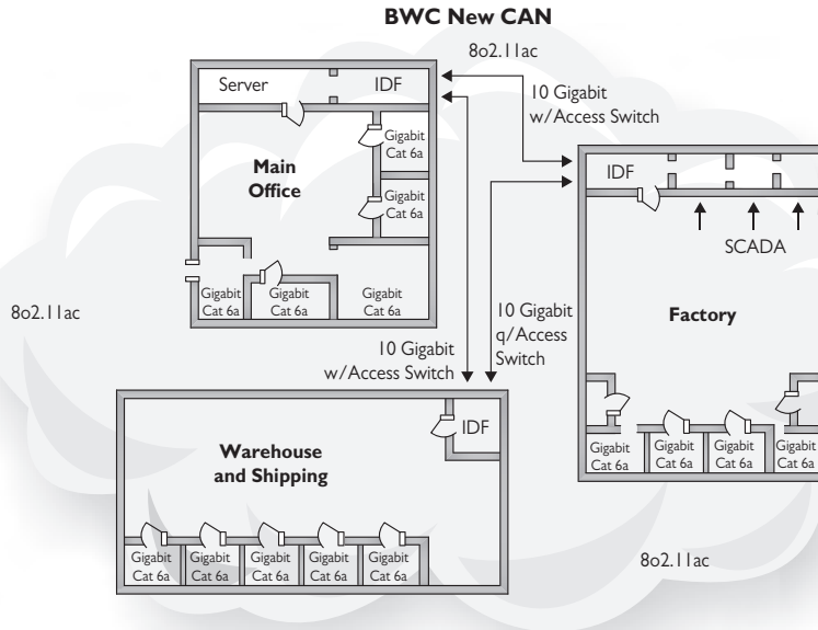
Figure 20-13 Diagram of Bayland Widgets' campus area network
