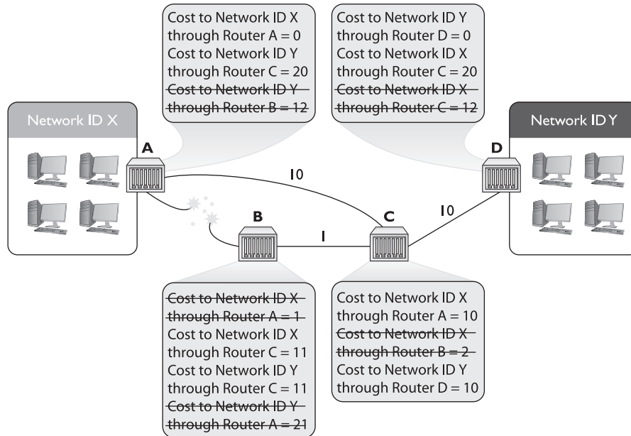
Figure 8-34 Announcing a disconnect
