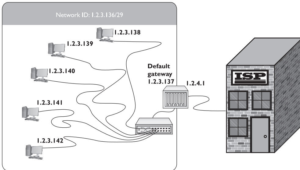
Figure 8-13 Network setup
