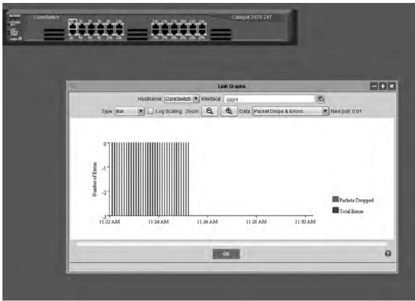
Figure 20-11 Hmm . . . looks pretty clean
