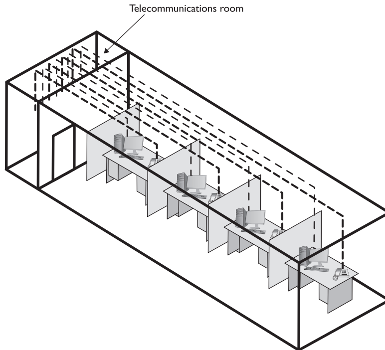
Figure 6-4 Telecommunications room
