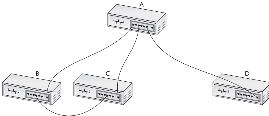
Figure 4-28 A bridging loop
