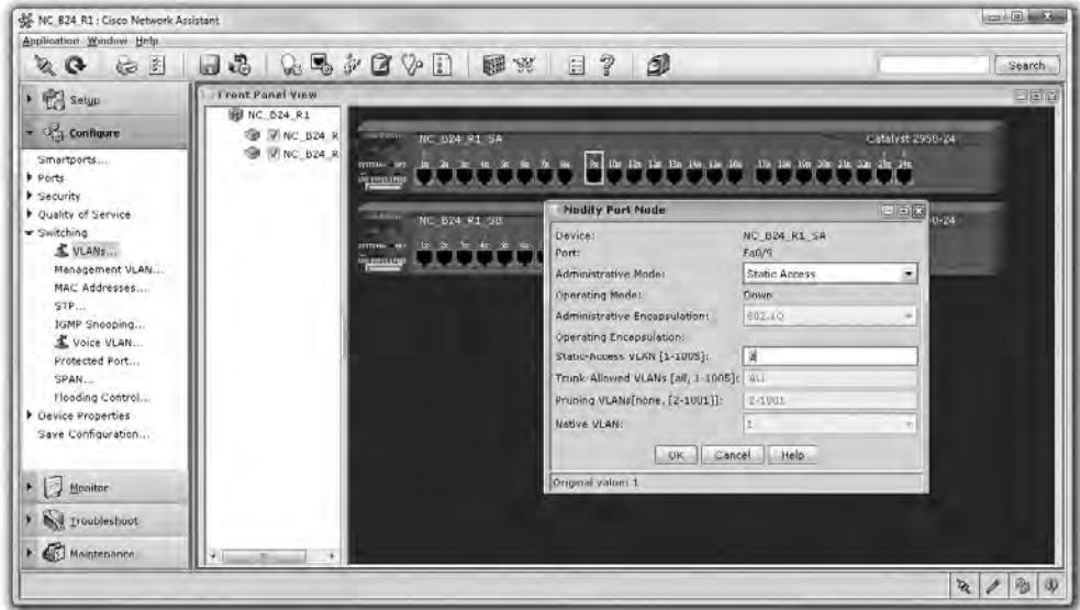
Figure 12-19 Assigning a port to a VLAN
