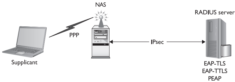
Figure 15-8 Authentication using RADIUS with protocols in place
