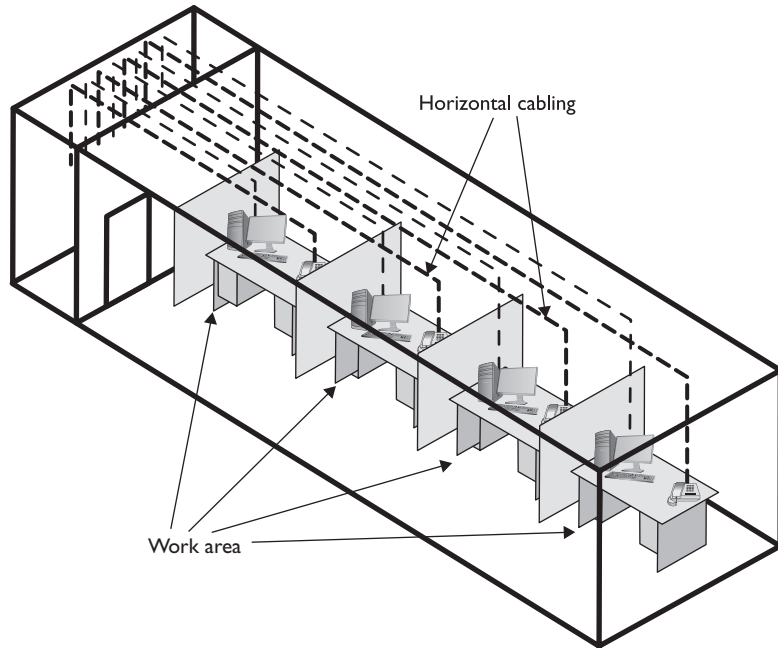
Figure 6-5 Horizontal cabling and work area
