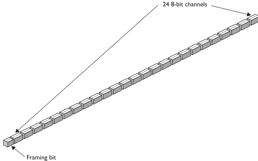
Figure 14-13 DS1 frame
