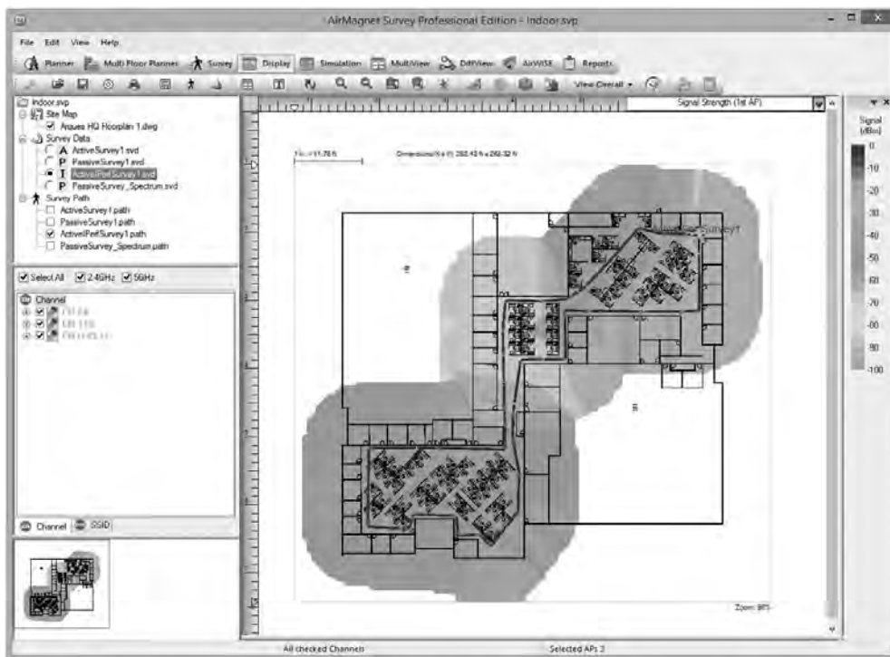
Figure 15-13 AirMagnet Survey Pro
