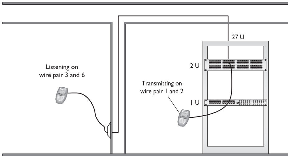
Figure 6-50 Far-end crosstalk
