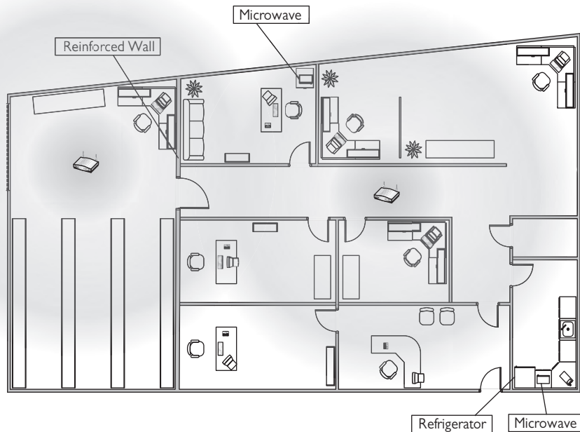
Figure 15-15 Site survey with heat map
