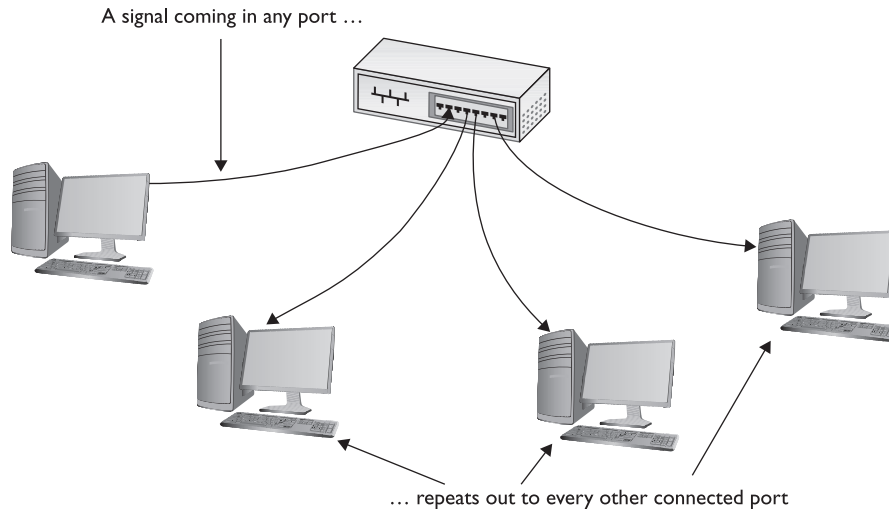
Figure 4-1 Ethernet hub
