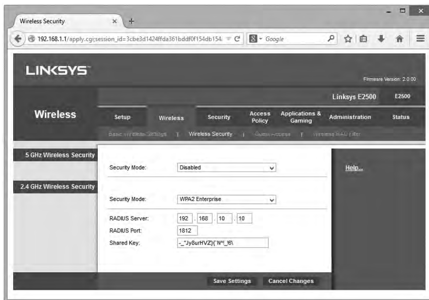
Figure 15-33 Encryption screen with RADIUS option
