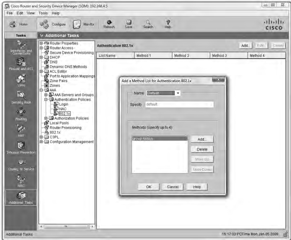
Figure 12-32 802.1X configuration on a Cisco 2811
