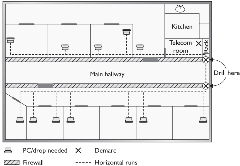
Figure 6-26 Network floor plan
