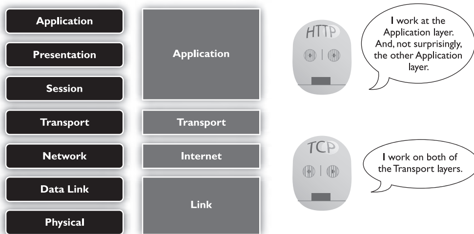
Figure 2-49 OSI model and TCP/IP model side by side
