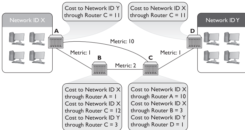
Figure 8-24 Updated routing tables
