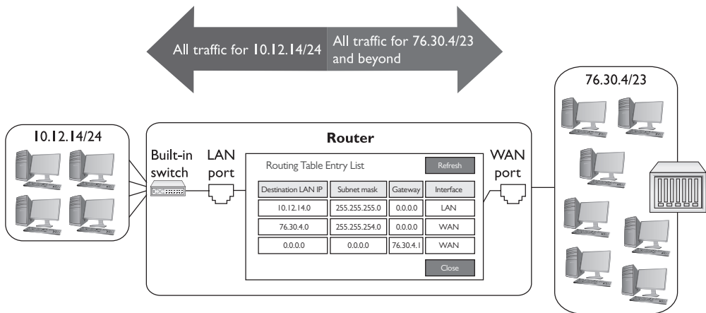
Figure 8-9 The network based on the routing table in Figure 8-7
