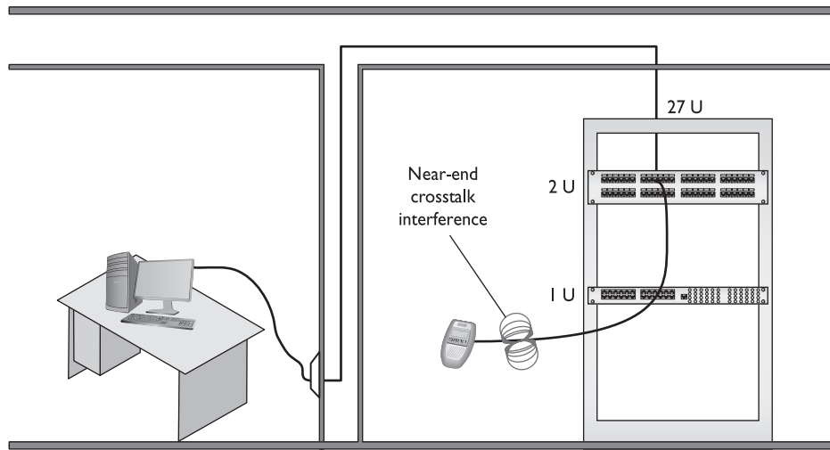
Figure 6-49 Near-end crosstalk
