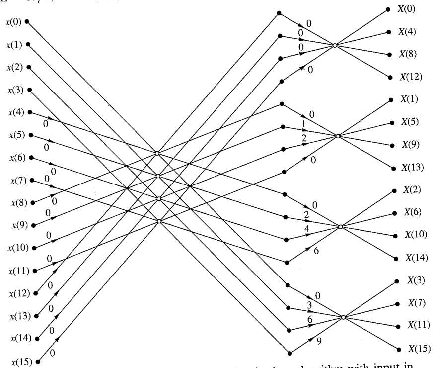
Figure 8.1.13 Sixteen-point radix-4 decimation-in-time algorithm with input in normal order and output in digit-reversed order. The integer multipliers shown on the graph represent the exponents on W_{16} .
