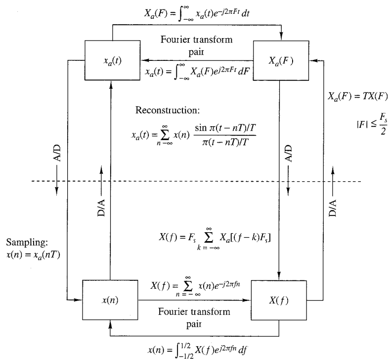
Figure 6.1.5 Time-domain and frequency-domain relationships for sampled signals.
