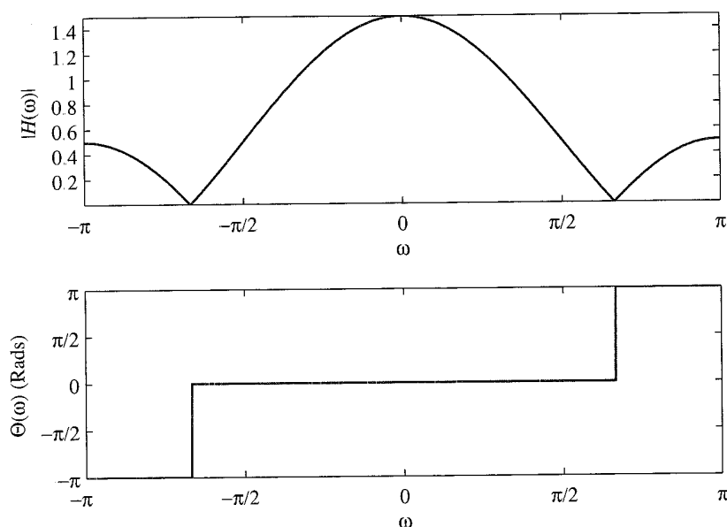
Figure 5.1.1 Magnitude and phase responses for the MA system in Example 5.1.2.
