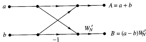
Figure 8.1.10 Basic butterfly computation in the decimation-in-frequency FFT algorithm.
