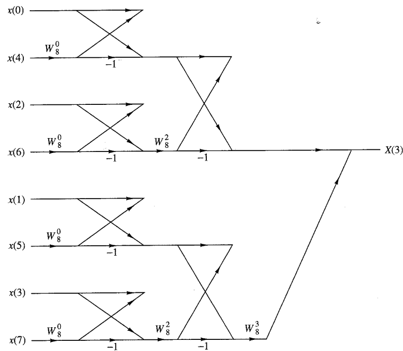
Figure 8.4.2 Butterflies that affect the computation of X(3) .
