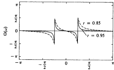
Figure 5.4.10 Frequency response characteristics of two notch filters with poles at (1) r = 0.85 and (2) r = 0.95 ; H(z) = b_0[(1 - 2 \cos \omega_0 z^{-1} + z^{-2}) / (1 - 2r \cos \omega_0 z^{-1} + r^2 z^{-2})] .
