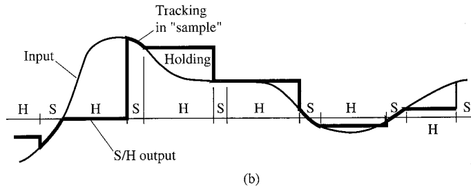
Figure 6.3.1 (a) Block diagram of basic elements of an A/D converter; (b) time-domain response of an ideal S/H circuit.
