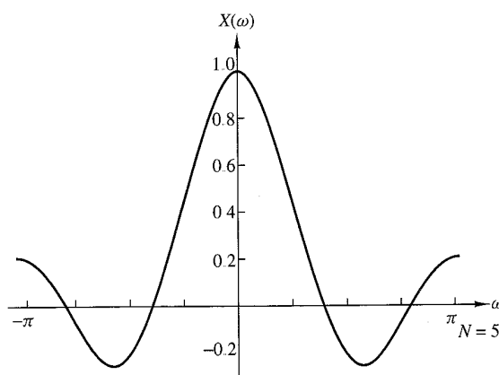
Figure 7.1.3 Plot of the function [\sin(\omega N/2)]/[N \sin(\omega/2)] .
