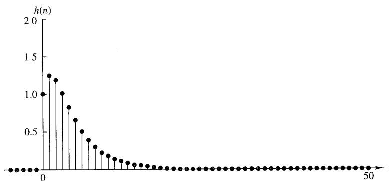
Figure 3.5.2 Plot of h(n) given by (3.5.16) with p_1 = 0.5 , p_2 = 0.75 ; h(n) = [1/(p_1 - p_2)](p_1^{n+1} - p_2^{n+1})u(n) .
