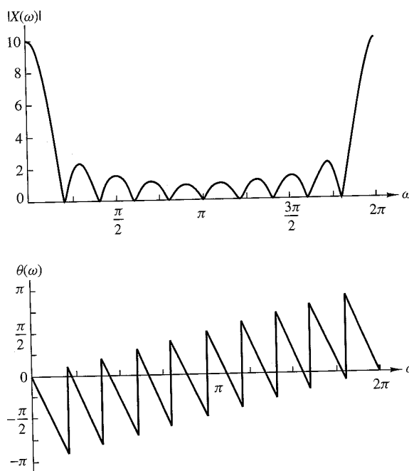
Figure 7.1.5 Magnitude and phase characteristics of the Fourier transform for signal in Example 7.1.2.
