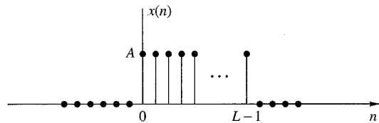
Figure 4.2.7 Discrete-time rectangular pulse
