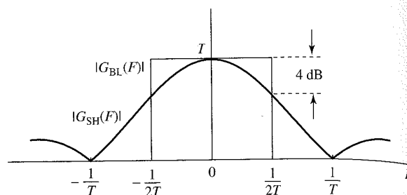
Figure 6.3.9 Frequency responses of sample-and-hold and the ideal bandlimited interpolator.
