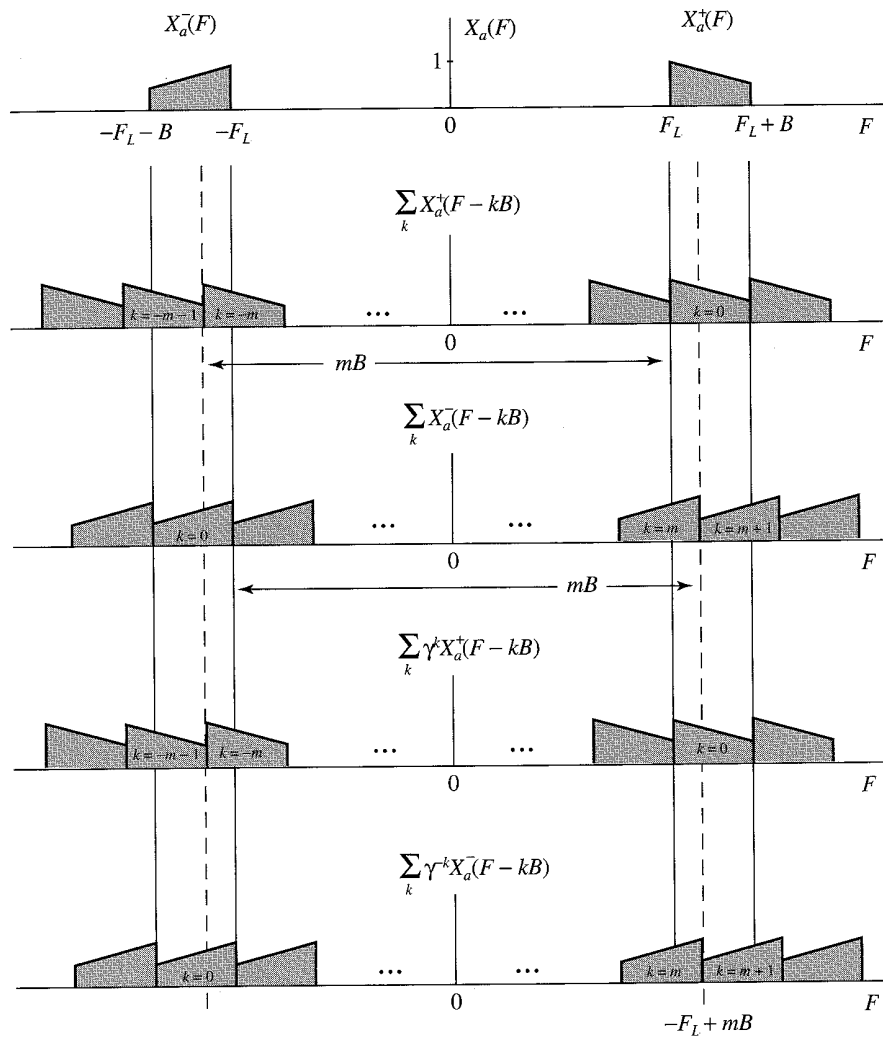
Figure 6.4.6 Illustration of aliasing in second-order bandpass sampling.
