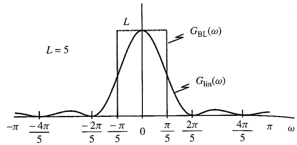
Figure 6.5.3 Frequency response of ideal and linear discrete-time interpolators.
