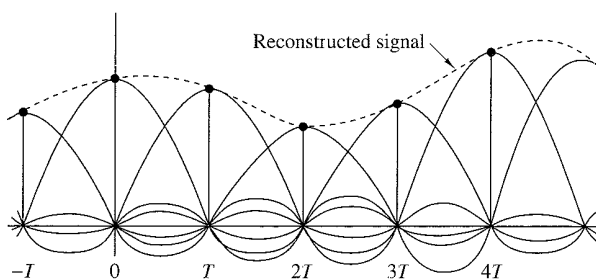
Figure 6.1.2 Reconstruction of a continuous-time signal using ideal interpolation.
