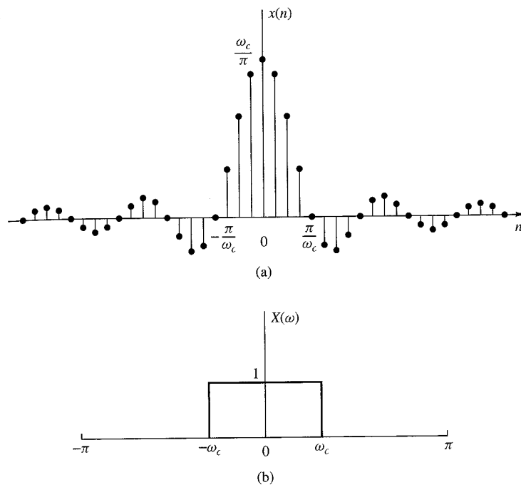
Figure 4.2.4 Fourier transform pair in (4.2.35) and (4.2.36).
