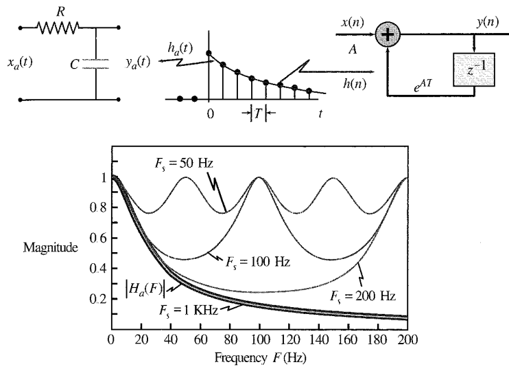
Figure 6.2.4 Discrete-time implementation of an analog integrator using impulse response sampling. The approximation is satisfactory when the bandwidth of the input signal is much less than the sampling frequency.
