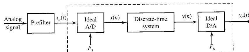
Figure 6.2.1 System for the discrete-time processing of continuous-time signals.
