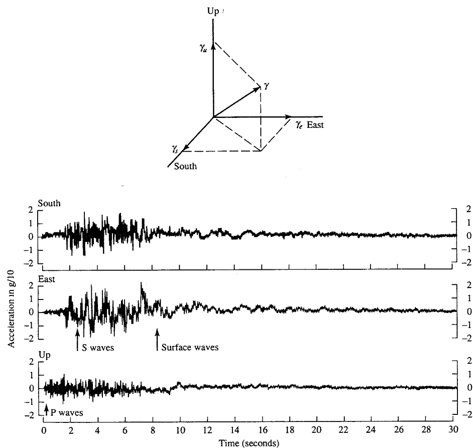
Figure 1.2.1 Three components of ground acceleration measured a few kilometers from the epicenter of an earthquake. (From Earthquakes , by B. A. Bold, ©1988 by W. H. Freeman and Company Reprinted with permission of the publisher.)
