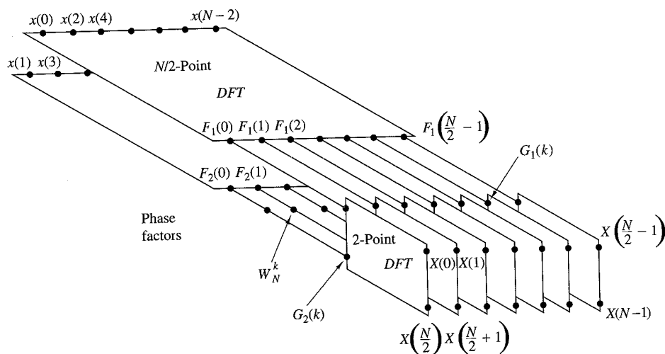
Figure 8.1.4 First step in the decimation-in-time algorithm.
