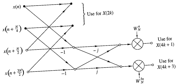
Figure 8.1.16 Butterfly for SRFFT algorithm.
