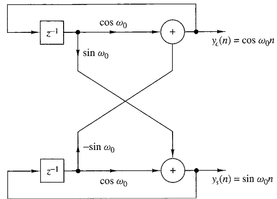
Figure 5.4.19 Realization of the coupled-form oscillator.
