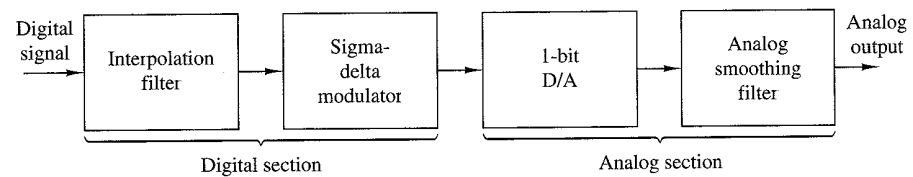
Figure 6.6.7 Elements of an oversampling D/A converter.
