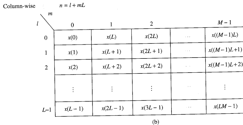
Figure 8.1.2 Two arrangements for the data arrays.
