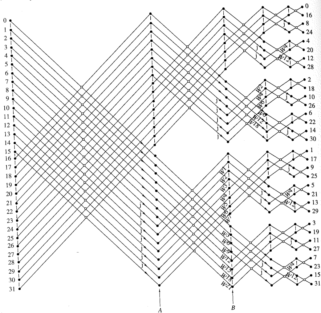
Figure 8.1.15 Length 32 split-radix FFT algorithms from paper by Duhamel (1986); reprinted with permission from the IEEE.
