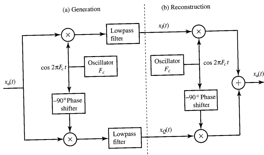
Figure 6.4.8 (a) Scheme for generating the in-phase and quadrature components of a bandpass signal. (b) Scheme for reconstructing a bandpass signal from its in-phase and quadrature components.
