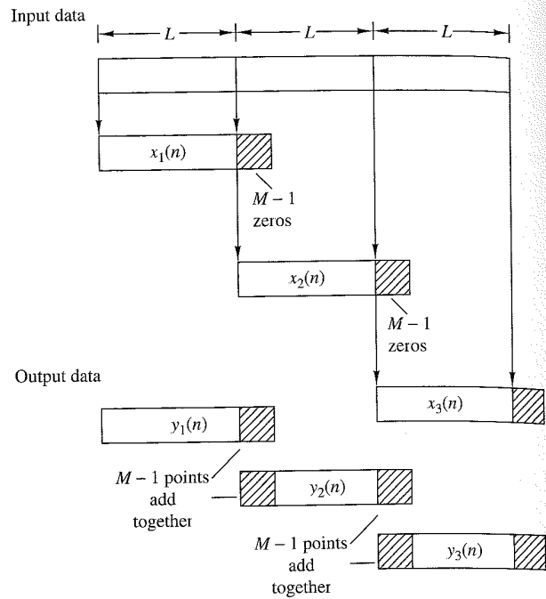
Figure 7.3.2 Linear FIR filtering by the overlap-add method.
