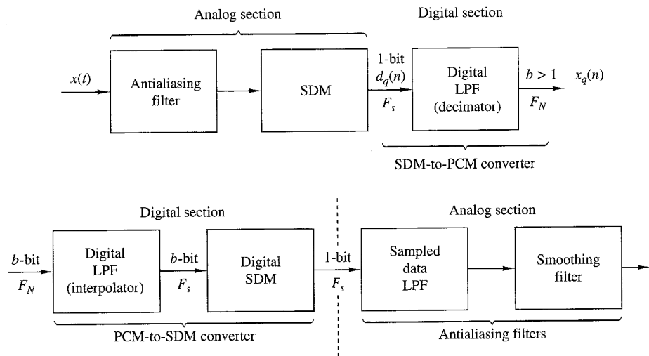
Figure 6.6.6 Basic elements of an oversampling A/D converter.
