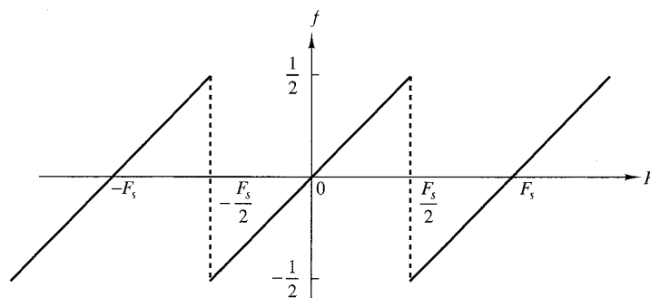
Figure 6.1.4 Relationship between frequency variables F and f .
