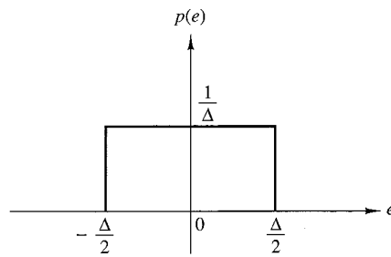
Figure 6.3.5 Probability density function for the quantization error.
